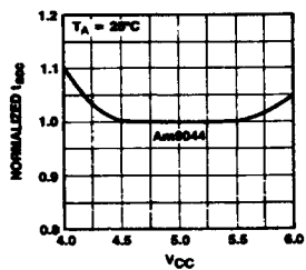
Normalized Access Time Versus Supply Voltage
