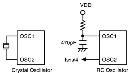
System oscillator
