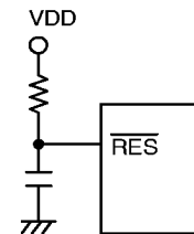
Reset circuit
