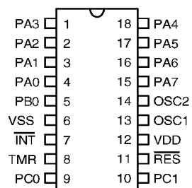
HT48R31 - 18 DIP-A-0
