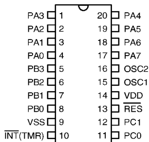
HT48R31 - 20 DIP-F-0
