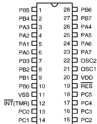
HT48R31 - 28 SKDIP-B-0
