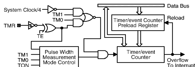
Timer/event counter
