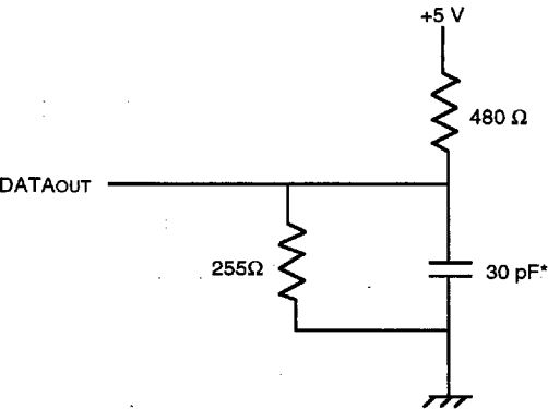
*Includes scope and jig. Figure 1. Output Load
