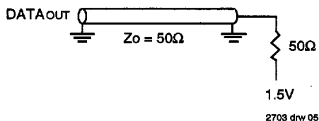
Figure 3. Alternate Output Load
