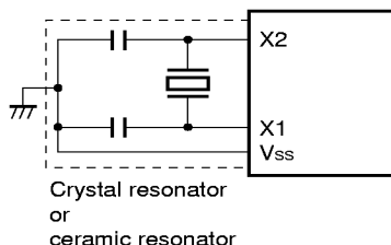
Figure 8-4. Example of Using Subsystem Clock Oscillation Circuit
