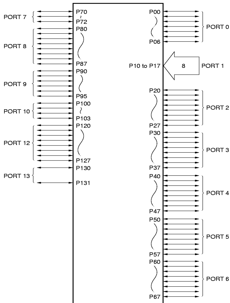
Figure 8-1. Port Configuration
