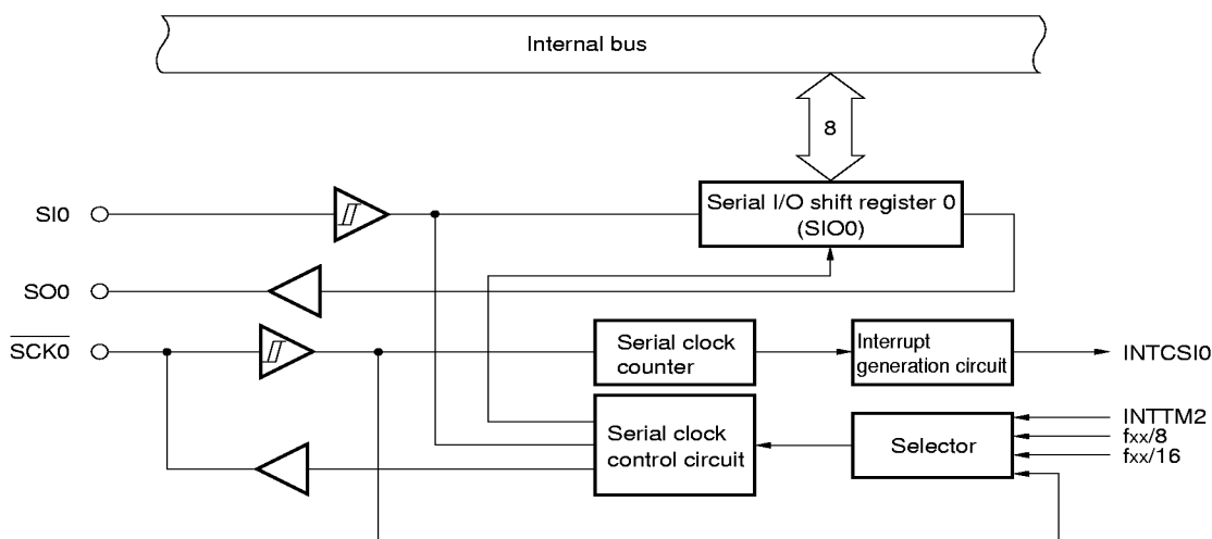
Figure 8-12. Block Diagram in 3-wire Serial I/O Mode
