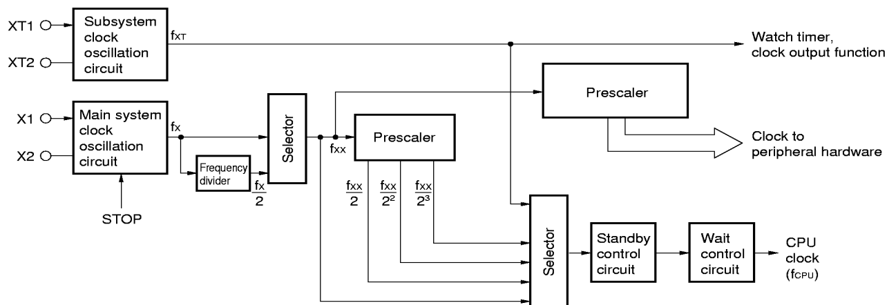
Figure 8-2. Block Diagram of Clock Generation Circuit
