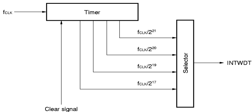
Figure 8-16. Block Diagram of Watchdog Timer
