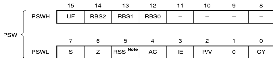
Figure 7-5. Program Status Word (PSW) Format
