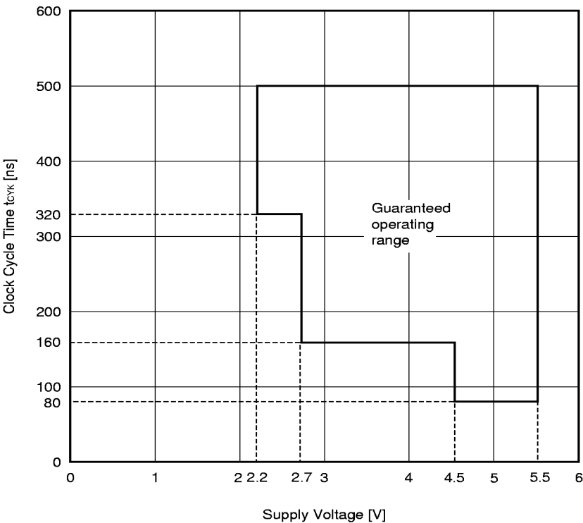
Figure 15-1. Power Supply Voltage and Clock Cycle Time
