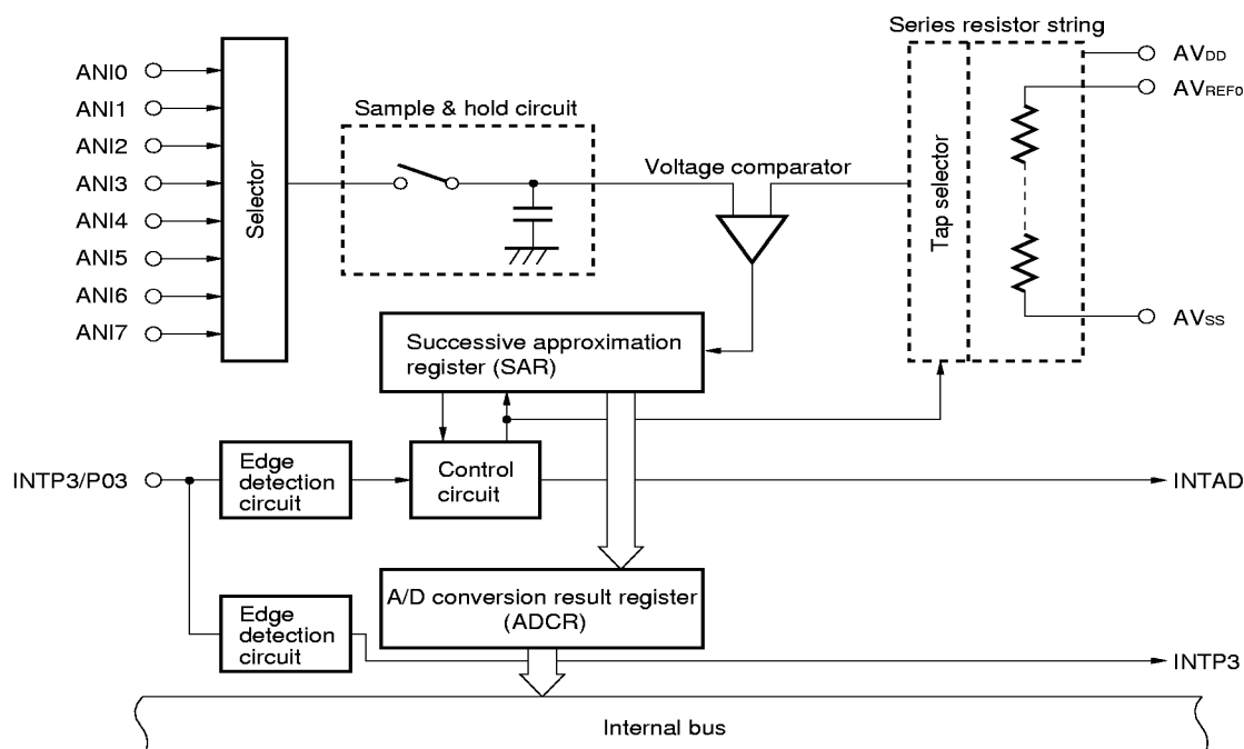
Figure 8-7. Block Diagram of A/D Converter
