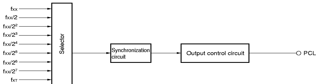
Figure 8-13. Block Diagram of Clock Output Function
