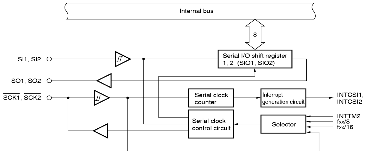
Figure 8-11. Block Diagram in 3-wire Serial I/O Mode
