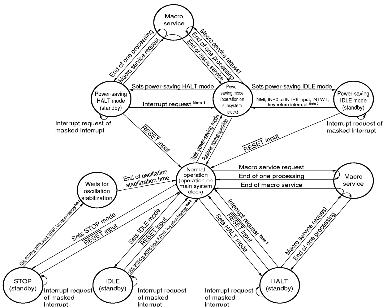
Figure 11-1. Transition of Standby Status
