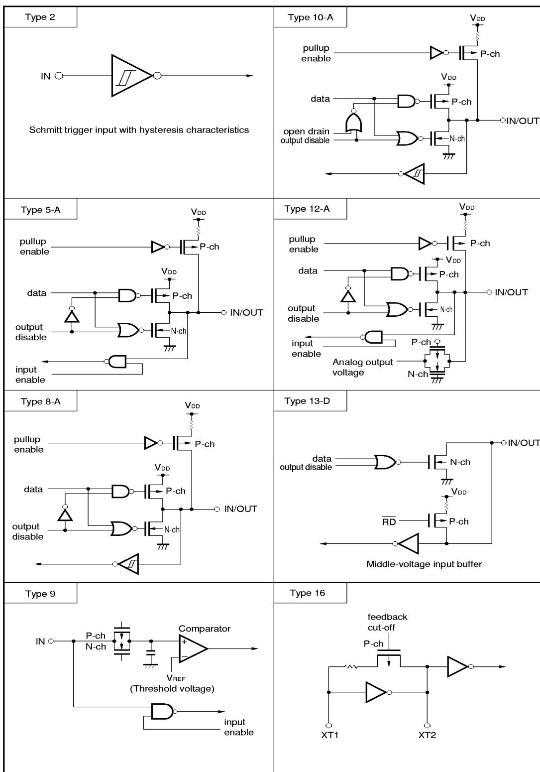
Figure 6-1. Pin I/O Circuits
