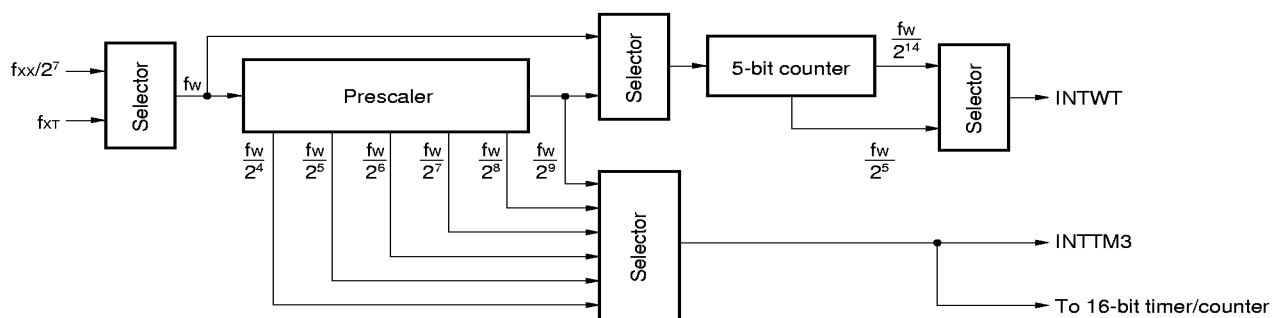
Figure 8-15. Block Diagram of Watch Timer
