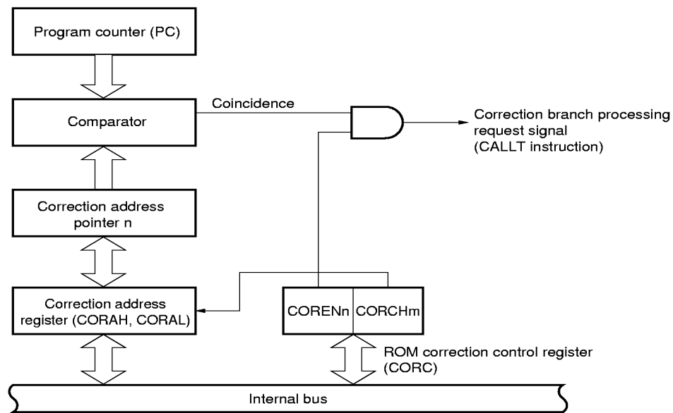
Figure 13-1. Block Diagram of ROM Correction
