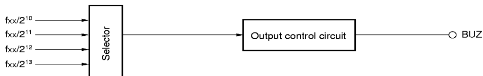
Figure 8-14. Block Diagram of Buzzer Output Function
