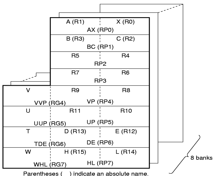
Figure 7-3. General-Purpose Register Format
