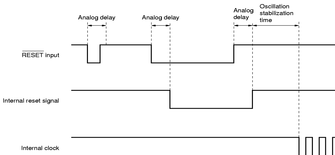
Figure 12-2. Accepting Reset Signal
