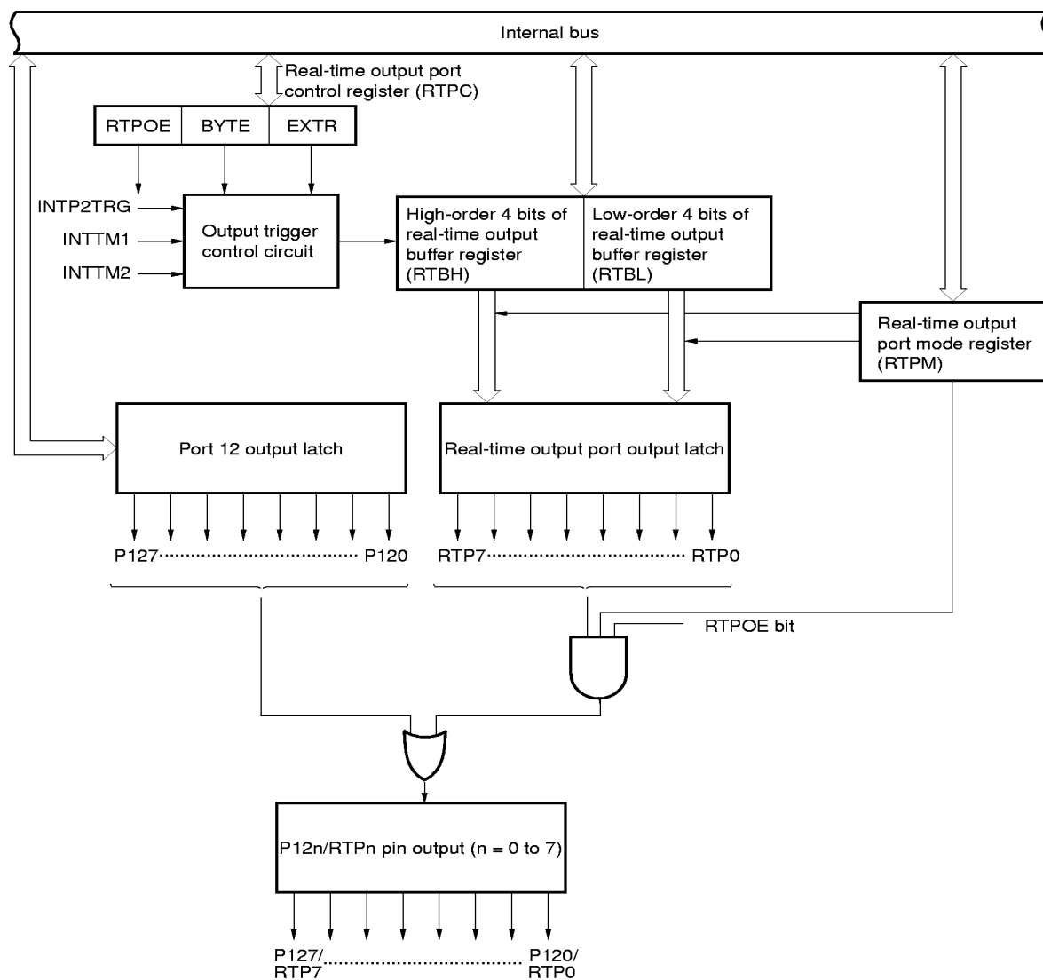
Figure 8-5. Block Diagram of Real-Time Output Port
