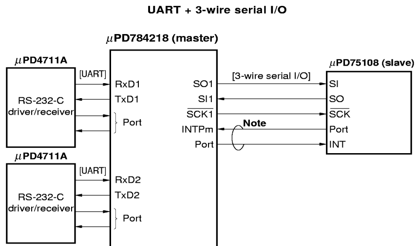
Figure 8-9. Example of Serial Interface
