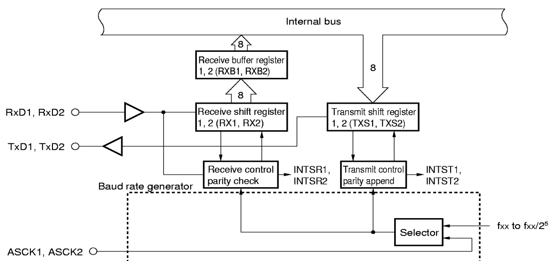
Figure 8-10. Block Diagram in Asynchronous Serial Interface Mode
