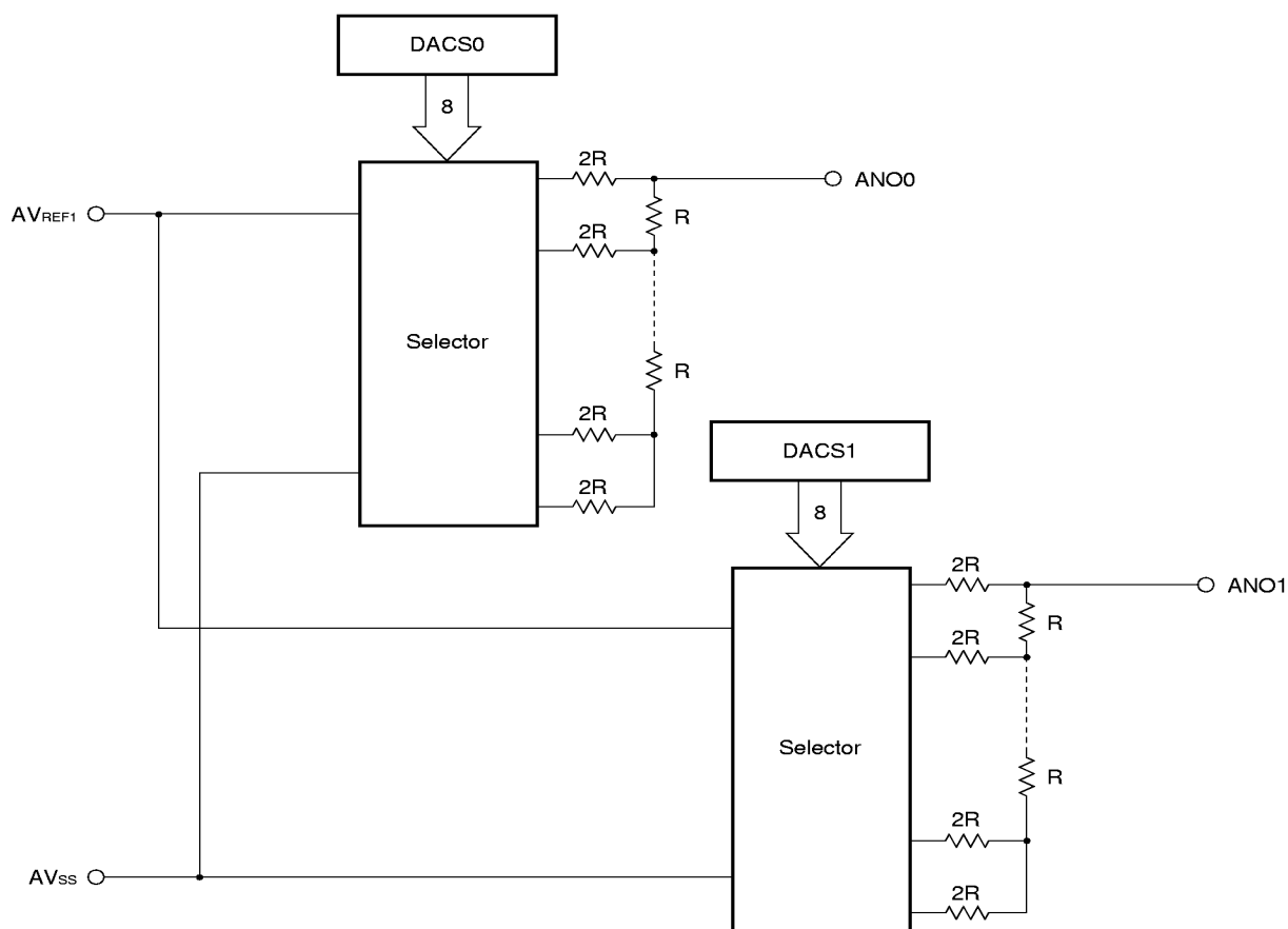
Figure 8-8. Block Diagram of D/A Converter
