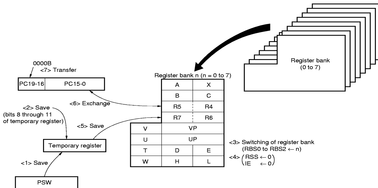
Figure 9-1. Context Switching Operation When Interrupt Request Is Generated
