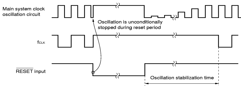
Figure 12-1. Oscillation of Main System Clock during Reset Period
