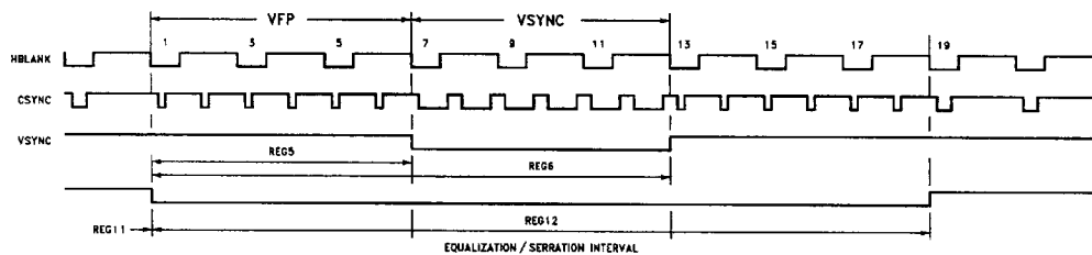
FIGURE 3. Equalization/Serration Interval Programming
