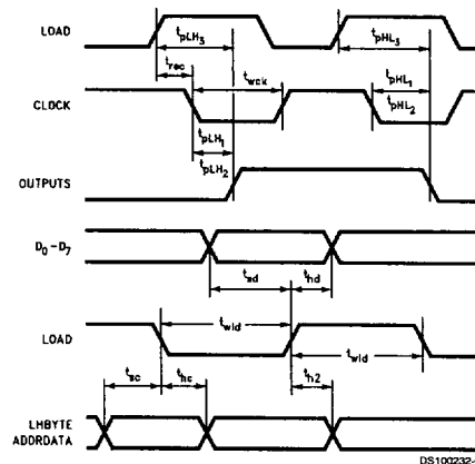
FIGURE 5. AC Specifications
