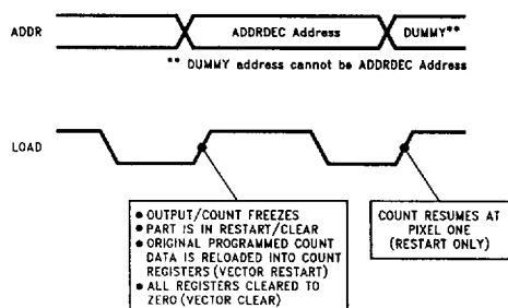
FIGURE 4. ADDRDEC Timing
