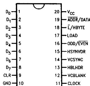
Pin Assignment for DIP and SOIC
