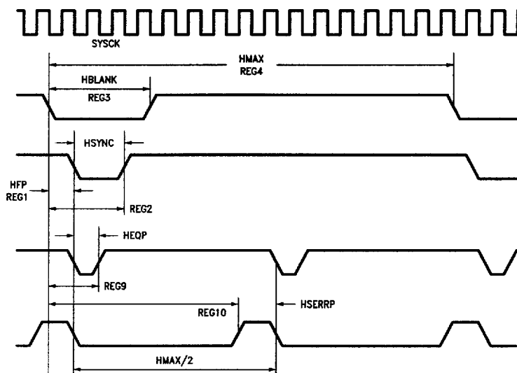
FIGURE 1. Horizontal Waveform Specification
