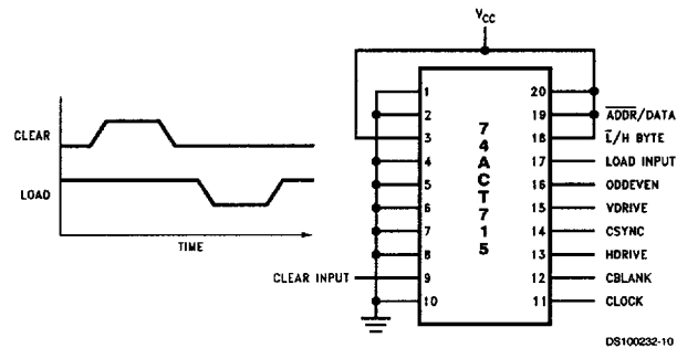
FIGURE 6. Default RS170 Hardwire Configuration
