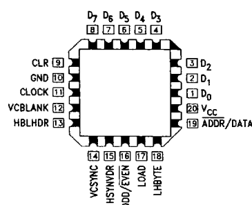
Pin Assignment for LCC
