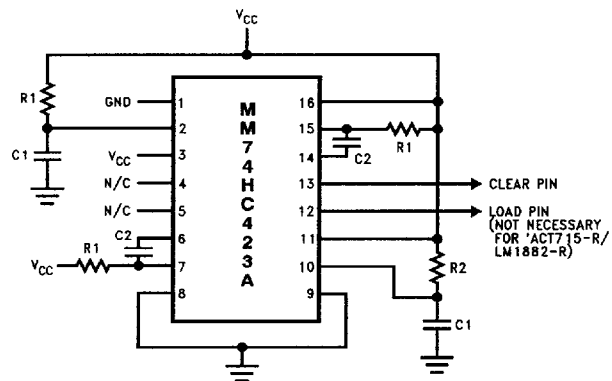
FIGURE 6. Default RS170 Hardwire Configuration
