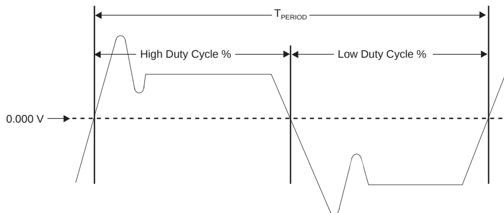
Figure 1 - Differential (CPUCLK - CPUCLK#) Measurement Points (Tperiod, Duty Cycle, Jitter)
