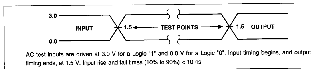
Fig. 10 Transient Input/Output Reference Waveform for V_{CC} = 3.3 \pm 0.3\text{ V}
