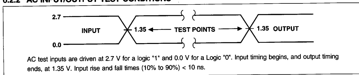
Fig. 9 Transient Input/Output Reference Waveform for V_{CC} = 2.7 to 3.6\text{ V}
