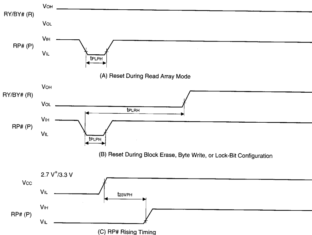
Fig. 15 AC Waveform for Reset Operation
