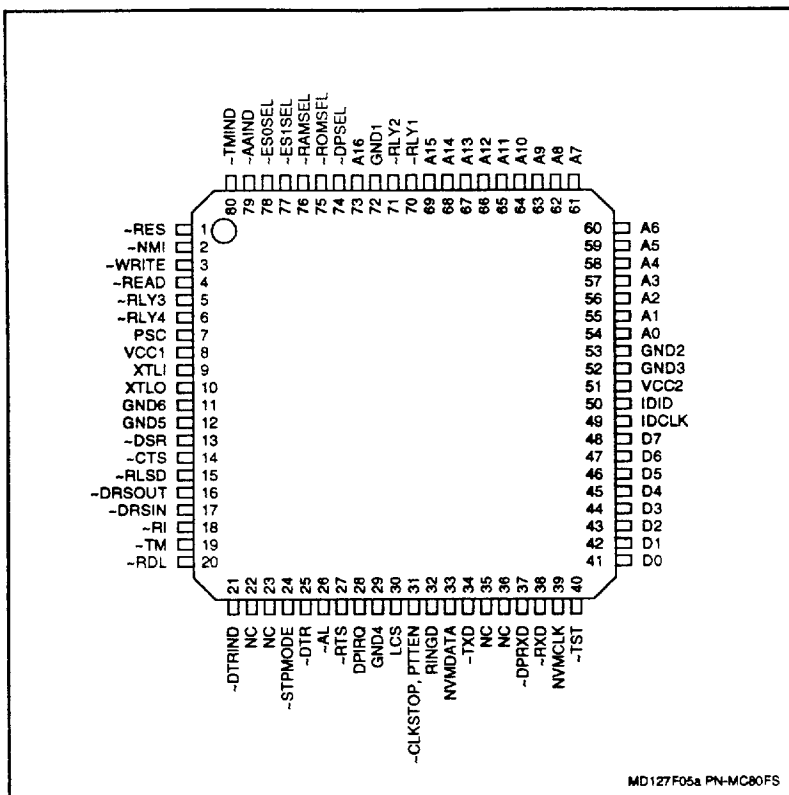
Figure 5a. MCU Pin Signals- 80-Pin PQFP - Serial Interface
