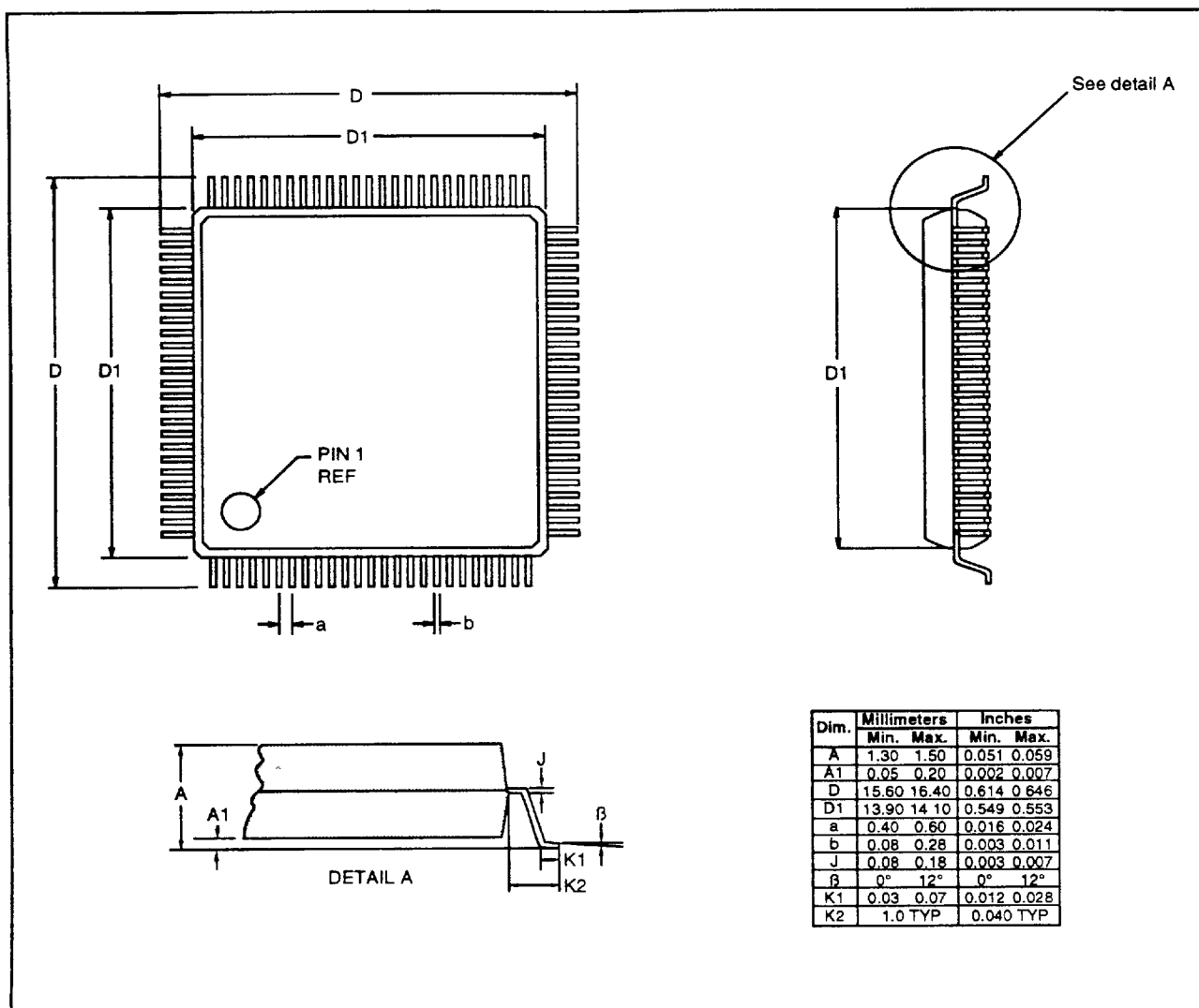
Figure 18f. Package Dimensions - 100-Pin TQFP
