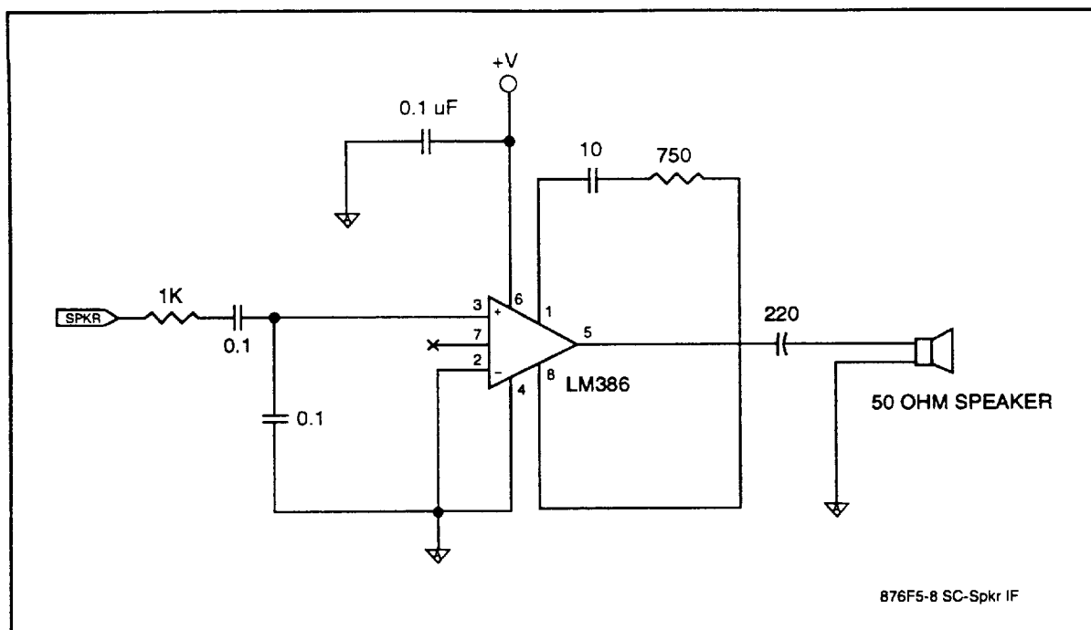
Figure 17. Typical External Speaker Circuit
