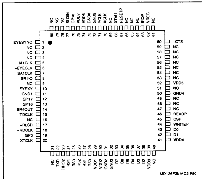
Figure 8b. MDP Pin Signals - 80-Pin PQFP (MDP2)
