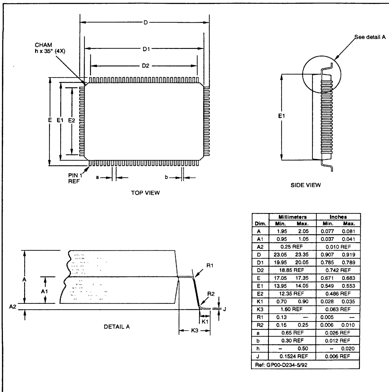
Figure 18c. Package Dimensions - 100-Pin PQFP
