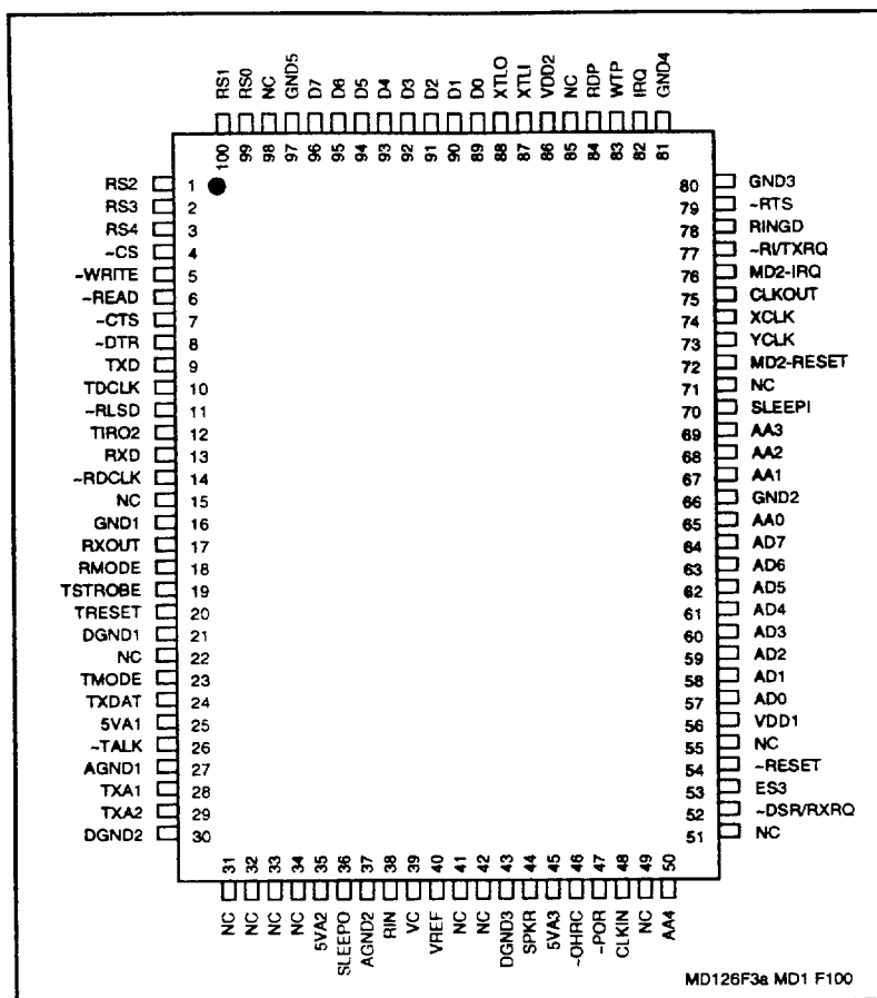
Figure 8a. MDP Pin Signals - 100-Pin PQFP (MDP1)
