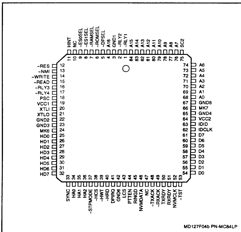
Figure 4b. MCU Pin Signals - 84-Pin PLCC - Parallel Interface
