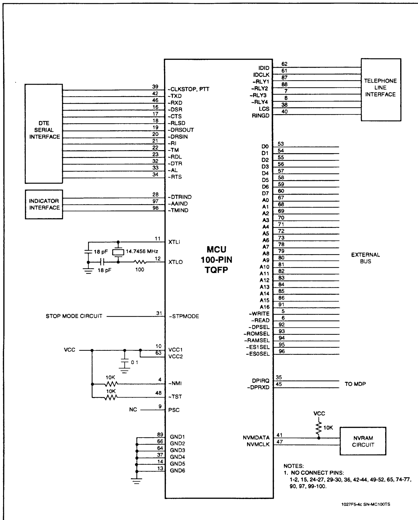
Figure 12c. Interface Schematic - MCU with Serial DTE Interface - 100-Pin TQFP
