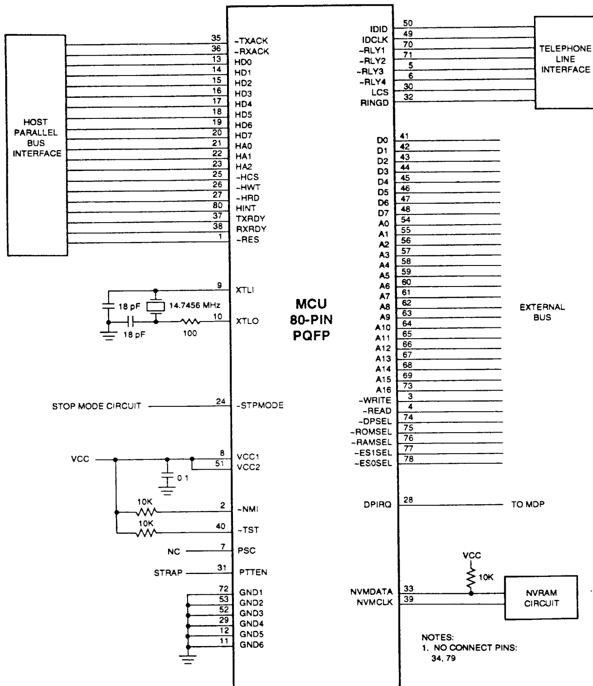
Figure 11b. Interface Schematic - MCU with Parallel Host Interface - 80-Pin PQFP
