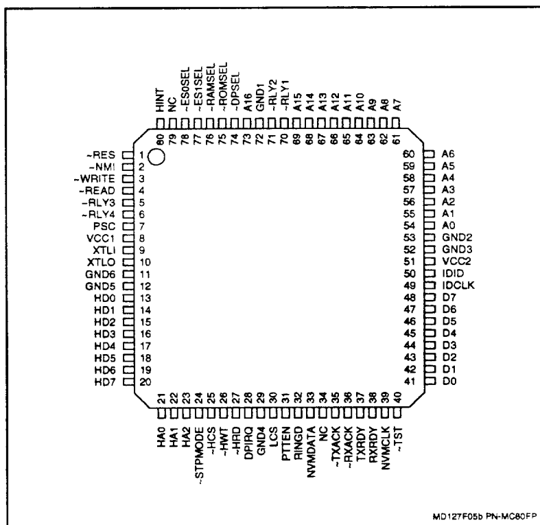
Figure 5b. MCU Pin Signals- 80-Pin PQFP - Parallel Interface
