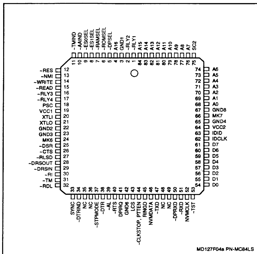
Figure 4a. MCU Pin Signals - 84-Pin PLCC - Serial Interface
