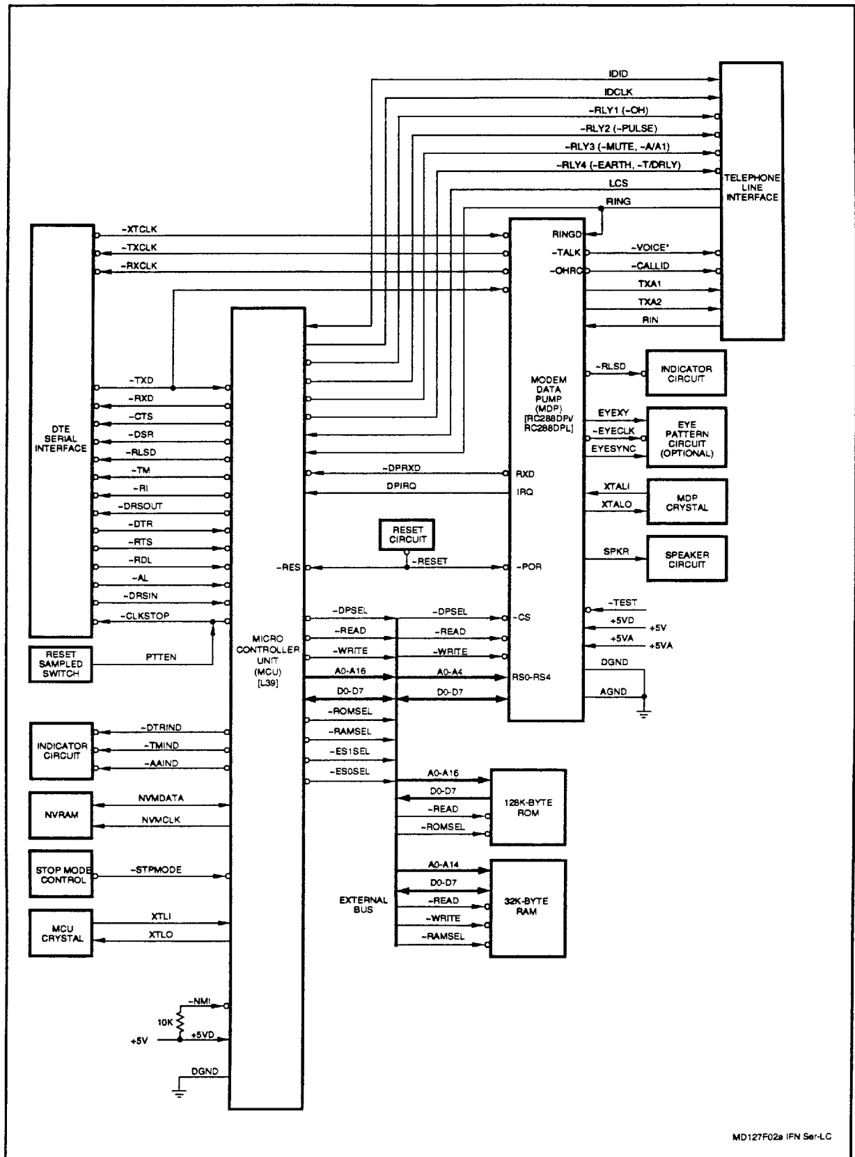
Figure 2a. Hardware Interface Signals - Serial Interface - Low Cost
