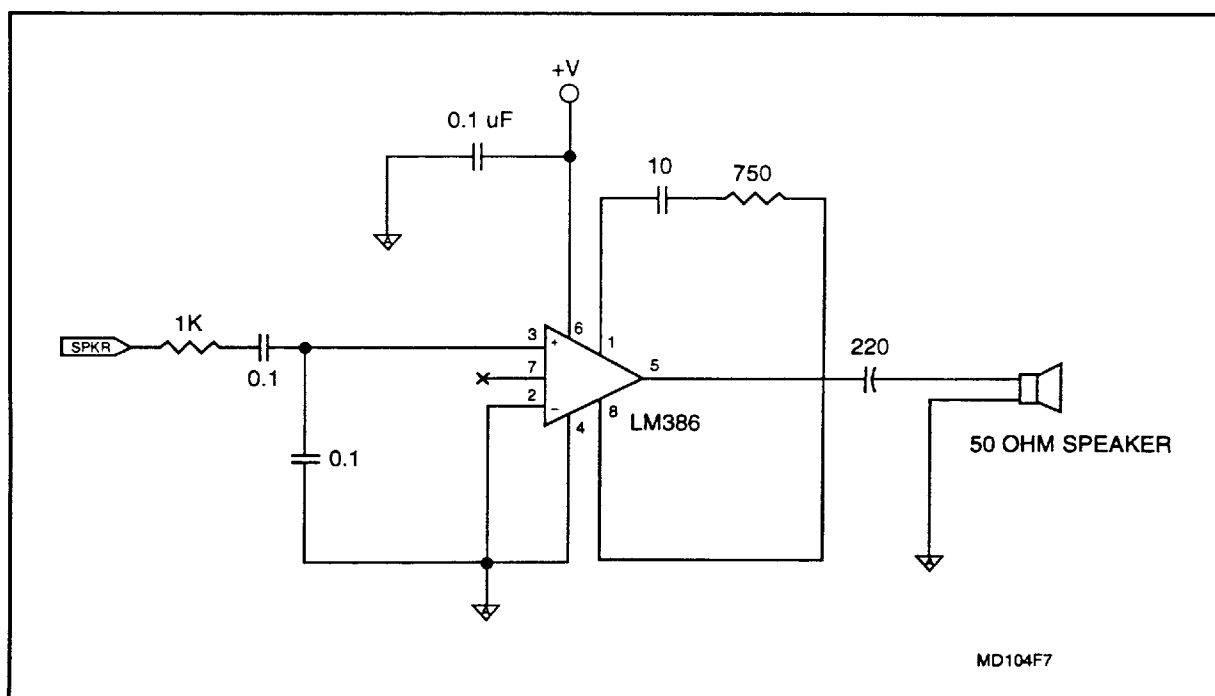
Figure 16. Typical Interface to External Hybrid
