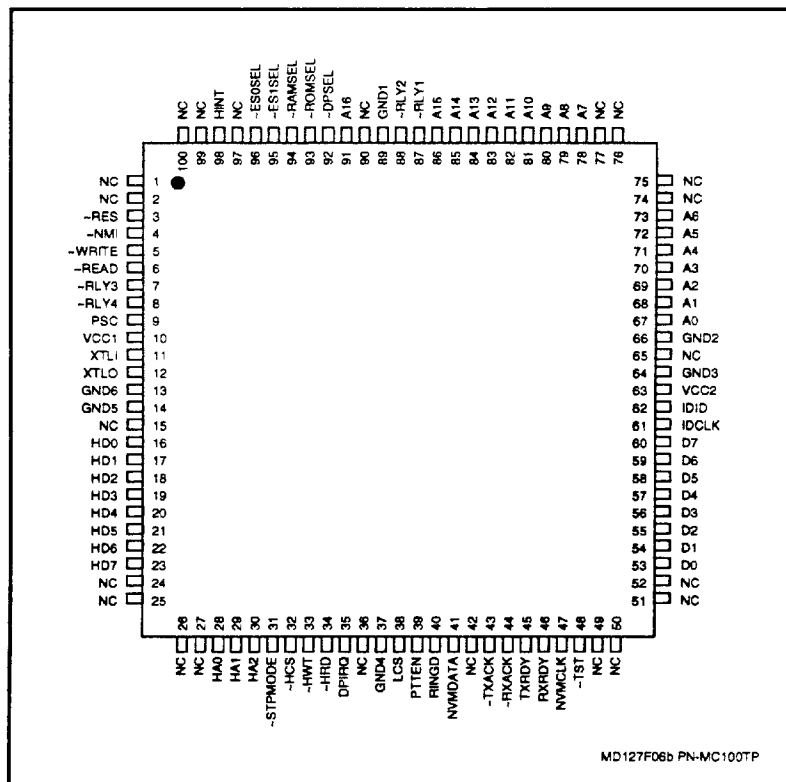
Figure 6b. MCU Pin Signals- 100-Pin TQFP - Parallel Interface
