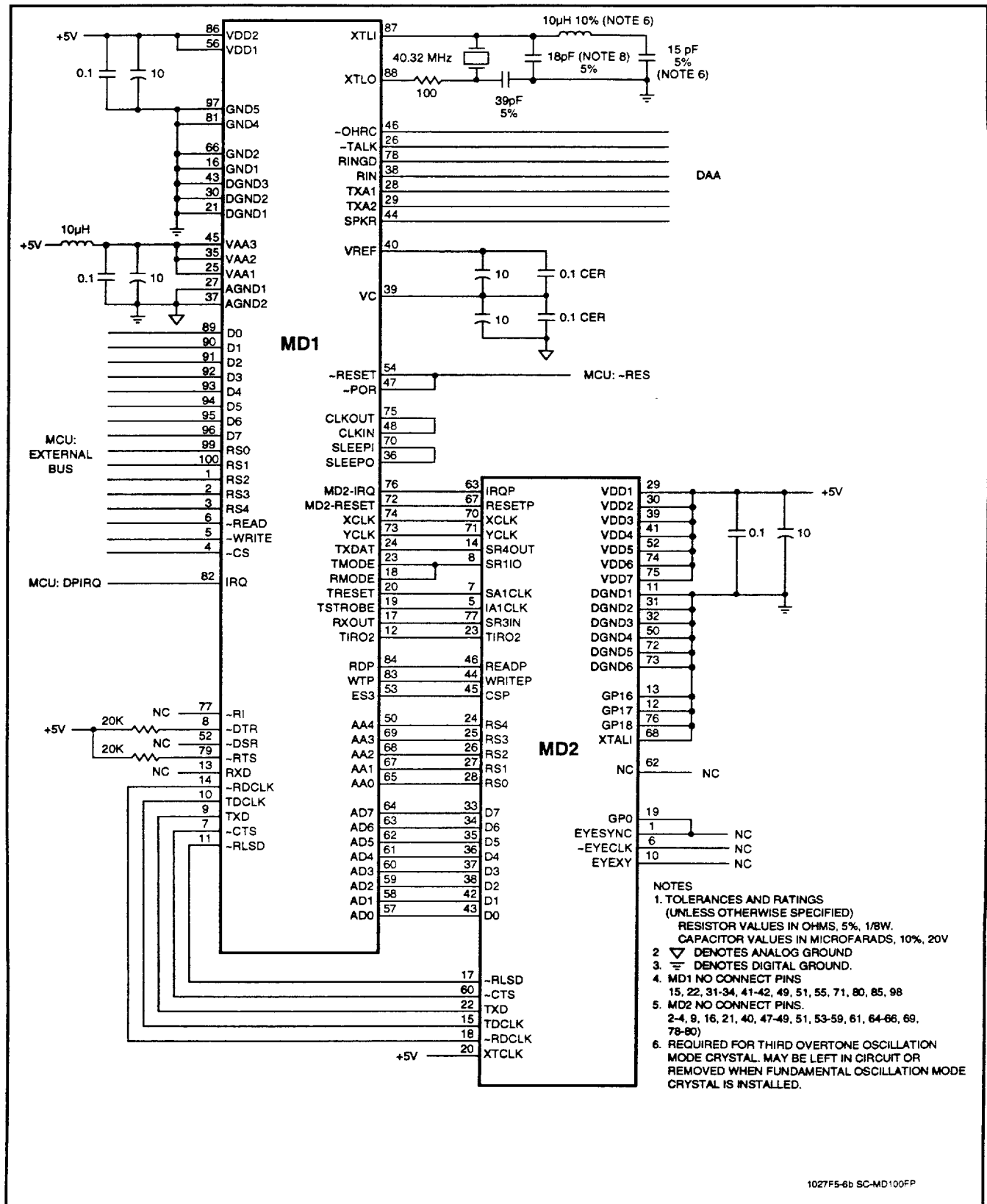
Figure 14b. Interface Schematic - MDP with Parallel Host Interface - 100-Pin PQFP and 80-Pin PQFP
