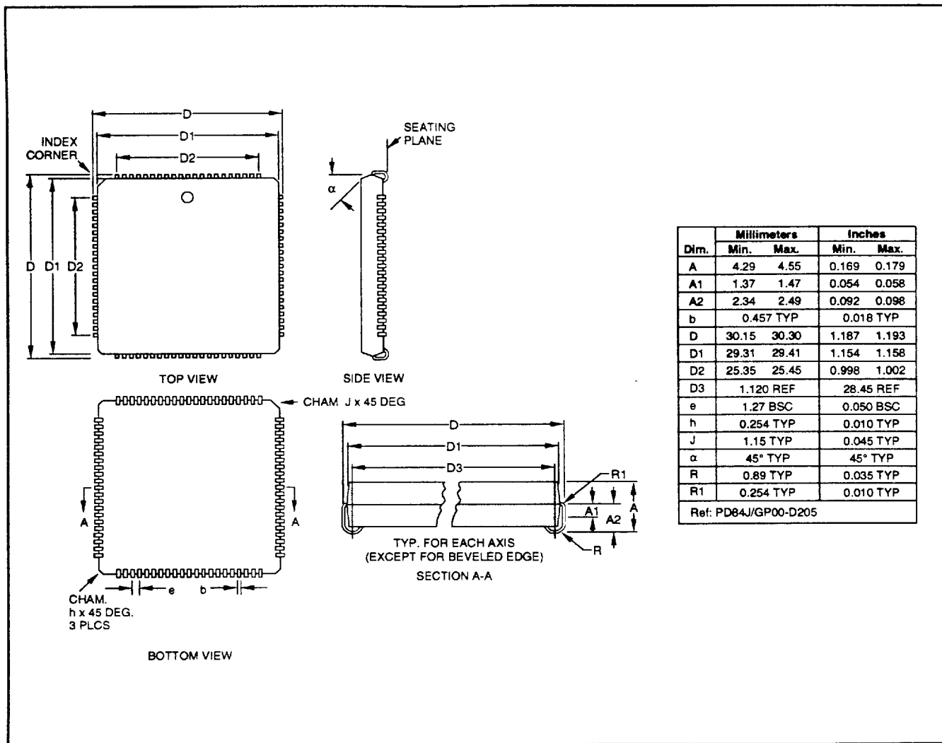
Figure 18b. Package Dimensions - 84-Pin PLCC
