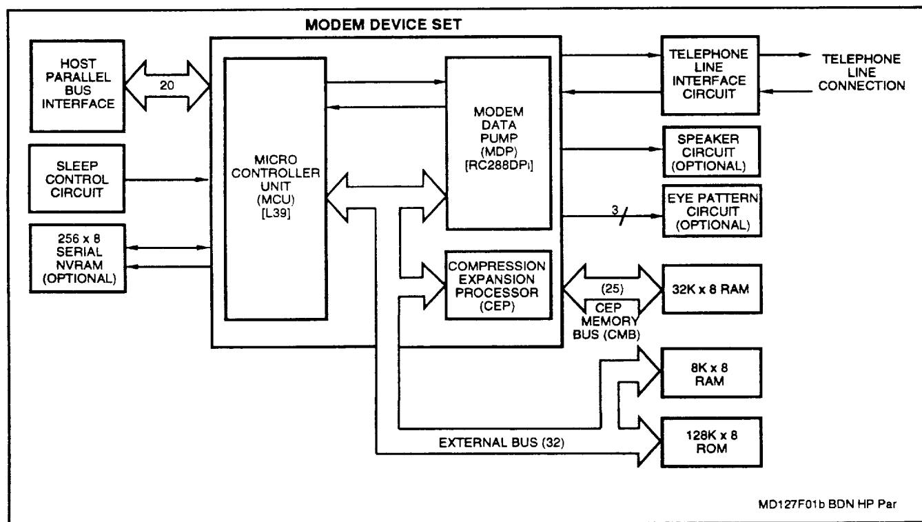
Figure 1b. Modem General Interface - RC288ACi High Performance Configuration
