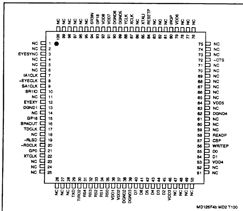
Figure 9b. MDP Pin Signals - 100-Pin TQFP (MDP2)
