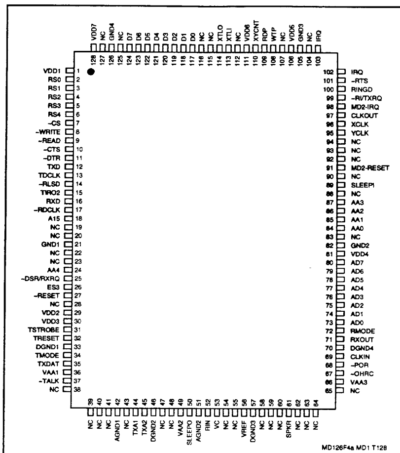
Figure 9a. MDP Pin Signals - 128-Pin TQFP (MDP1)
