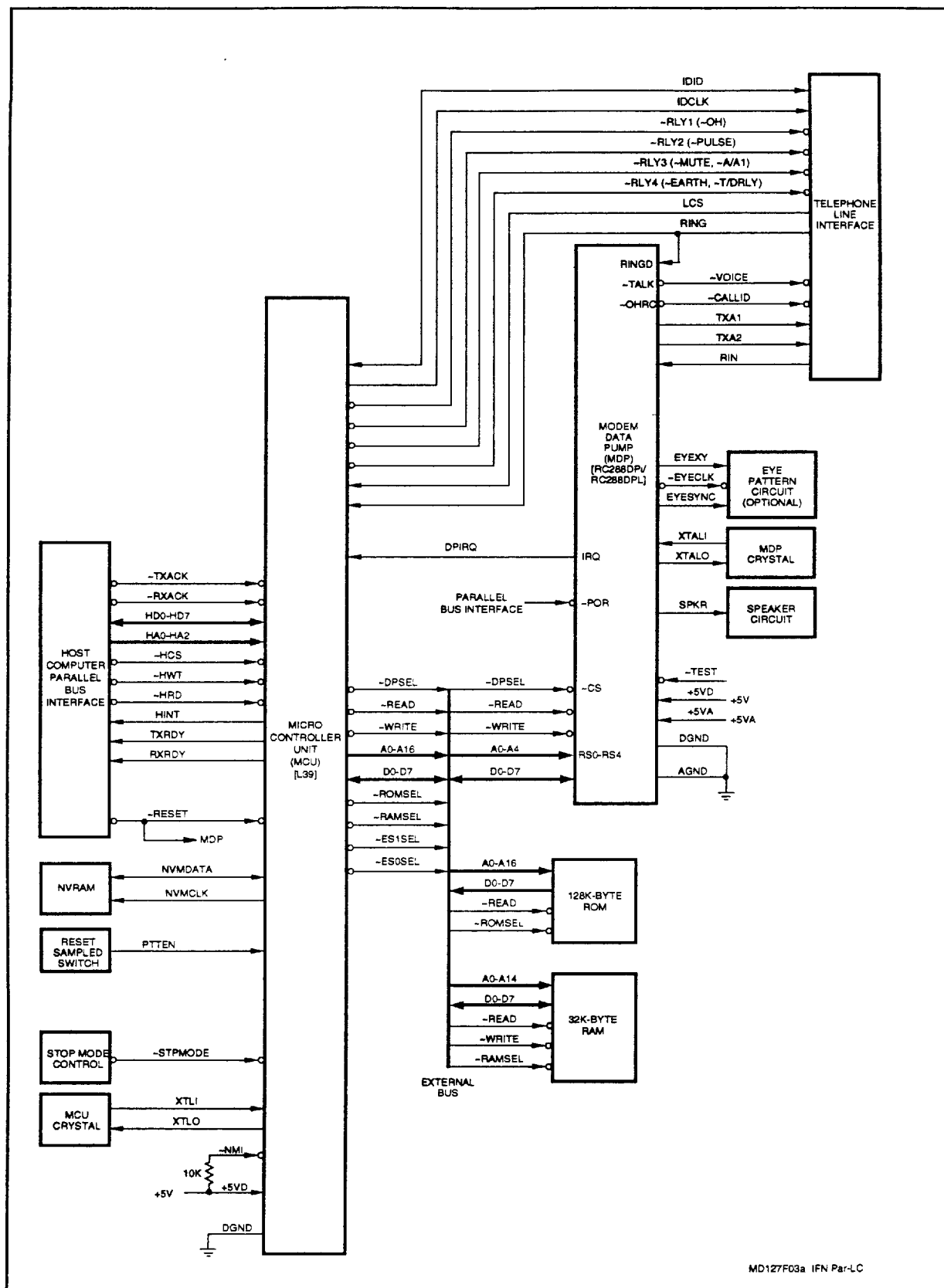
Figure 3a. Hardware Interface Signals - Parallel Interface - Low Cost
