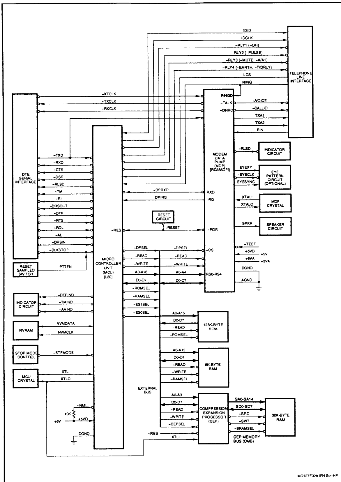
Figure 2b. Hardware Interface Signals - Serial Interface - High Performance
