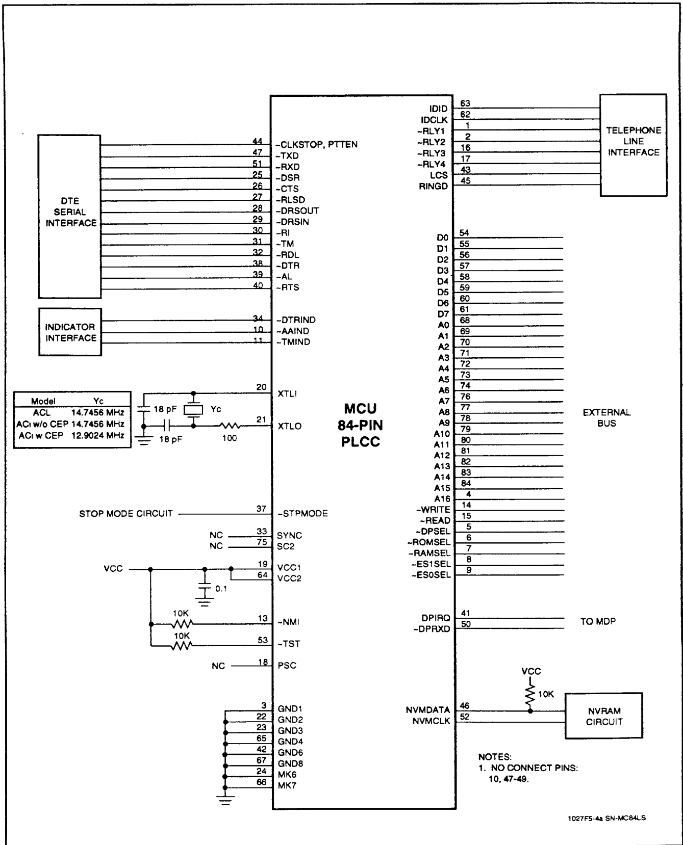
Figure 12a. Interface Schematic - MCU with Serial DTE Interface - 84-Pin PLCC
