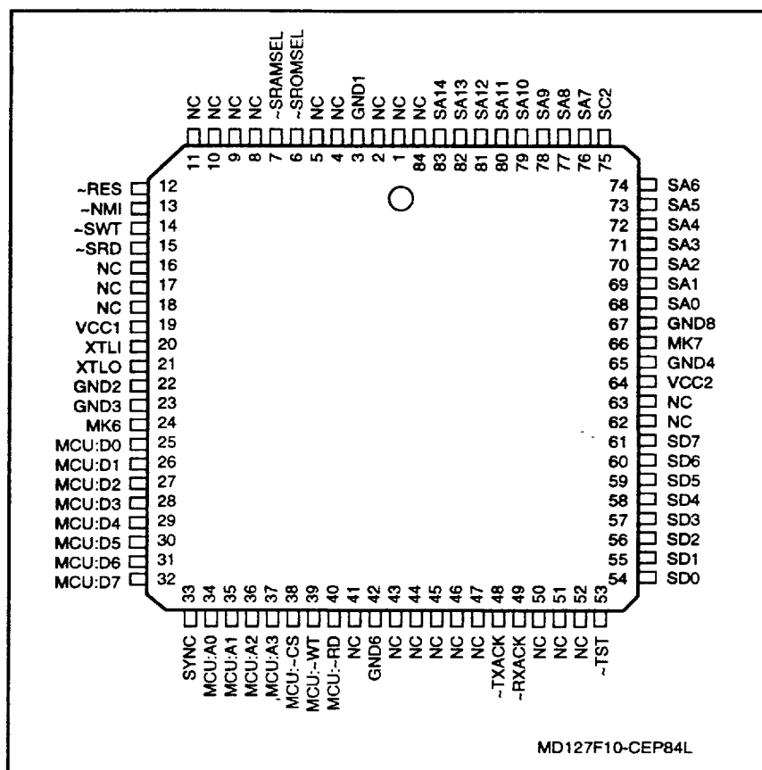
Figure 10. CEP Pin Signals - 84-Pin PLCC
