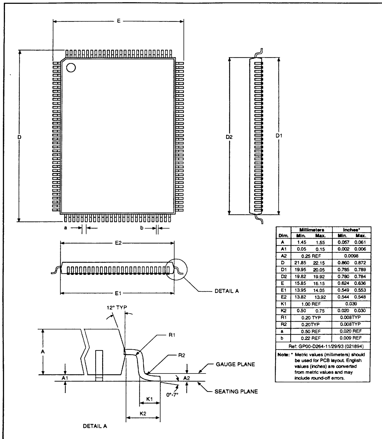
Figure 18e. Package Dimensions - 128-Pin TQFP
