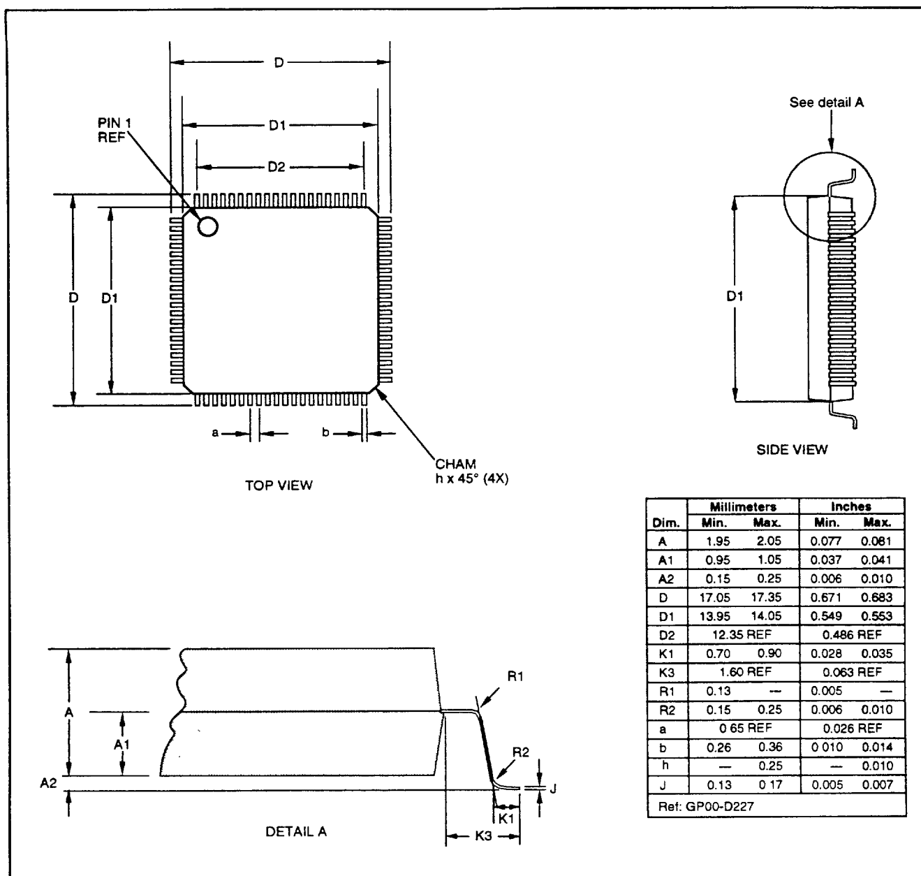
Figure 18d. Package Dimensions - 80-Pin PQFP
