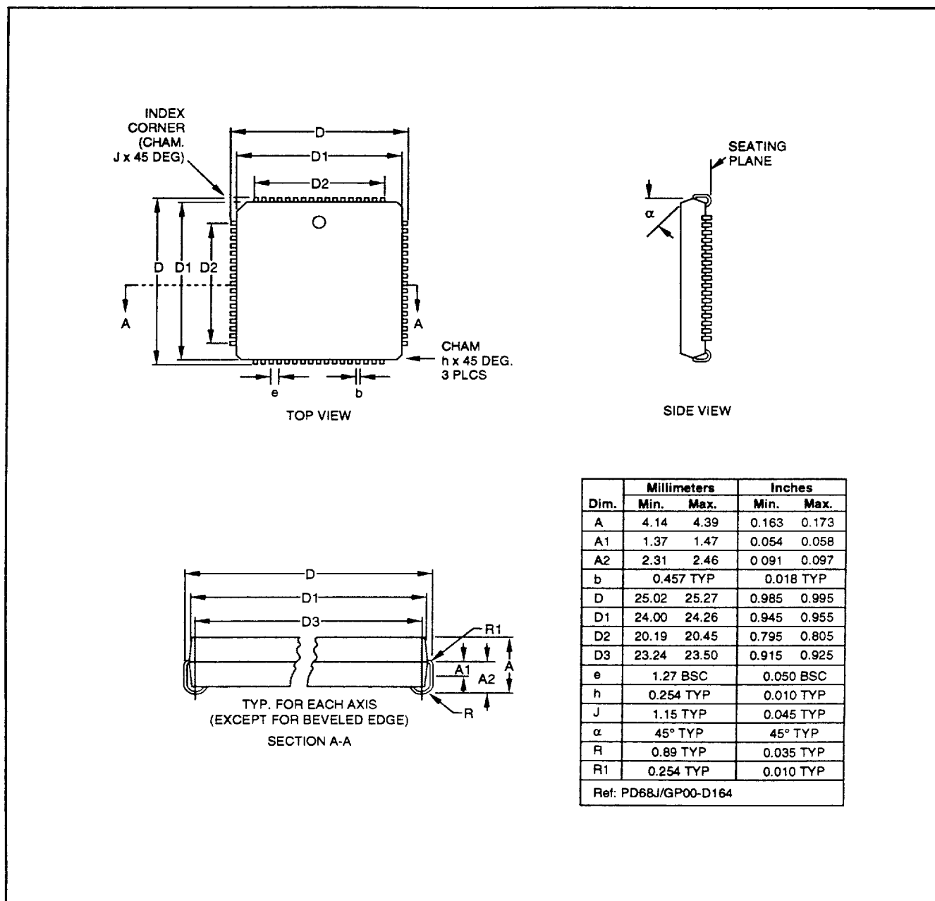
Figure 18a. Package Dimensions - 68-Pin PLCC
