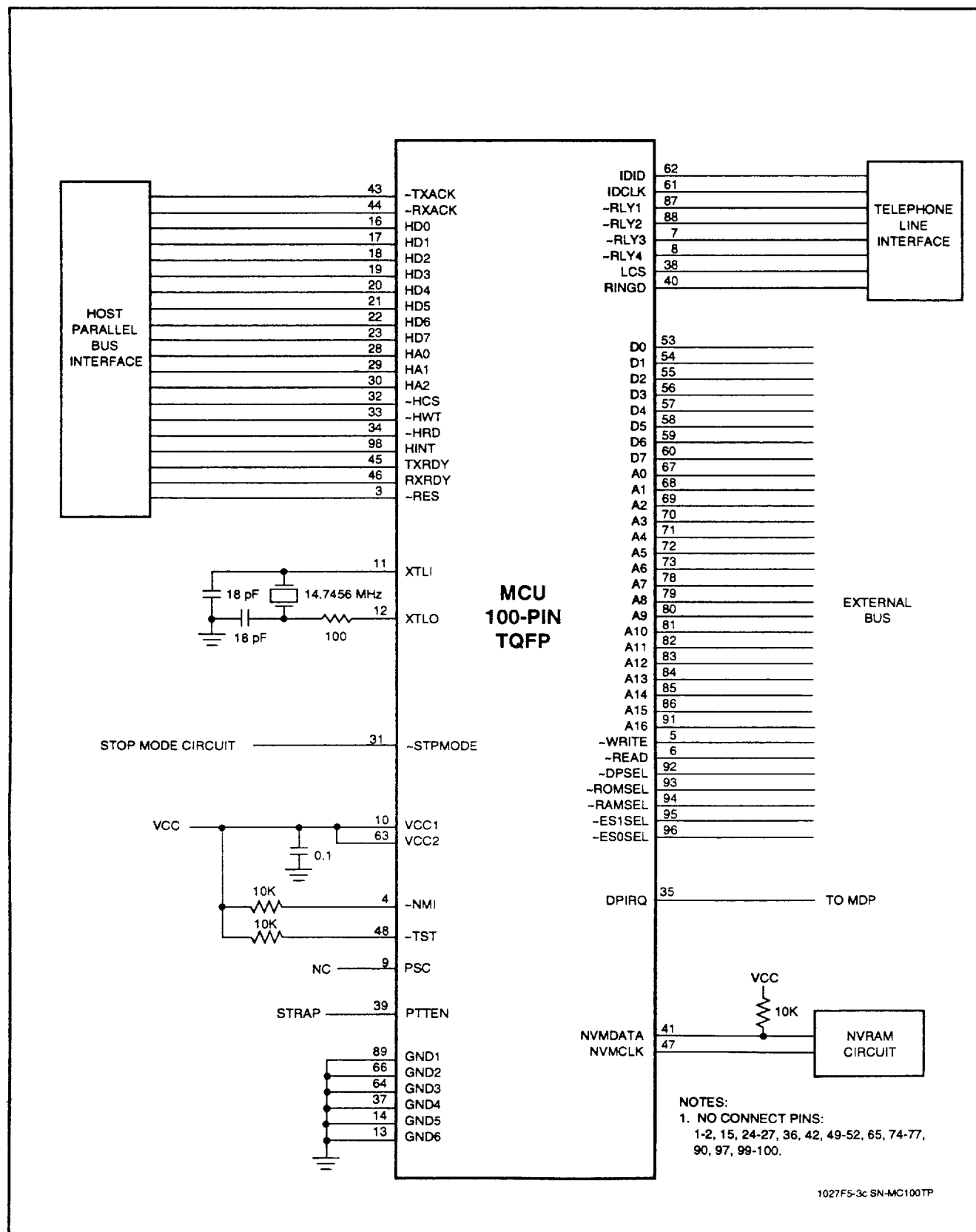
Figure 11c. Interface Schematic - MCU with Parallel Host Interface - 100-Pin TQFP
