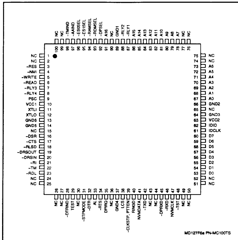
Figure 6a. MCU Pin Signals- 100-Pin TQFP - Serial Interface
