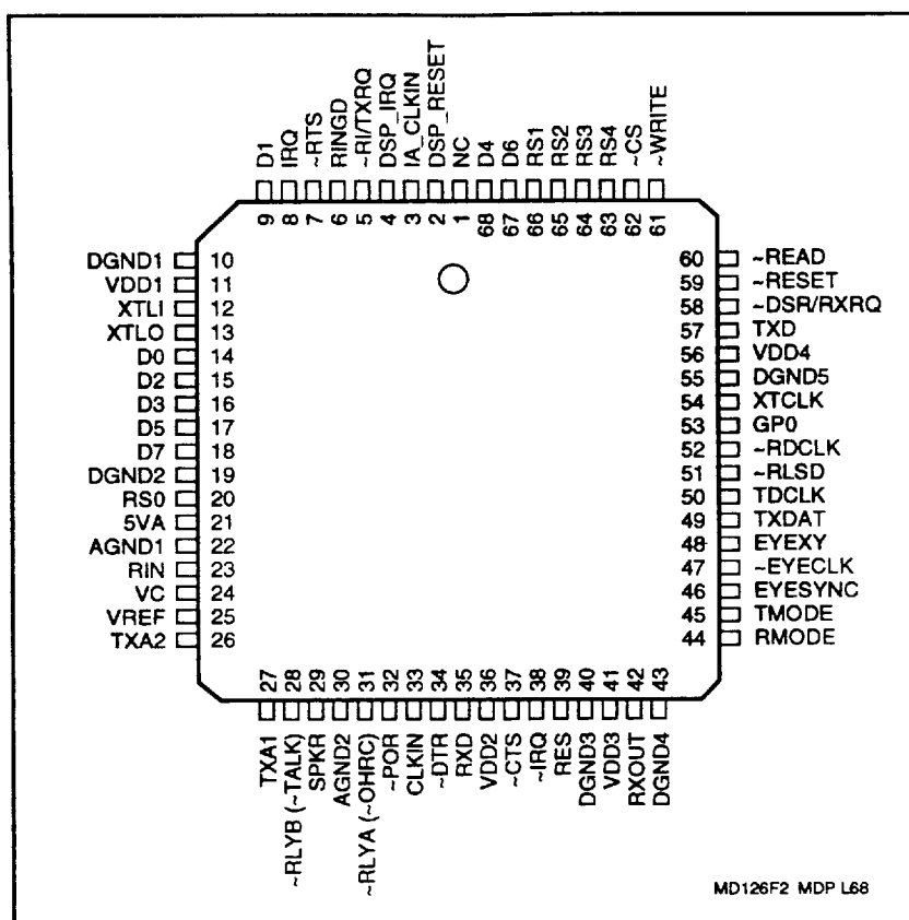
Figure 7. MDP Pin Signals - 68-Pin PLCC
