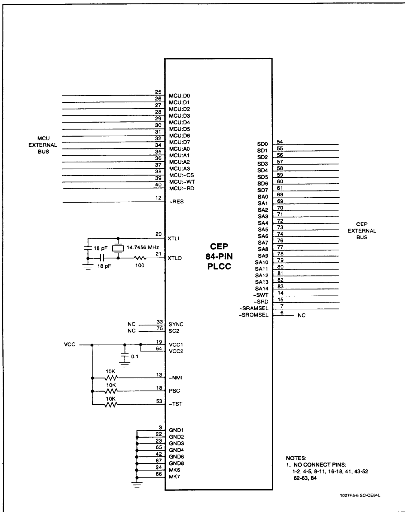
Figure 13. Interface Schematic - CEP - 68-Pin PLCC
