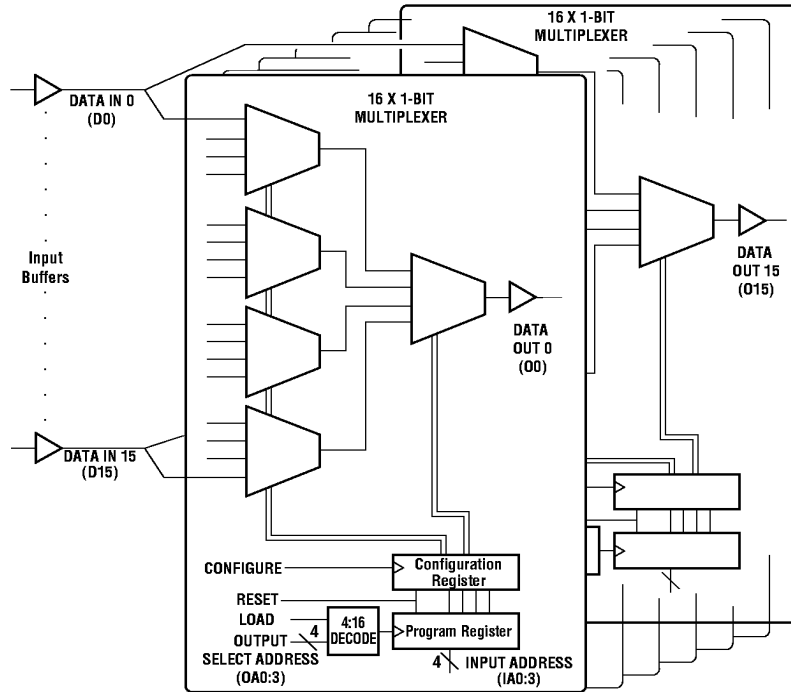
Figure 1. TQ8017 Architecture
