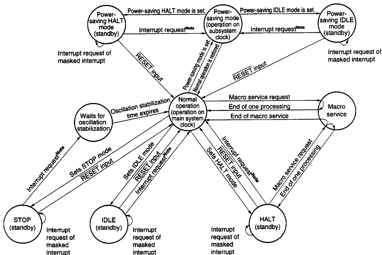
Figure 10-1. Transition of Standby Status
