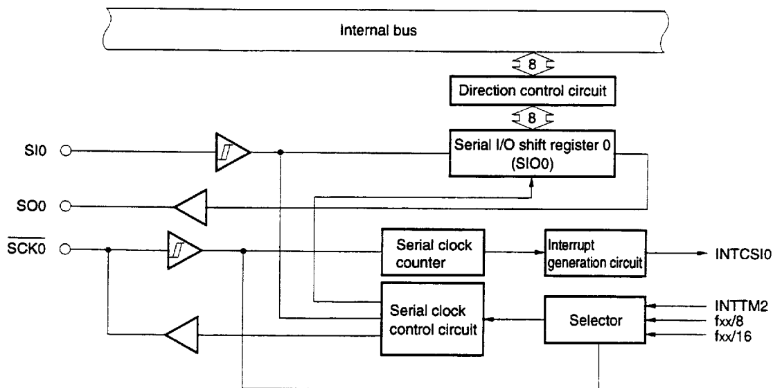
Figure 7-12. Block Diagram in 3-wire Serial I/O Mode
