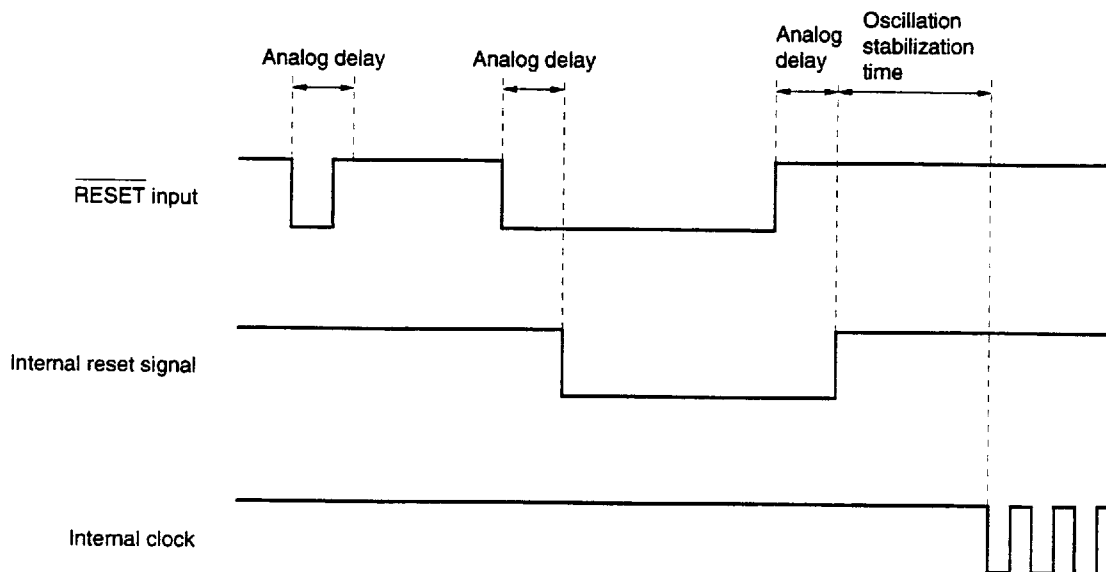
Figure 11-2. Accepting Reset Signal
