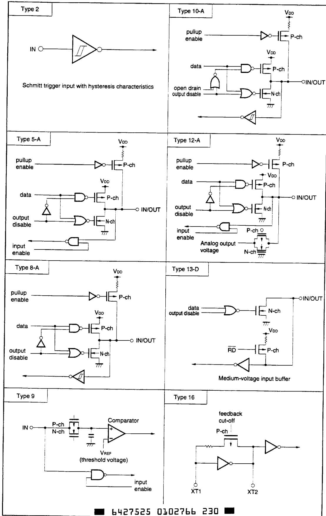
Figure 5-1. Types of Pin I/O Circuits
