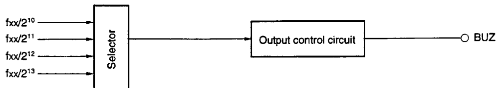
Figure 7-14. Block Diagram of Buzzer Output Function
