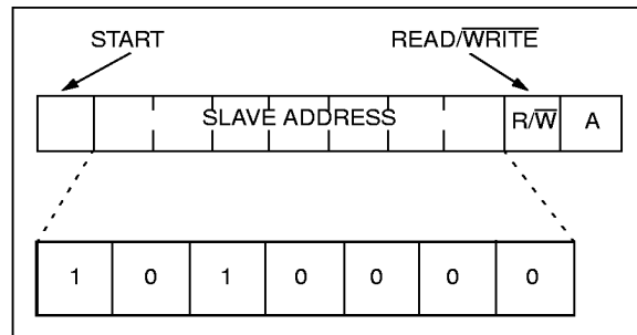
FIGURE 3-5: CONTROL BYTE ALLOCATION
