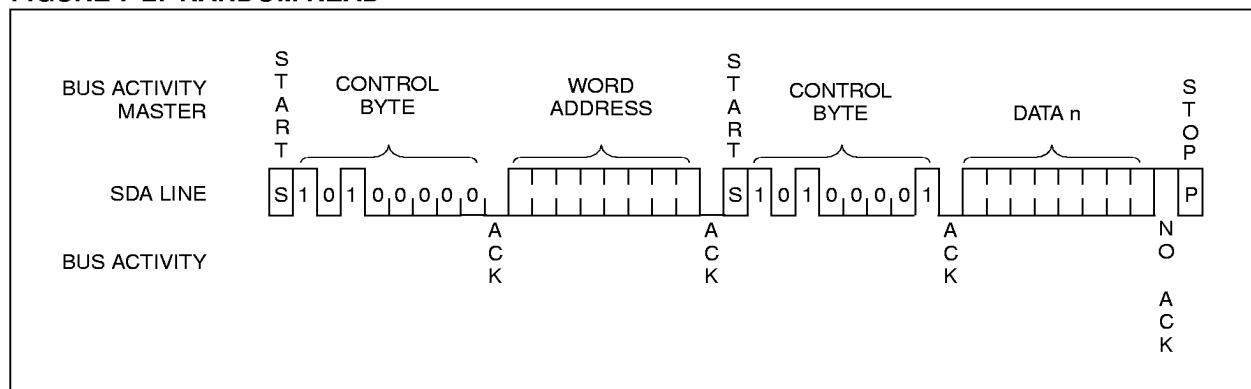
FIGURE 7-2: RANDOM READ
