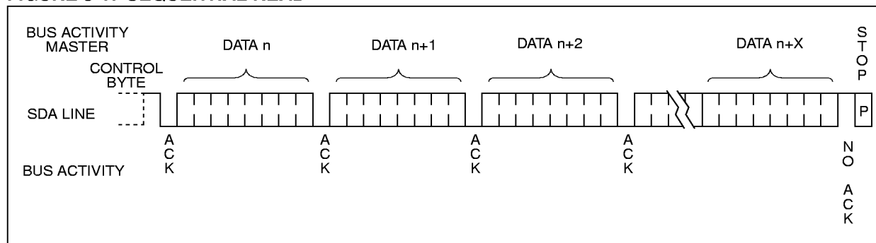
FIGURE 8-1: SEQUENTIAL READ
