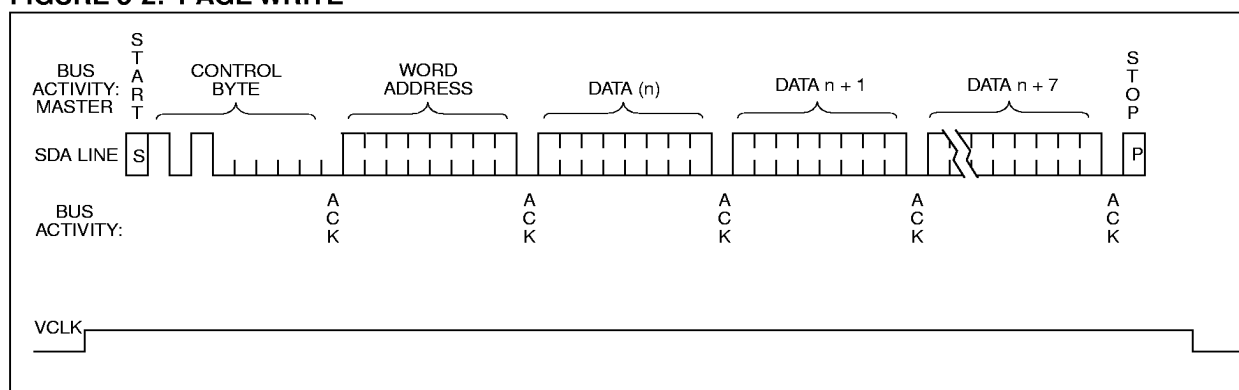
FIGURE 5-2: PAGE WRITE
