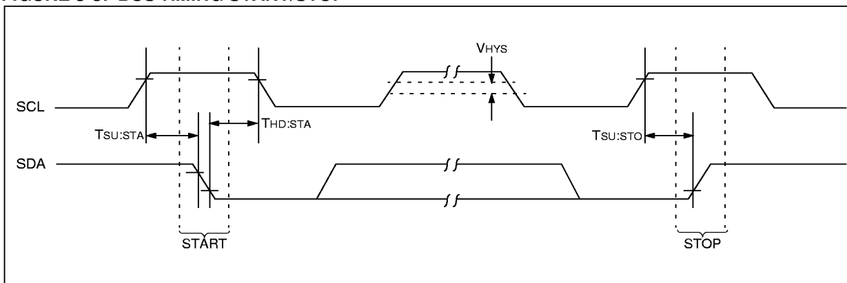
FIGURE 3-4: BUS TIMING DATA
