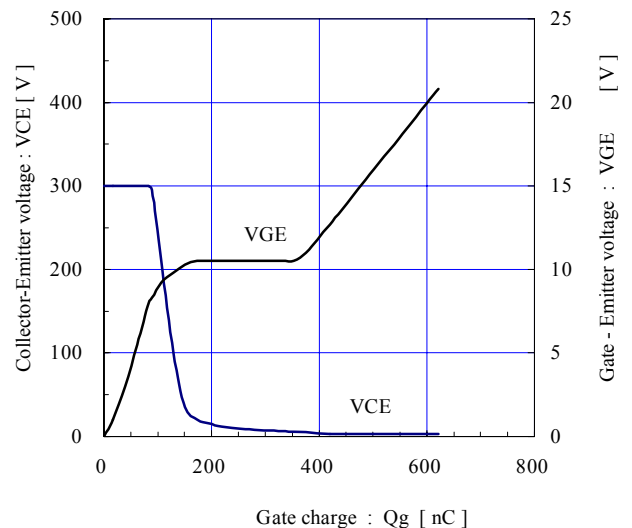
Dynamic Gate charge (typ.) Vcc=300V, Ic=150A, Tj= 25°C
