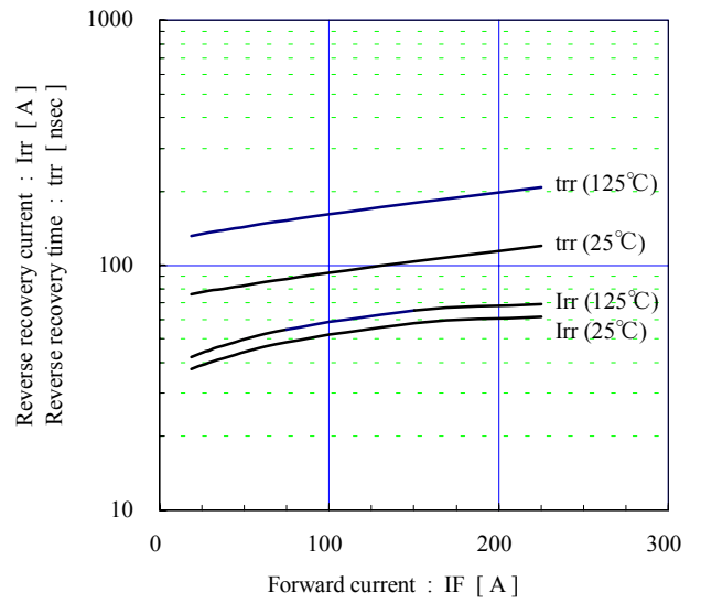
Reverse recovery characteristics (typ.) Vcc=300V, VGE=±15V, Rg=24Ω
