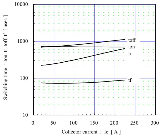
Switching time vs. Collector current (typ.) V_{cc}=300V , V_{GE}=\pm 15V , R_g=24\Omega , T_j=125^\circ C
