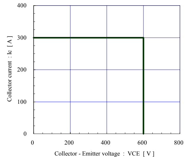
Reverse bias safe operating area (max.) +V_{GE}=15V , -V_{GE} \leq 15V , R_g \geq 24\Omega , T_j \leq 125^\circ C
