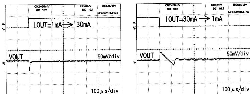
Fig.14 Load Transient response ( C_o=2.2\mu F )
