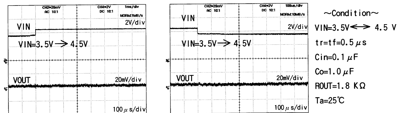
Fig.18 Line Transient response
