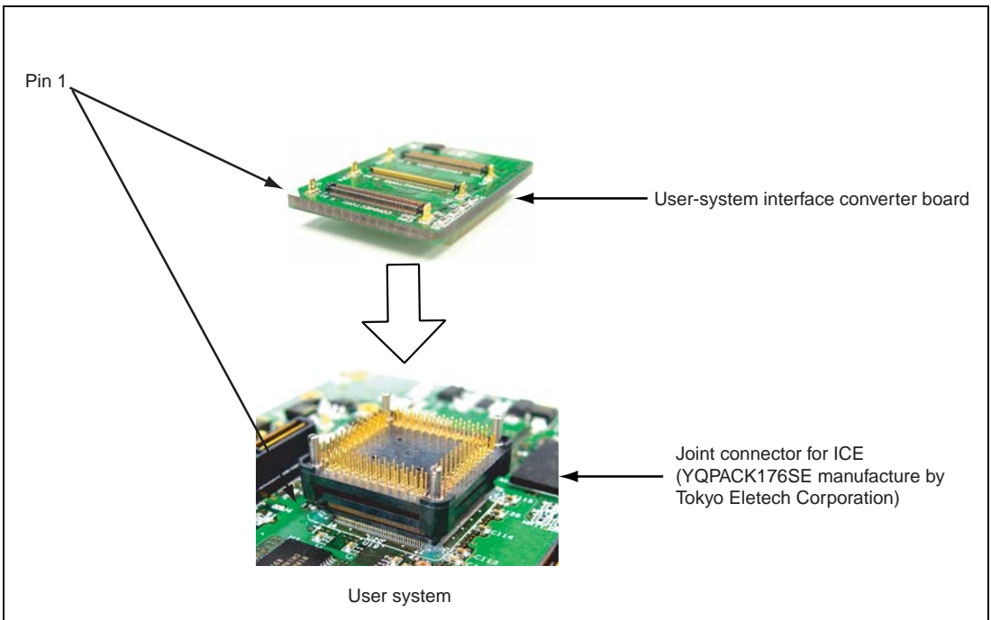
Figure 7 Connecting the User System and User System Interface Board
