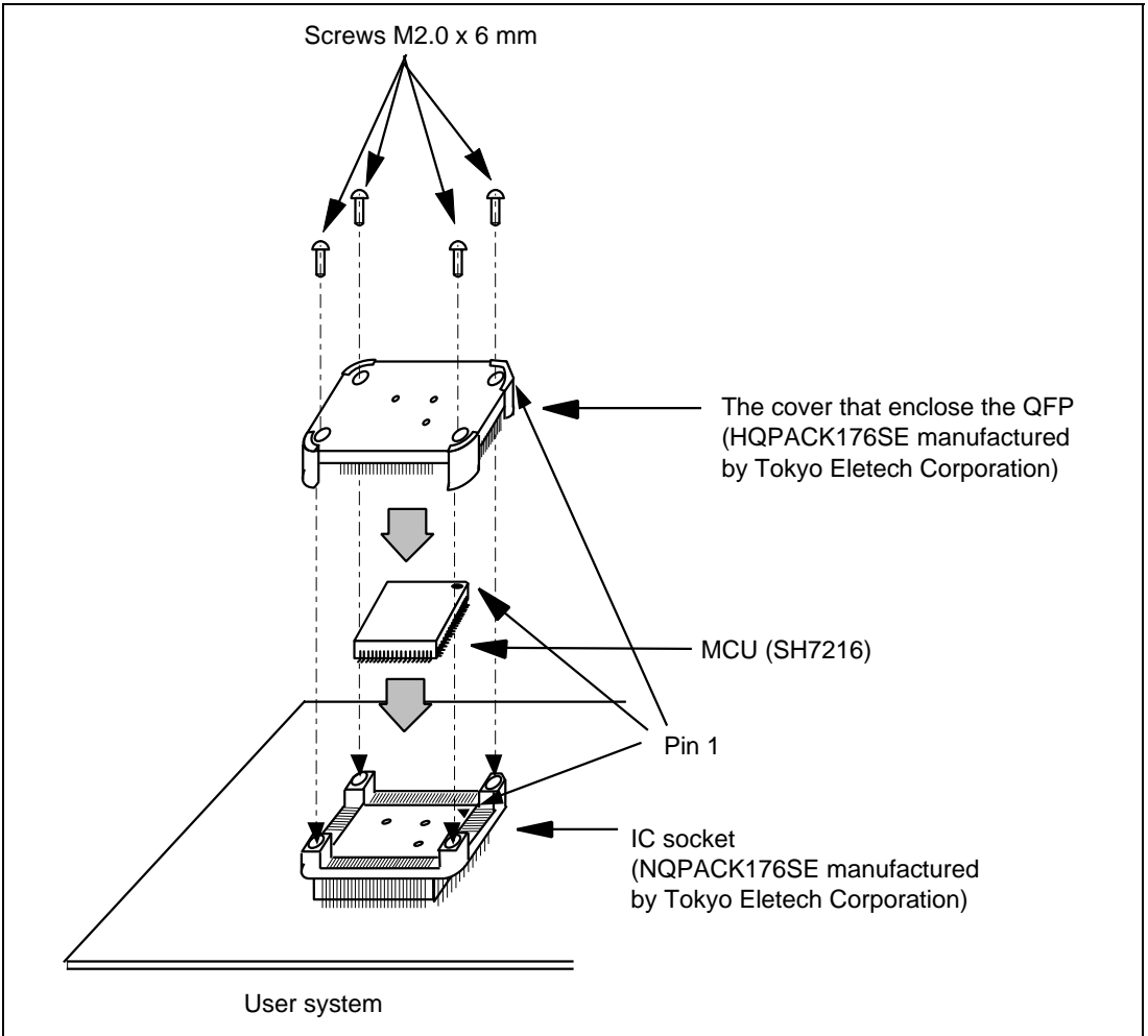
Figure 17 Installing MCU to User System
