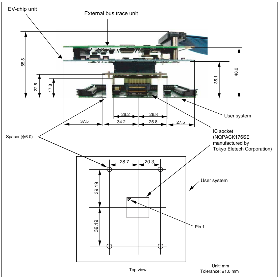
Figure 15 Dimensions of the User System and Connected User-System Interface Converter Board (with the External Bus Trace Unit and EV-chip Unit also Connected)
