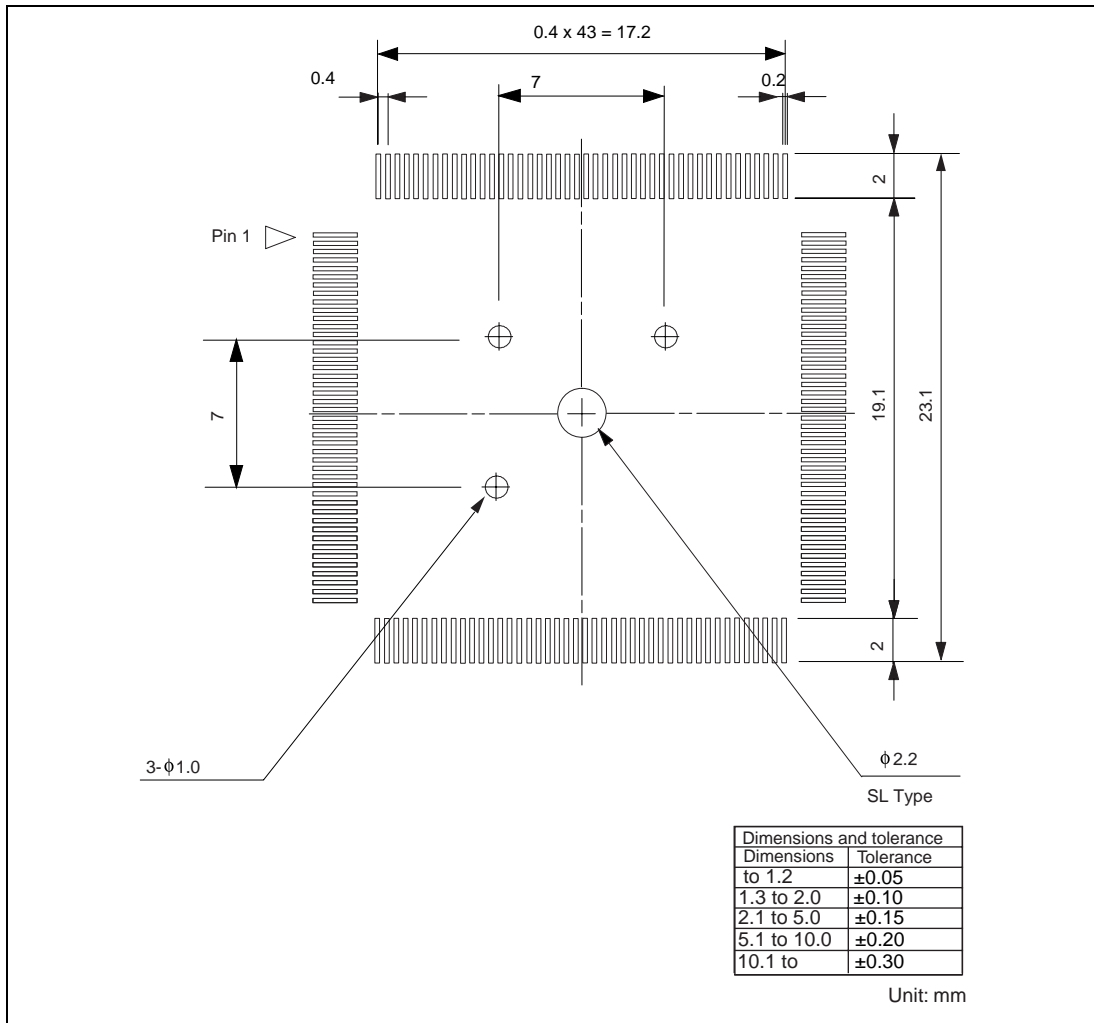
Figure 11 Recommended Dimensions for Mount Pad
