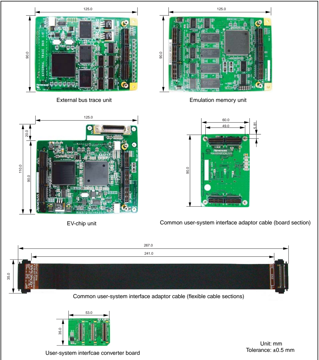
Figure 1 Appearance of the User System Interface Board for SH7216 Group Products in the PLQP0176LB-A Package
