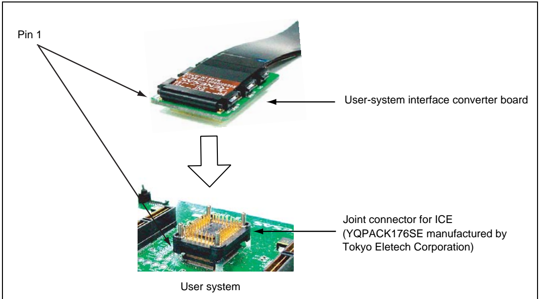
Figure 6 Connecting the User System and User System Interface Board
