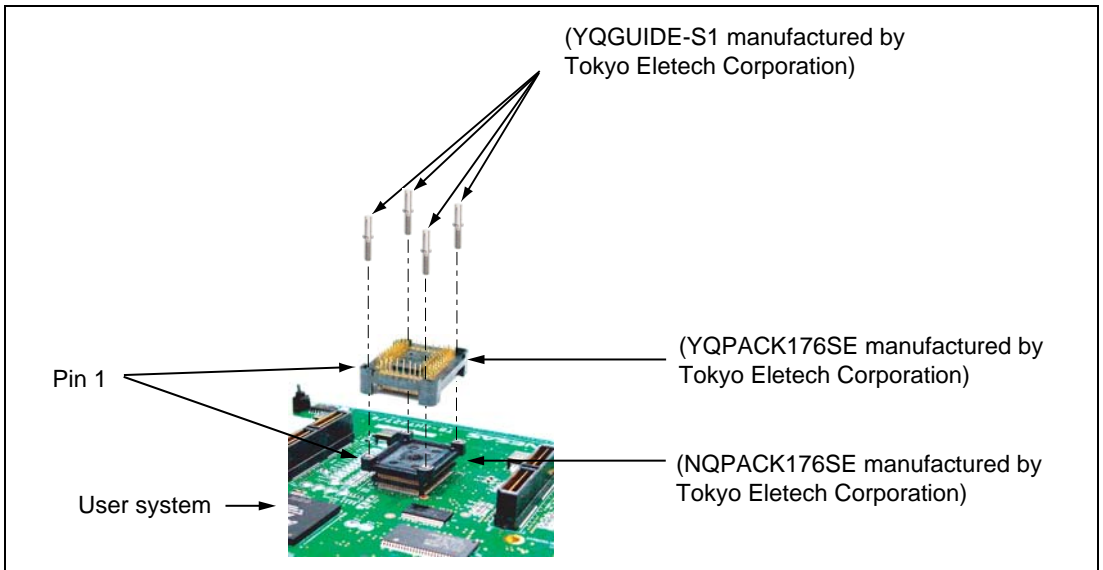
Figure 2 Connecting User System Interface Board to User System
