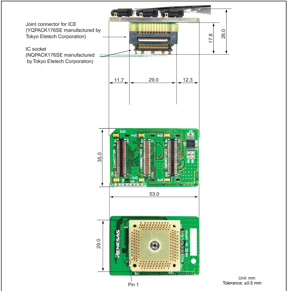
Figure 13 Dimensions of the User-System Interface Converter Board when Connected to the User System (Connection Includes the Flexible Cable)
