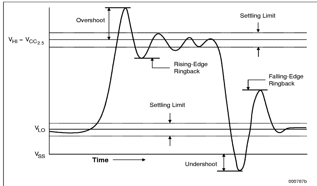
Figure 16. Non-GTL+ Overshoot/Undershoot, Settling Limit, and Ringback
