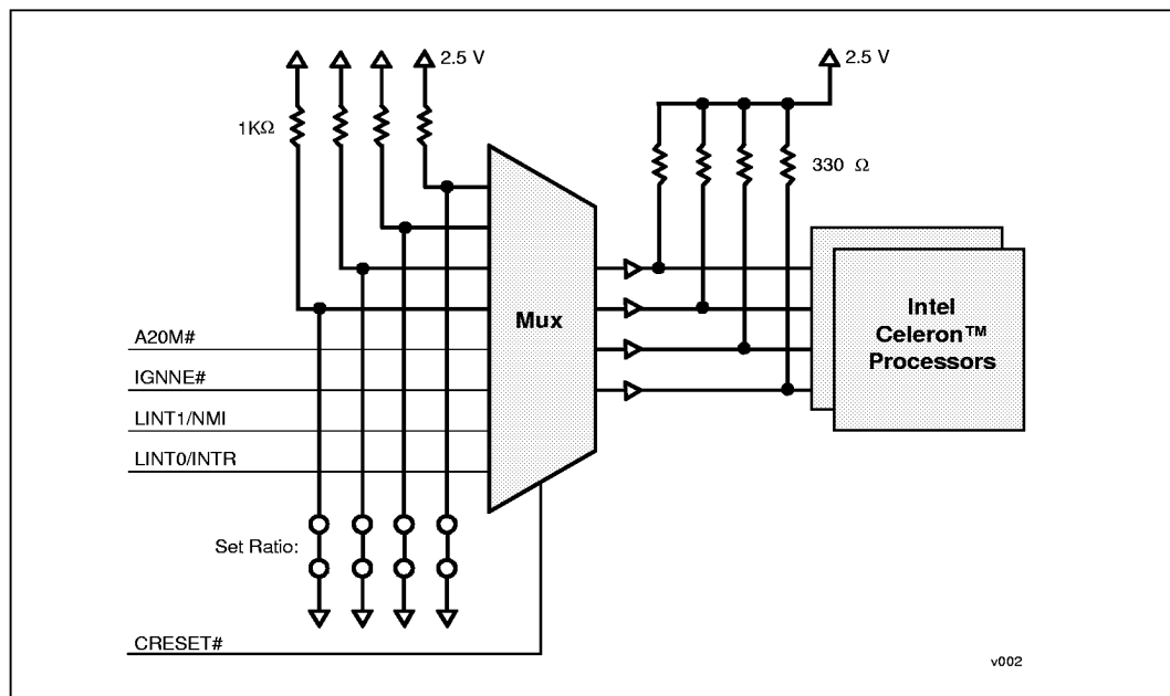
Figure 4. Example Schematic for Forcing a Safe Bus Fraction Ratio
