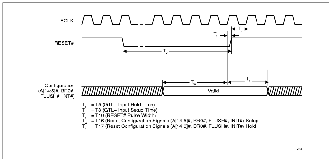
Figure 9. Intel® Celeron™ Processor System Bus Reset and Configuration Timings
