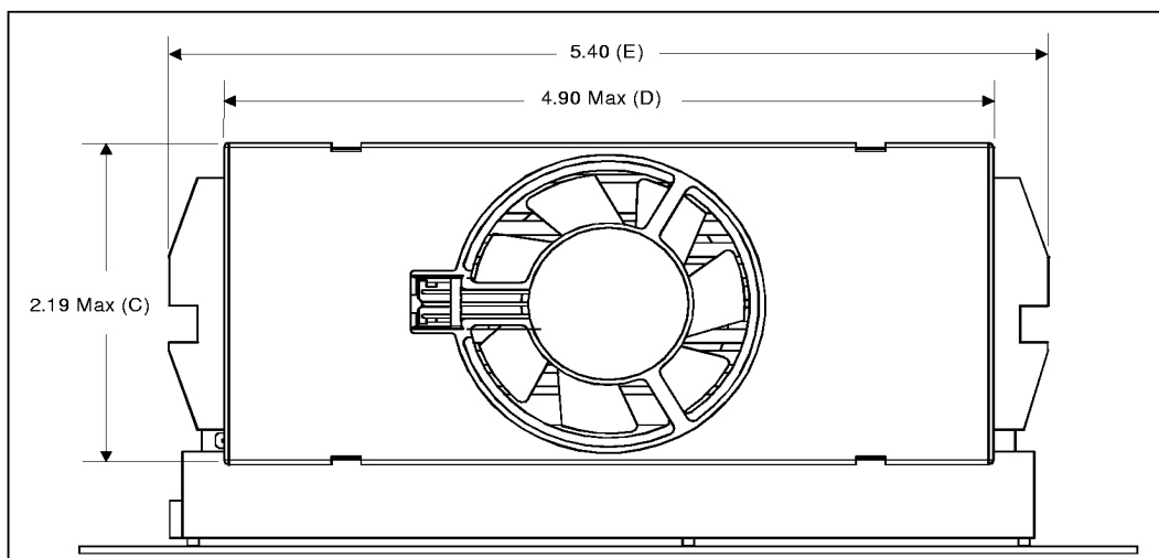
Figure 21. Front View Space Requirements for the Boxed Processor
