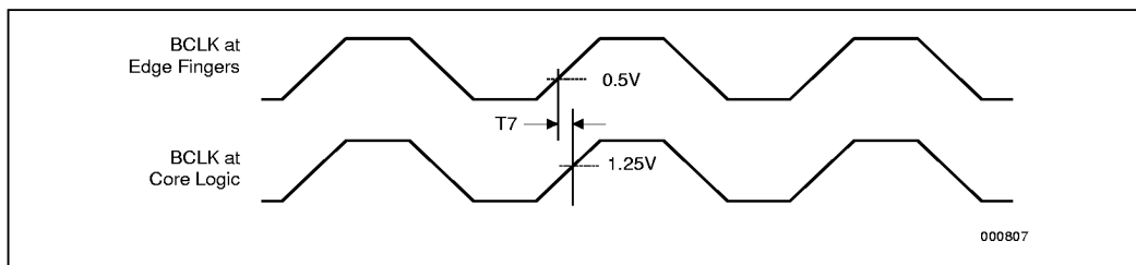
Figure 6. BCLK*, PICCLK, and TCK Generic Clock Waveform
