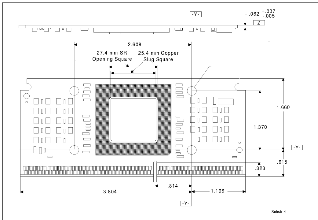
Figure 18. Intel Celeron™ Processor Substrate Primary/Secondary Side Dimensions
