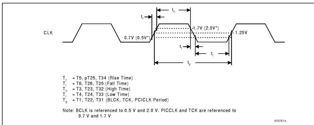
Figure 6. BCLK*, PICCLK, and TCK Generic Clock Waveform
