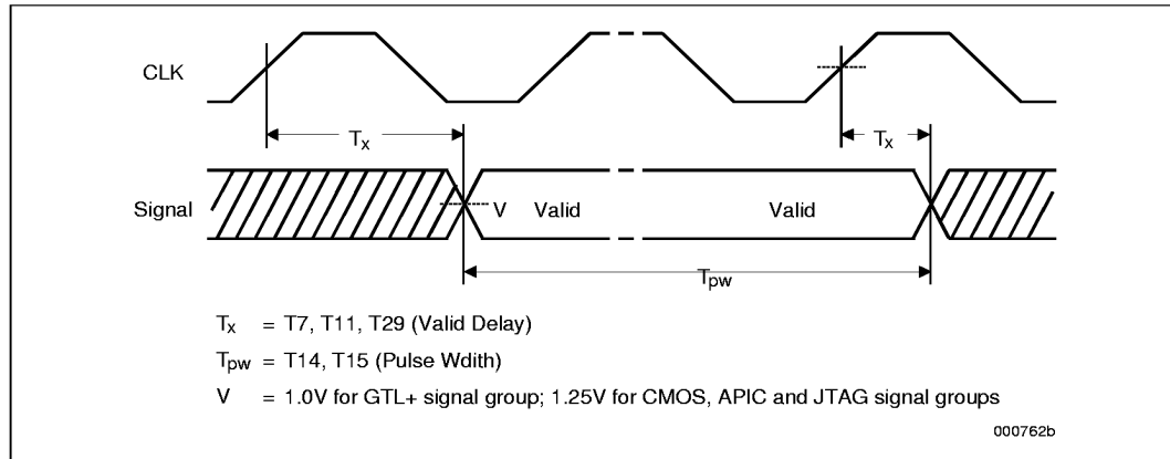
Figure 8. Intel® Celeron™ Processor System Bus Setup and Hold Timings
