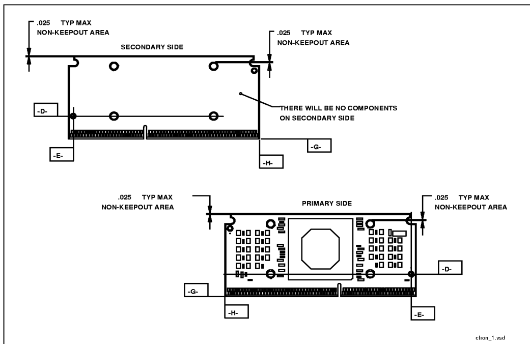
Figure 18. Intel Celeron™ Processor Substrate Primary/Secondary Side Dimensions
