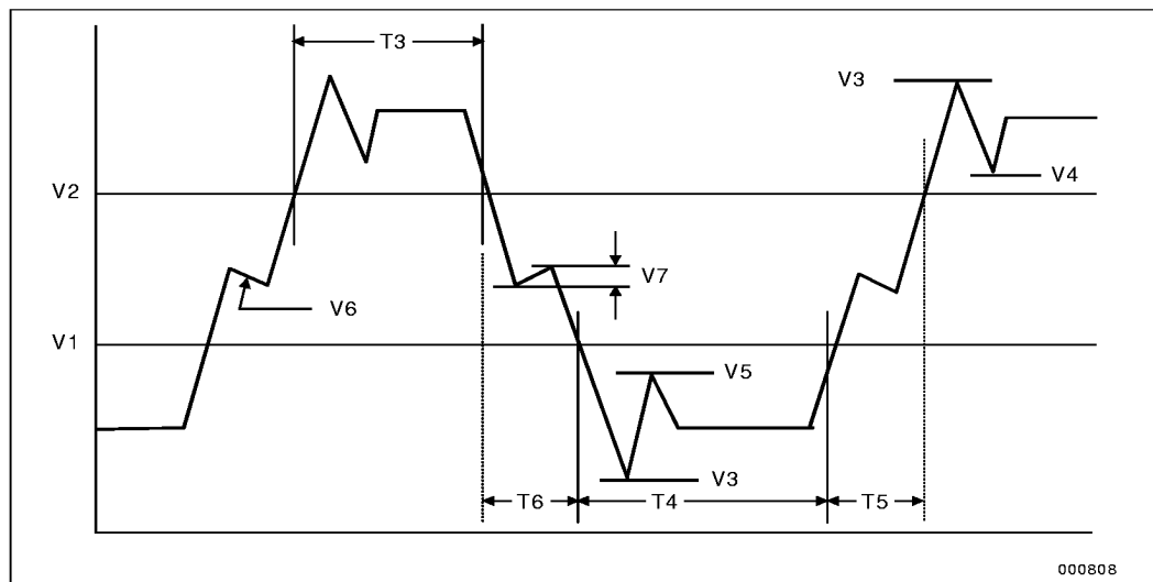
Figure 14. BCLK, TCK, PICCLK Generic Clock Waveform at the Processor Edge Fingers
