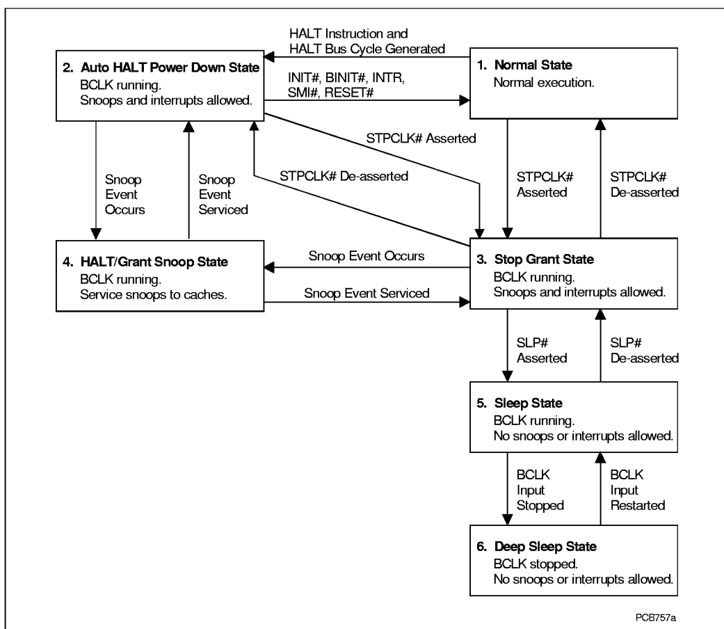
Figure 2. Clock Control State Machine
