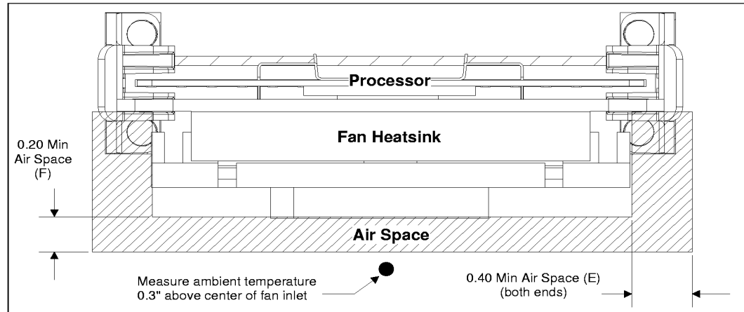
Figure 22. Top View Space Requirements for the Boxed Processor
