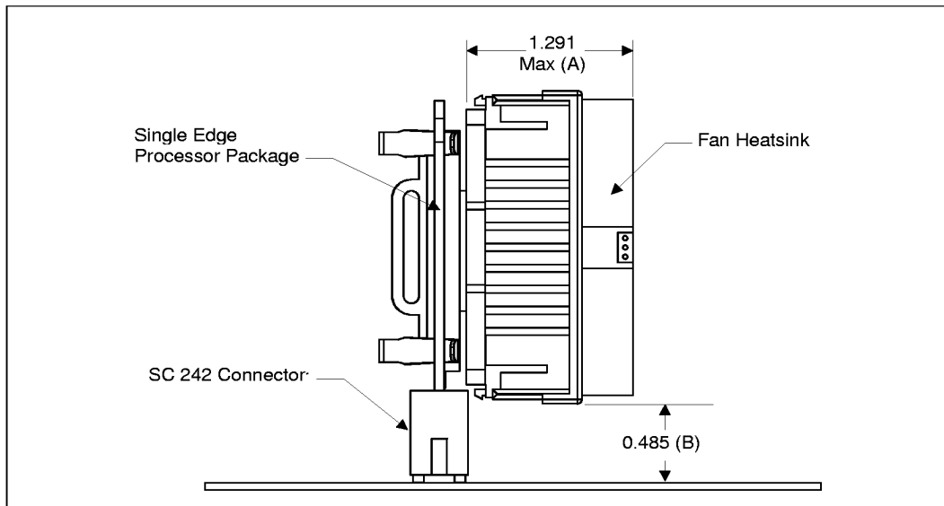
Figure 21. Front View Space Requirements for the Boxed Processor
