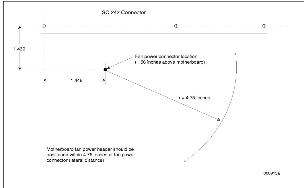
Figure 24. Motherboard Power Header Placement Relative to Fan Power Connector and SC 242
