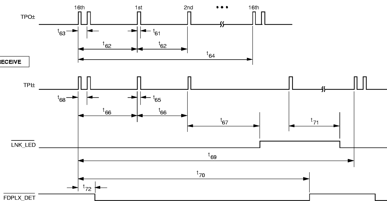
Figure 9. Link Pulse Timing
