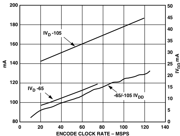
TPC 20. I_{VD} and I_{VDD} vs. Encode Rate ( A_{IN} = 10.3 MHz, @ -0.5 dBFS). -65/-105 MSPS Grade Cl = 5 pF
