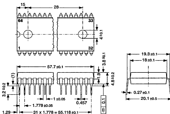
Fig. 4-2: 64-Pin Plastic Shrink Dual-Inline-Package (PSDIP64) Weight approx. 9.0 g Dimensions in mm
