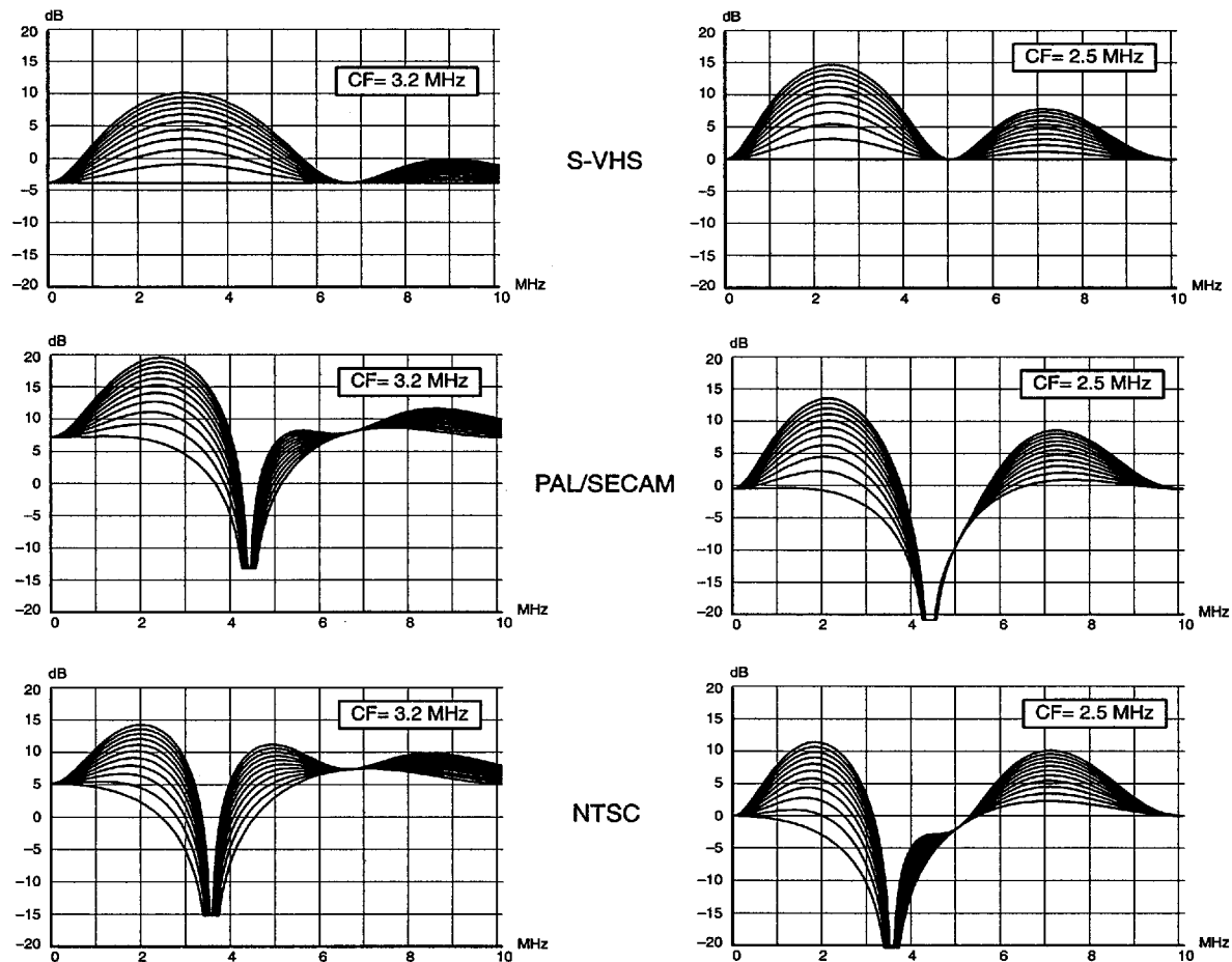
Fig. 2-4: Total frequency response for peaking filter and S-VHS, PAL, NTSC
