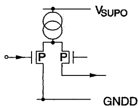
Fig. 4-15: Output pins for Vert and E/W
