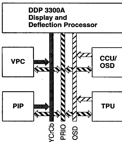
Fig. 1–3: DDP video interfaces
