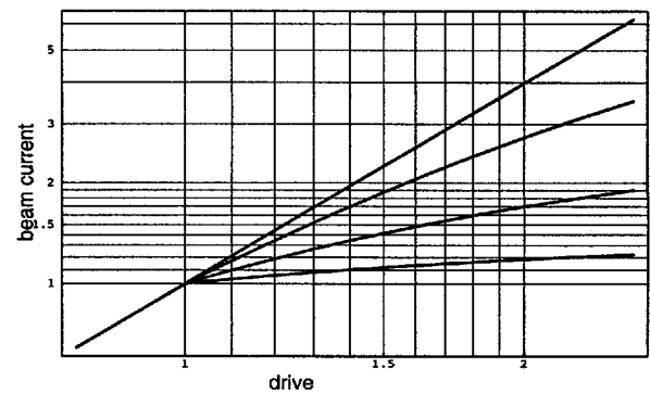
Fig. 2-13: Beam current limiter characteristics: beam current output vs. drive BCL threshold: 1
