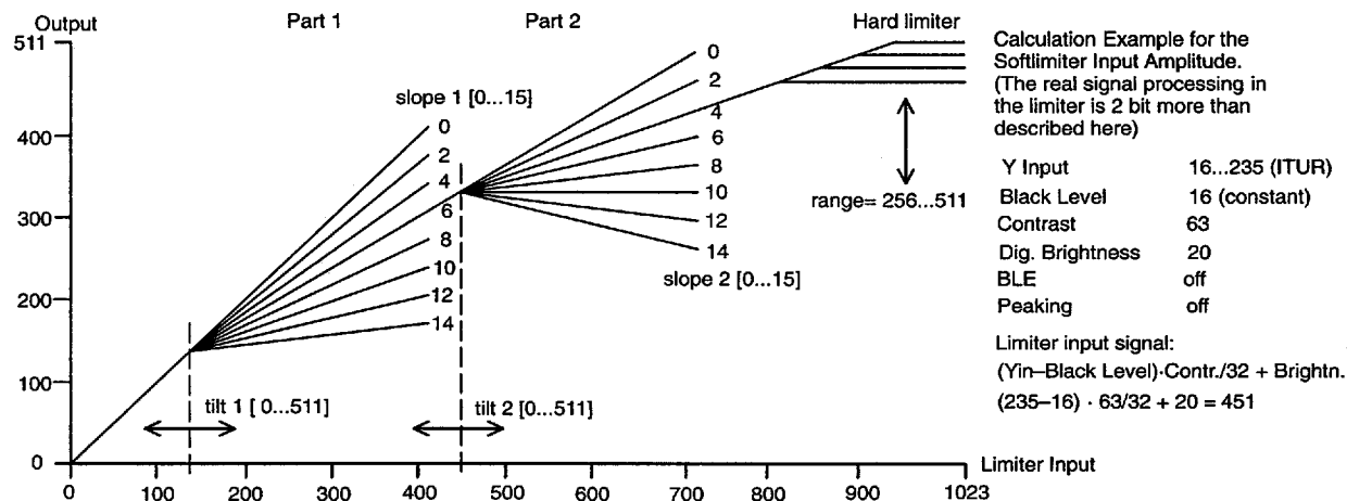
Fig. 2-5: Characteristic of soft limiter a and b and hard limiter
