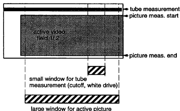
Fig. 2-12: Windows for tube and picture measurements
