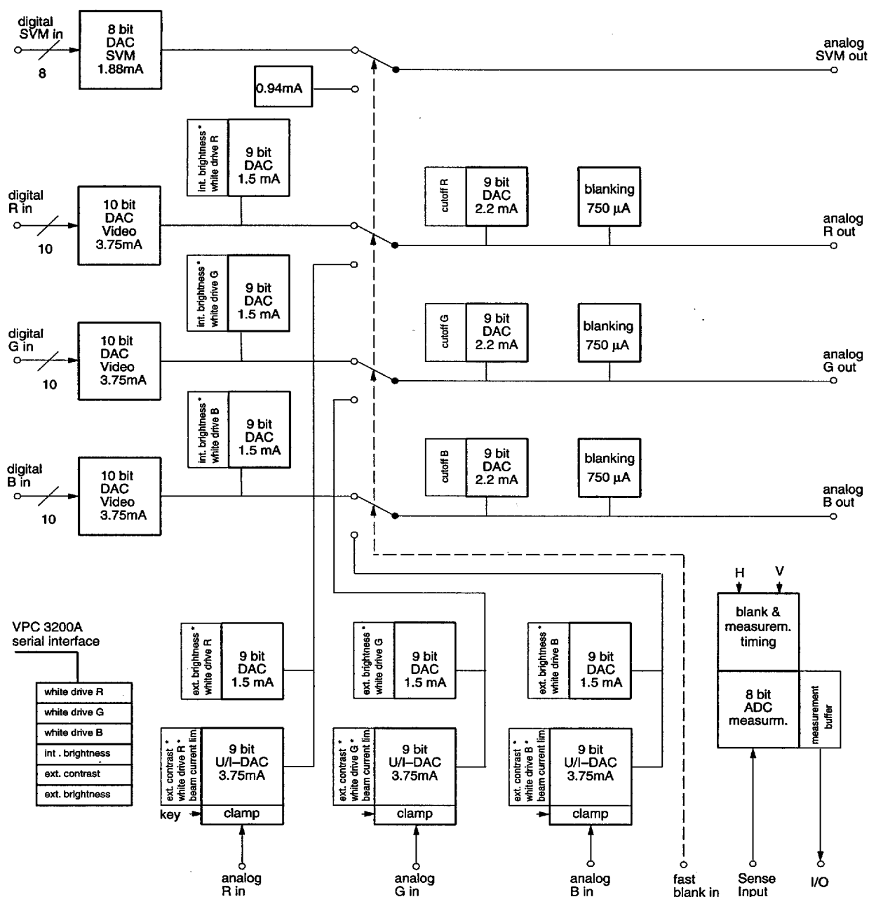
Fig. 2-14: Analog back-end
