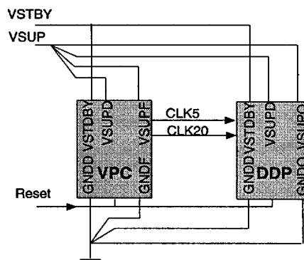
Fig. 2-19: VPC & DDP Supply and Clock
