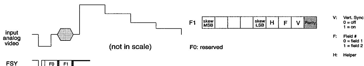
Fig. 2-15: Front sync format
