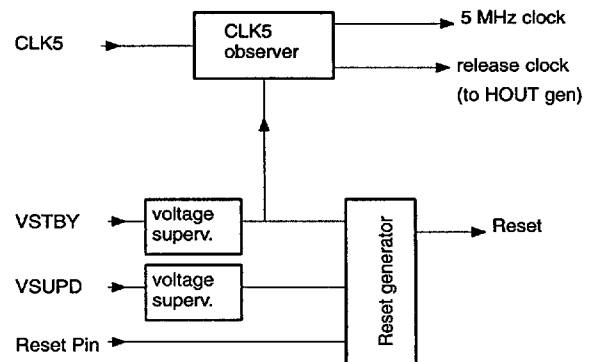
Fig. 2-22: DDP reset generation
