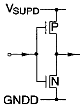
Fig. 4-11: Input pins C[7:0], L[7:0], OSD[4:0], FSX
