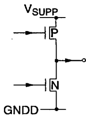
Fig. 4-5: Output pins MSY, CSY
