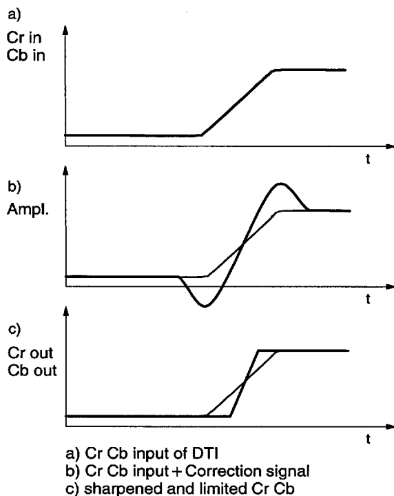
Fig. 2-7: Digital Color Transient Improvement
