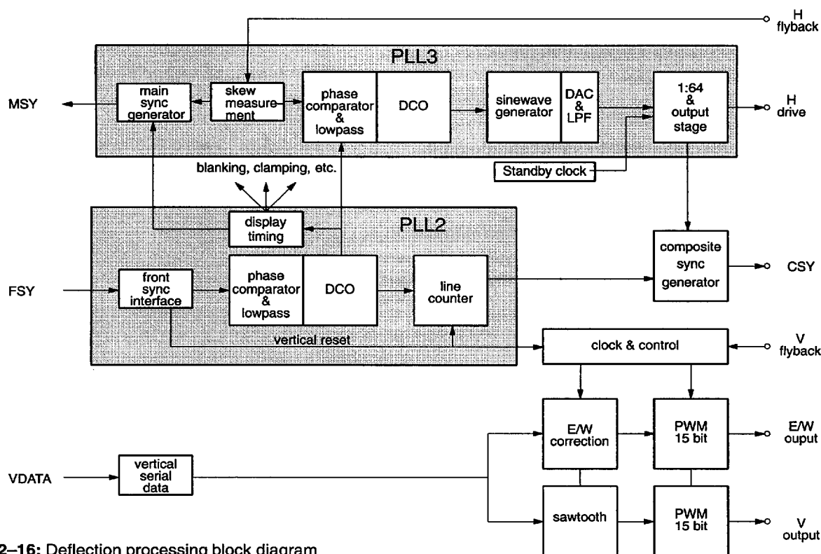
Fig. 2-16: Deflection processing block diagram
