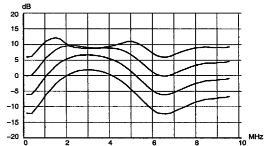
Fig. 2-3: Dynamic peaking frequency response
