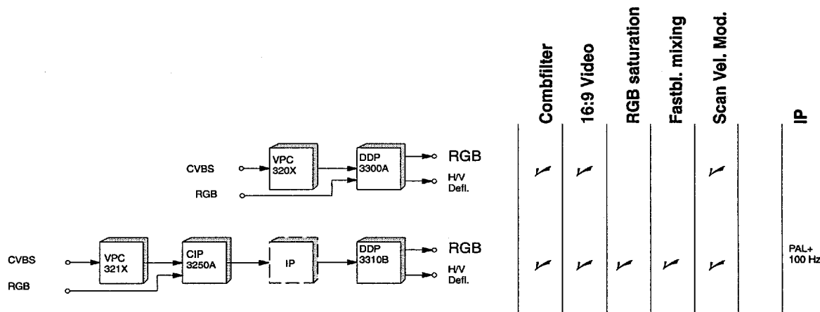
Fig. 1–2: DDP 3300 A Applications
