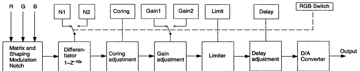
Fig. 2-8:SVM Block diagram
