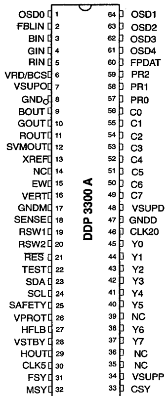
Fig. 4-4: Pinning of the DDP 3300 A in PSDIP64 Package
