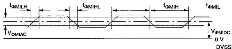
Fig. 4–18: Main clock input
