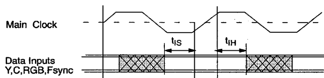
Fig. 4–17: Picture bus input timing
