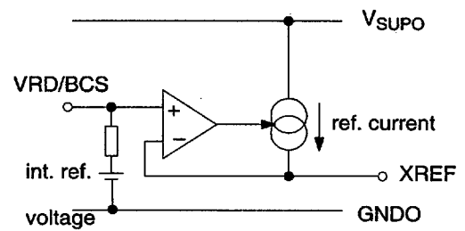
Fig. 4-16: Input pins XREF and VRD/BCS
