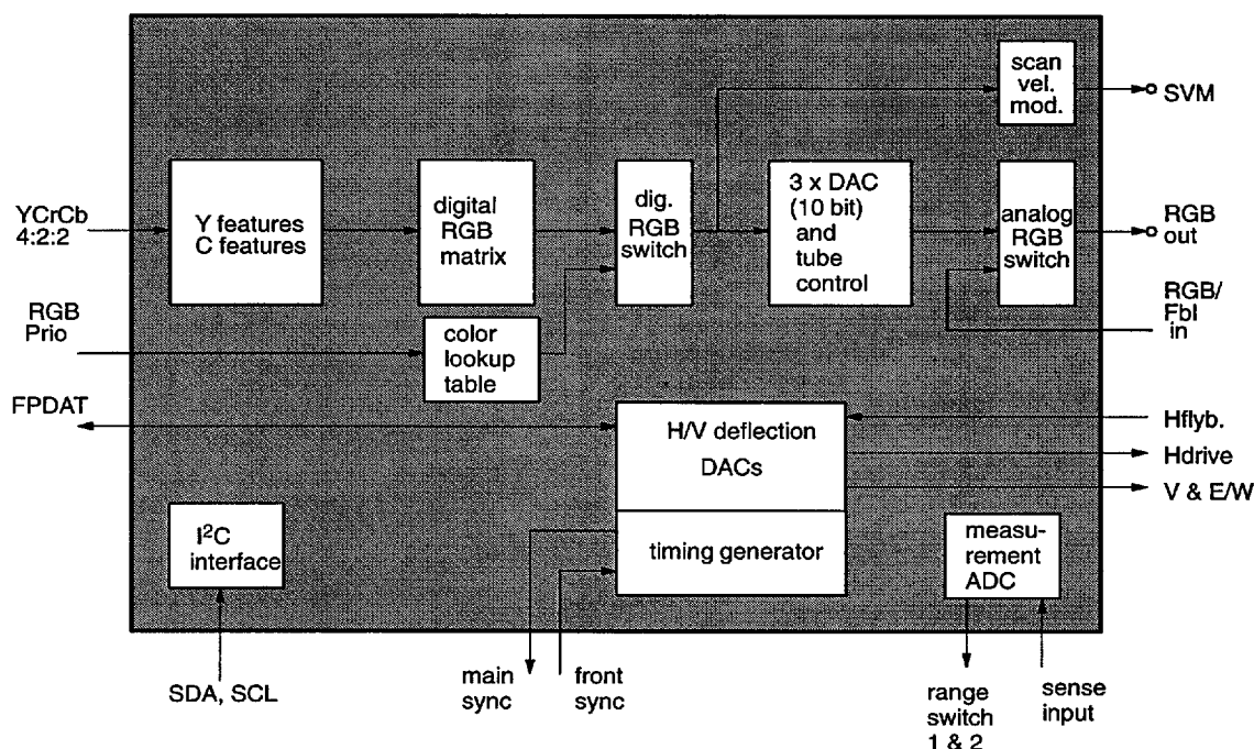
Fig. 1–1: Display and Deflection Processor
