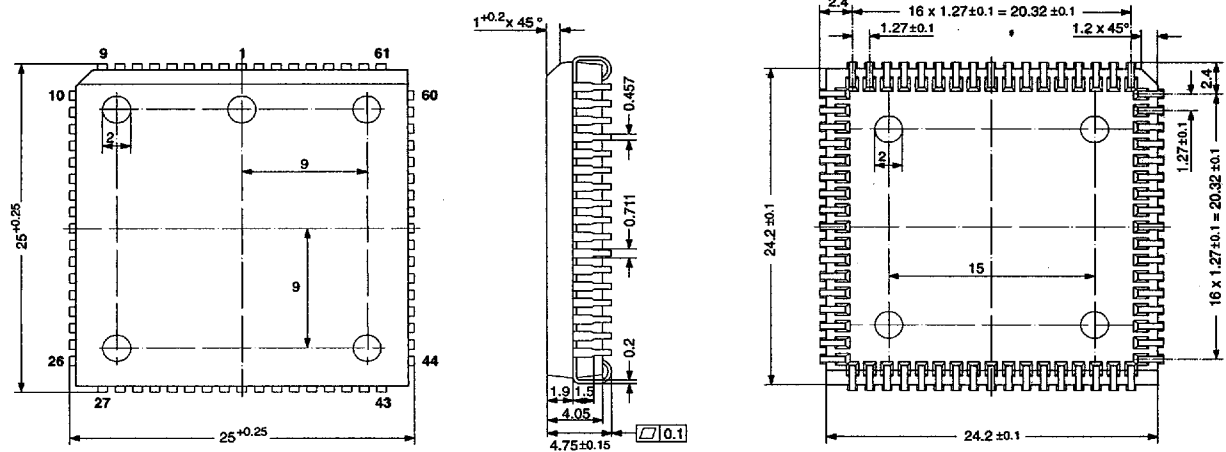
Fig. 4-1: 68-pin Plastic Leaded Chip Carrier Package (PLCC68) Weight approx. 4.8 g Dimensions in mm
