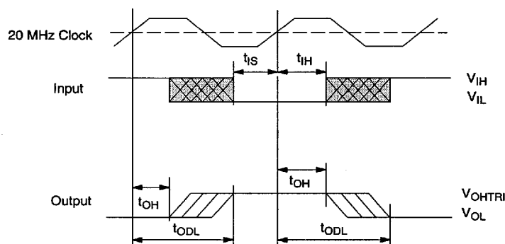
Fig. 4-20: Serial deflection interface
