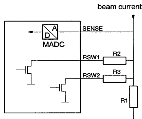
Fig. 2-10: MADC Range Switches
