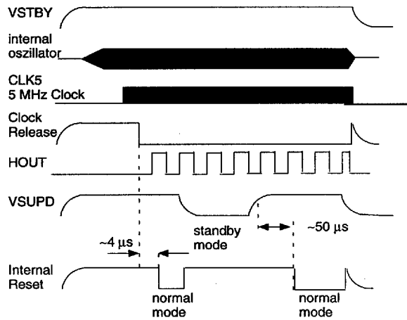
Fig. 2-20: DDP power on, standby on/off
