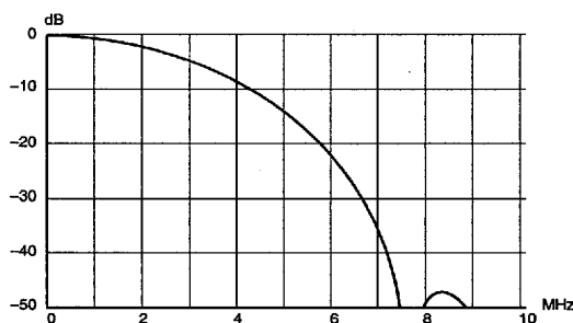
Fig. 2-6: Frequency response of the chroma interpolation filter
