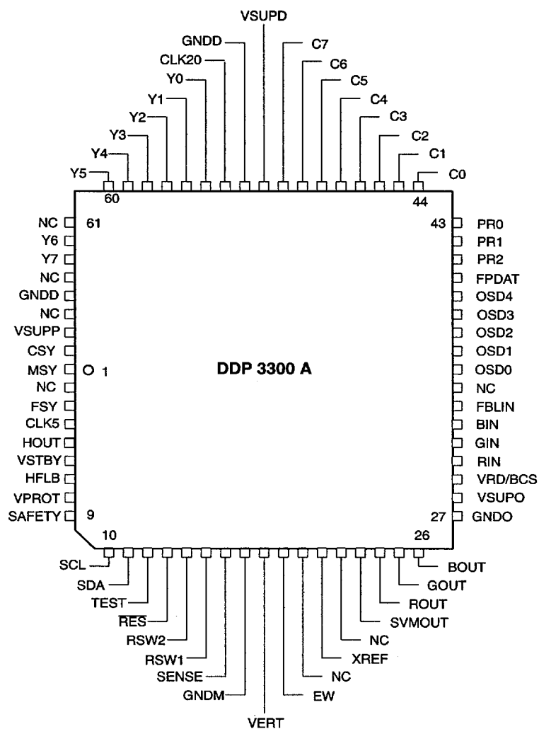
Fig. 4-3: Pinning of the DDP 3300 A in PLCC68 Package
