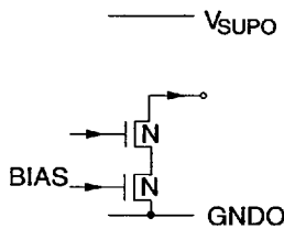
Fig. 4-12: Analog output pins ROUT, GOUT, BOUT, SVMOUT
