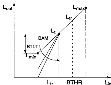
Fig. 2-1: Characteristics of the black level expander
