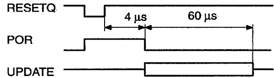
Fig. 2-21: External RESET
