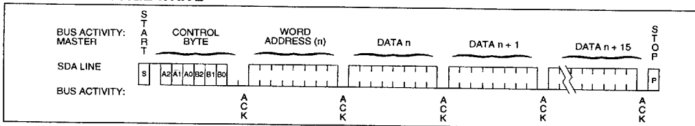
FIGURE 5-2: PAGE WRITE
