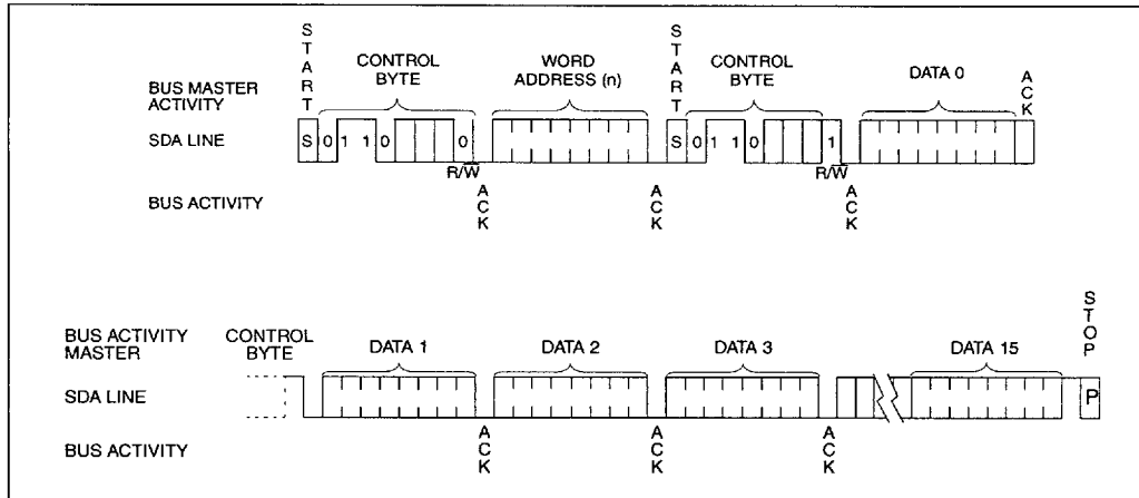
FIGURE 9-6: SECURITY PAGE WRITE
