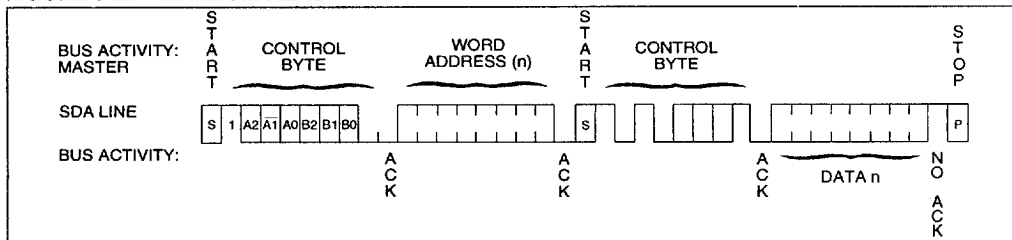
FIGURE 9-3: SEQUENTIAL READ
