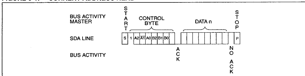
FIGURE 9-2: RANDOM READ
