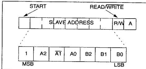
FIGURE 5-1: BYTE WRITE
