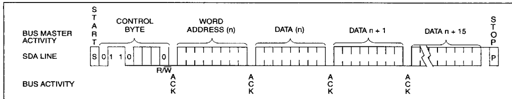
FIGURE 9-6: SECURITY PAGE WRITE
