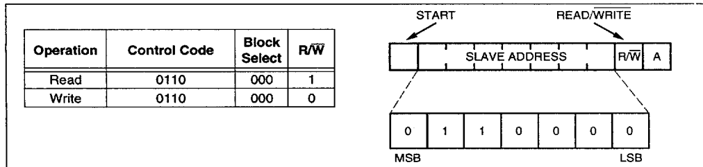
FIGURE 9-4: SECURITY CONTROL BYTE ALLOCATION
