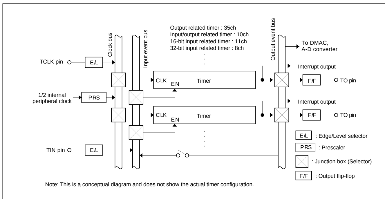
Figure 20 Conceptual Diagram of the Multijunction Timer (MJT)
