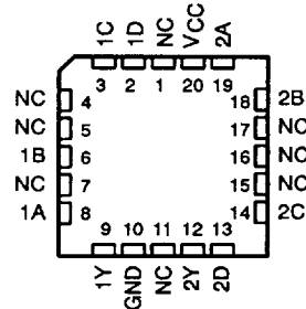
54ACT11021 ... FK PACKAGE (TOP VIEW)
