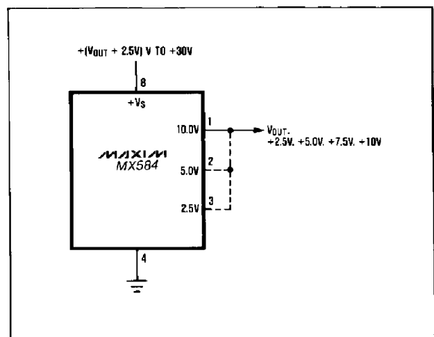
Figure 1. Basic Connection for Positive Outputs
