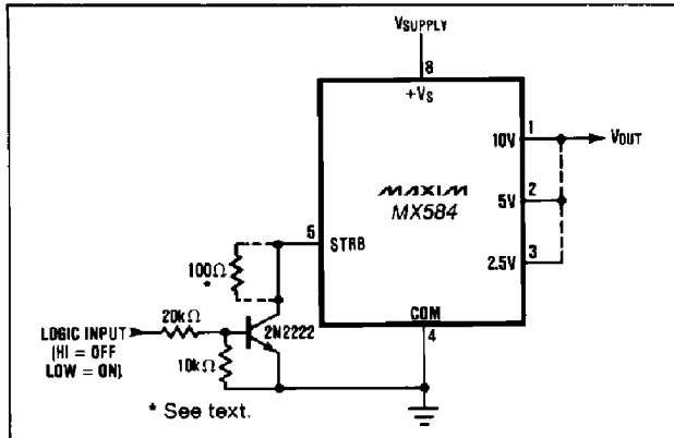
Figure 5. Use of Strobe Terminal
