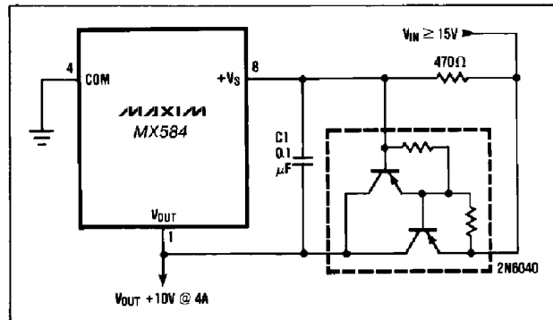
Figure 6. High Current Precision Supply
