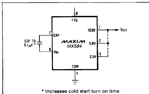
Figure 4. Additional Noise Filtering with an External Capacitor
