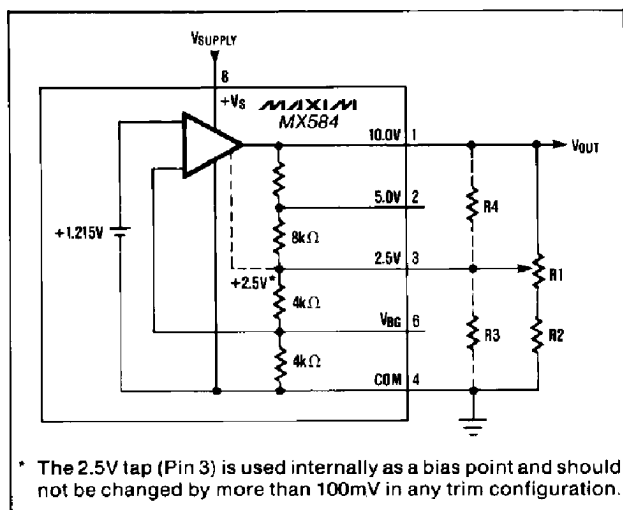
Figure 2. Variable Output Options
