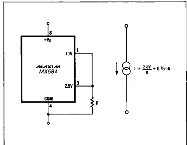
Figure 8. Precision Current Limiter
