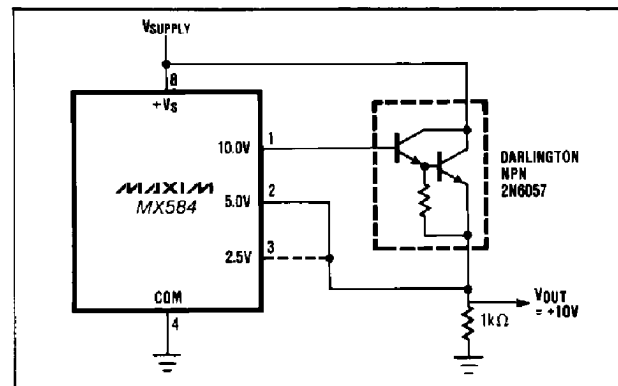
Figure 7. NPN Output Current Booster
