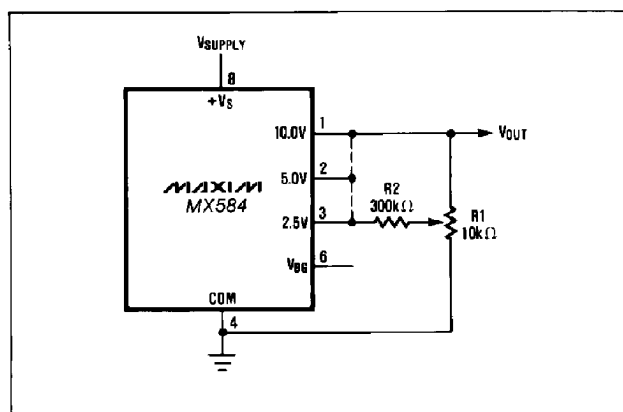
Figure 3. Fine Adjustment of Output Voltage ( \pm 200\text{mV} )
