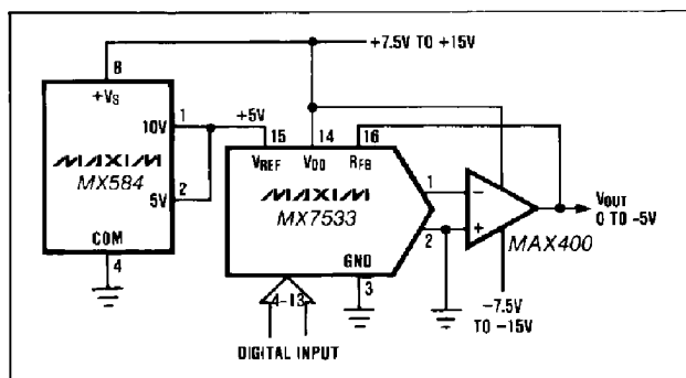
Figure 10. Low Power 10 Bit CMOS DAC Connection
