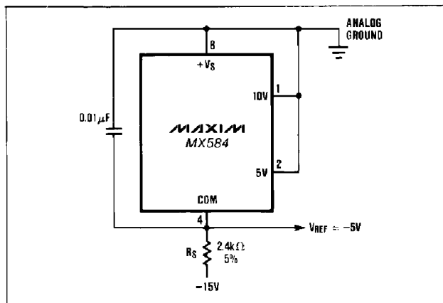
Figure 9. Two-Terminal -5 Volt Reference
