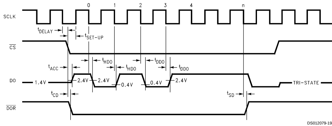
DO Data Output Timing Using \overline{\text{CS}}
