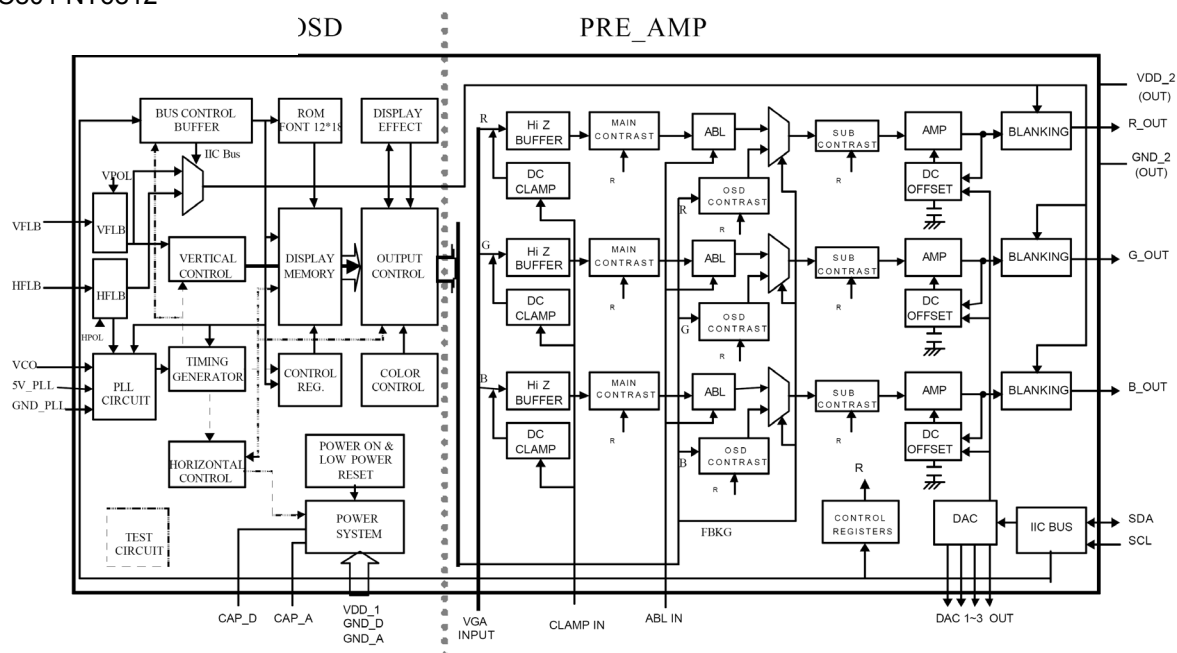
IC801 NT6812
