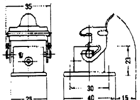
Montageausschnitt/Panel cut-out 22 x 22
