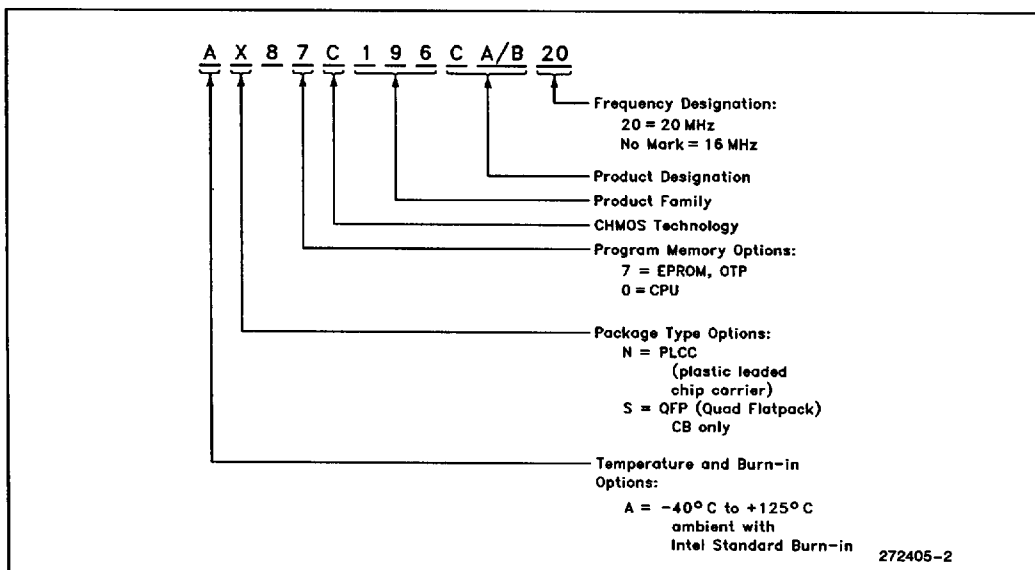
Figure 2. The 87C196CA/CB Family Nomenclature
