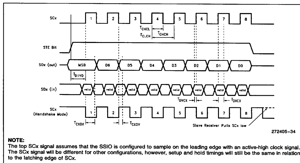
Figure 6. Synchronous Serial Port
