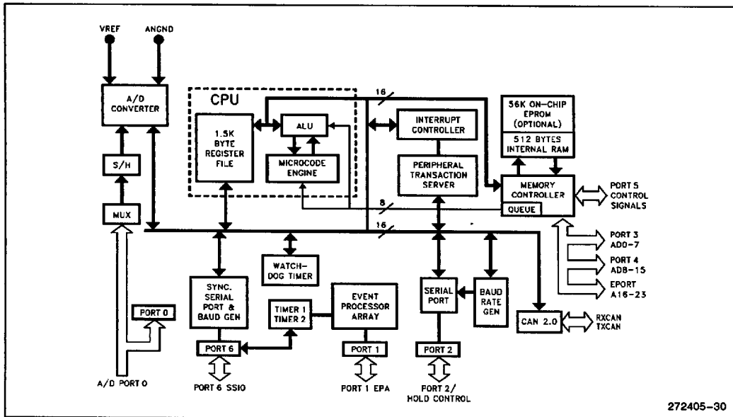
Figure 1. 8XC196CB Block Diagram
