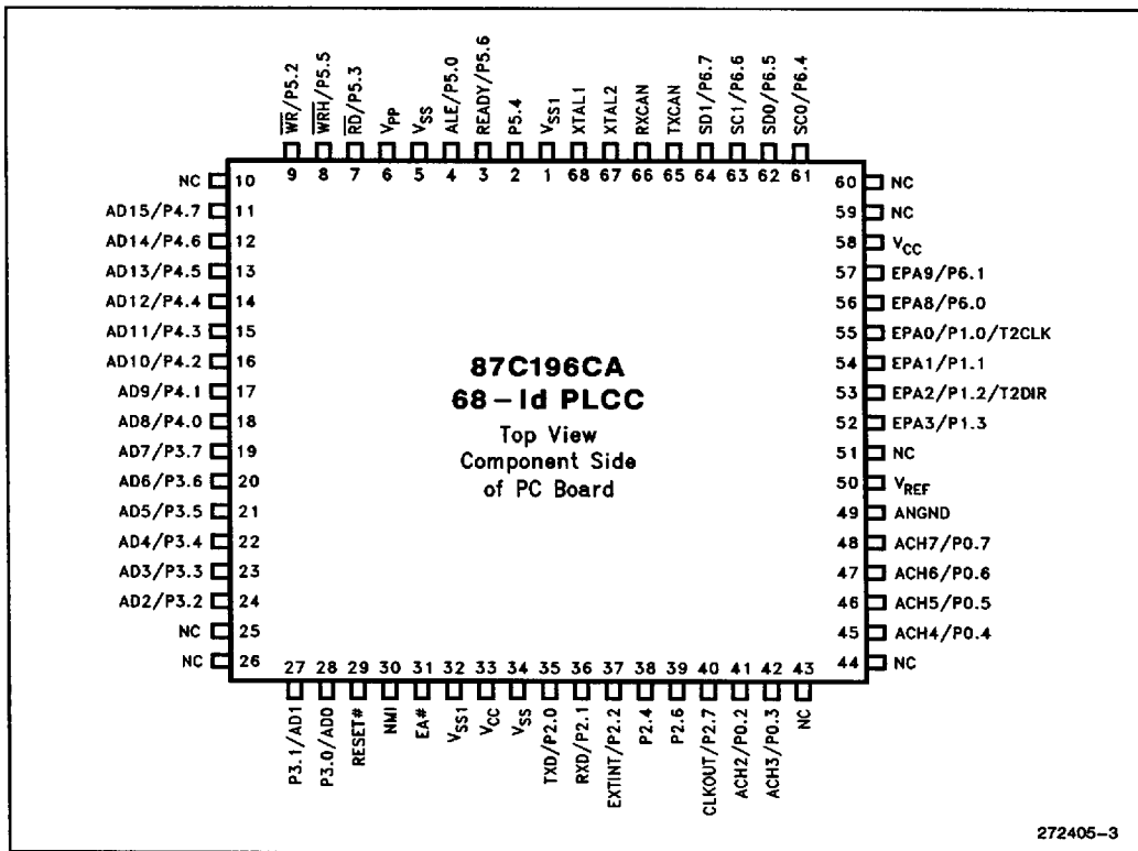
Figure 5. 68-Pin PLCC 87C196CA Diagram
