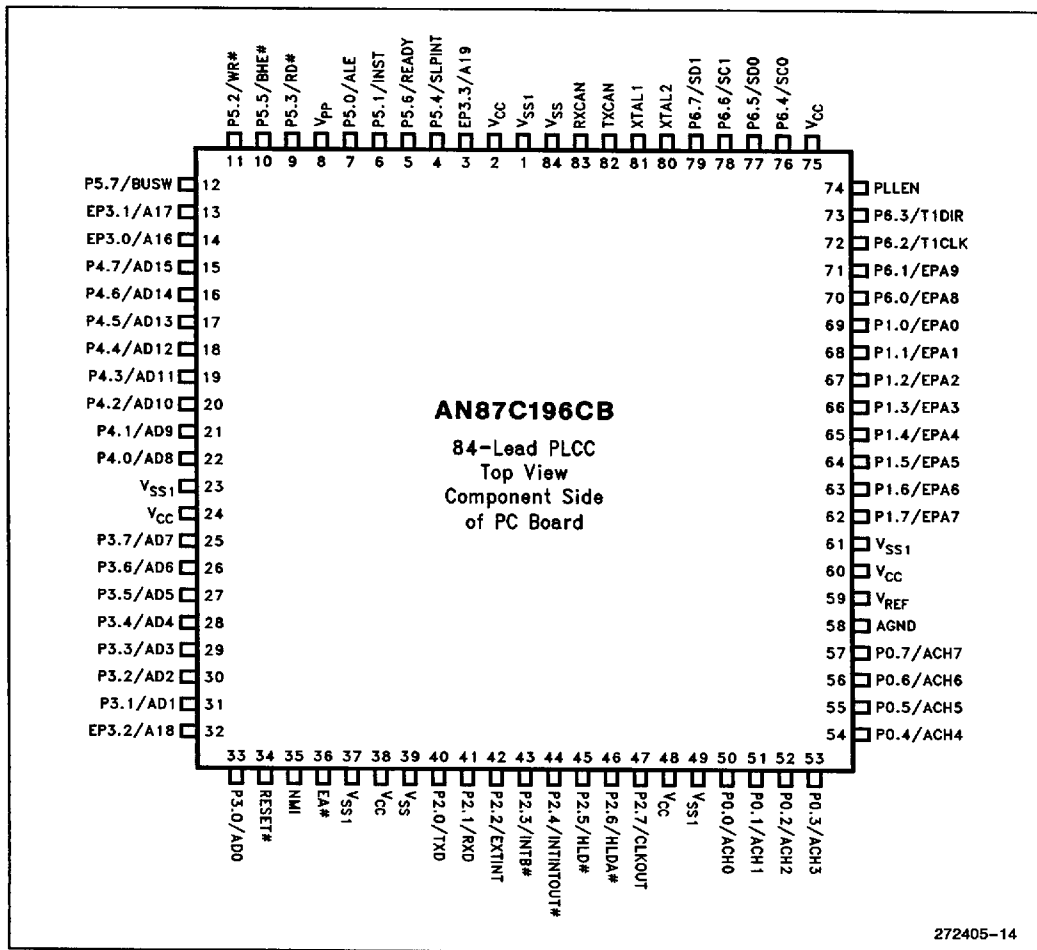
Figure 3. 84-Pin PLCC AN87C196CB Diagram
