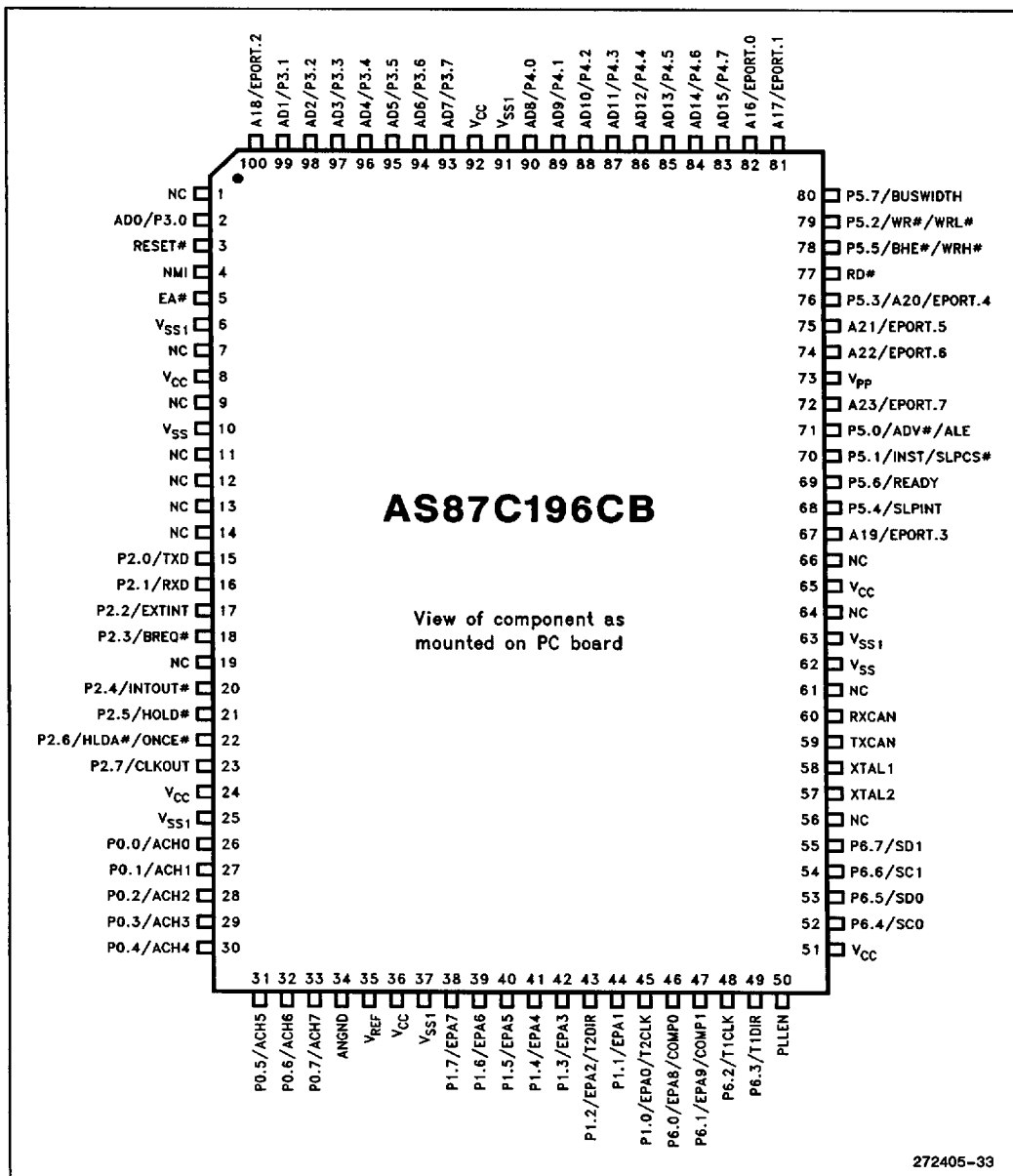
Figure 4. 100-Pin QFP AS87C196CB Diagram
