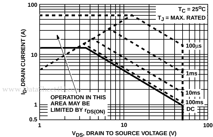
FIGURE 4. FORWARD BIAS SAFE OPERATING AREA
