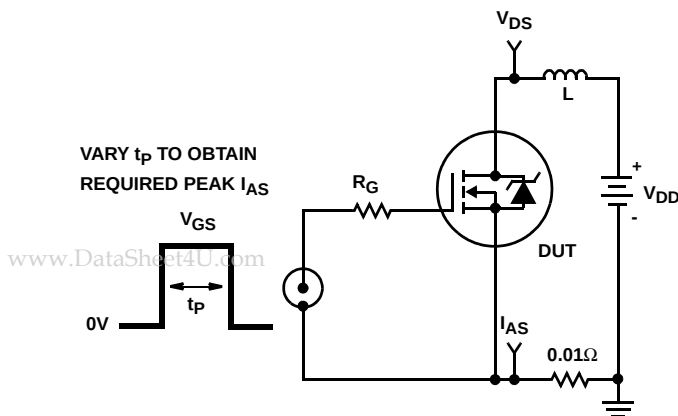
FIGURE 16. UNCLAMPED ENERGY TEST CIRCUIT
