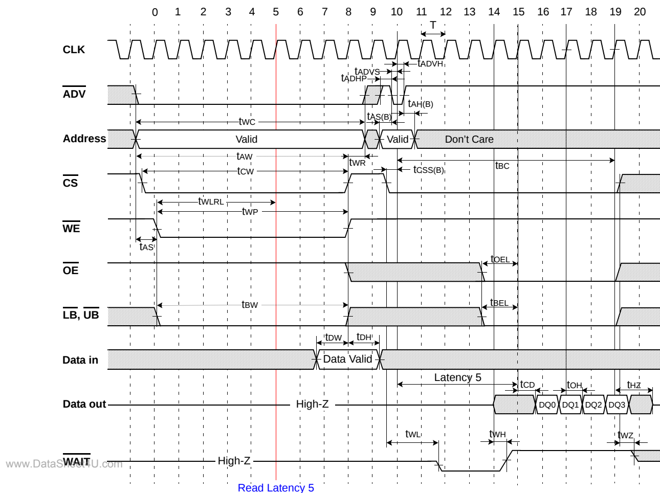
Fig.35 ASYNCH. WRITE(Low ADV Type) to SYNCH. BURST READ TIMING WAVEFORM [Latency=5, Burst Length=4]
