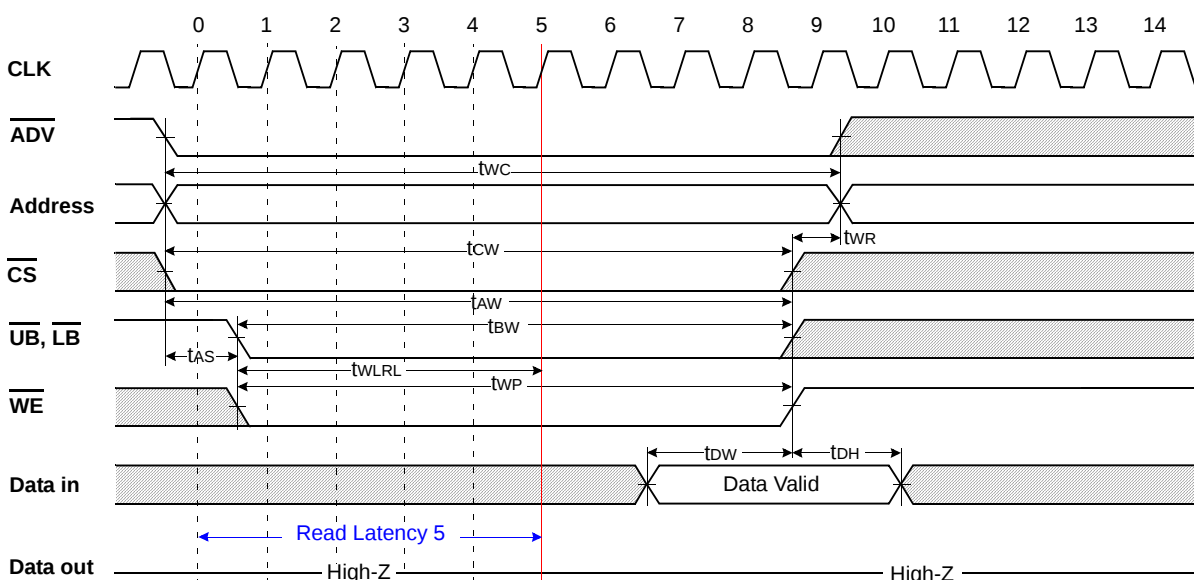
Fig.20 TIMING WAVEFORM OF WRITE CYCLE(Low ADV Type) ( \overline{OE}=V_{IH} , \overline{WAIT}=\text{High-Z} , \overline{UB} & \overline{LB} Controlled)
