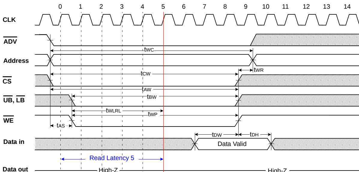
Fig.19 TIMING WAVEFORM OF WRITE CYCLE(Low ADV Type) ( \overline{OE}=V_{IH} , \overline{WAIT}=\text{High-Z} , \overline{WE} Controlled)
