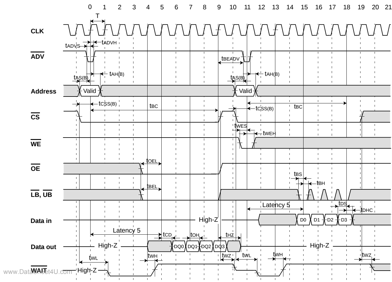
Fig.36 SYNCH. BURST READ to SYNCH. BURST WRITE TIMING WAVEFORM
