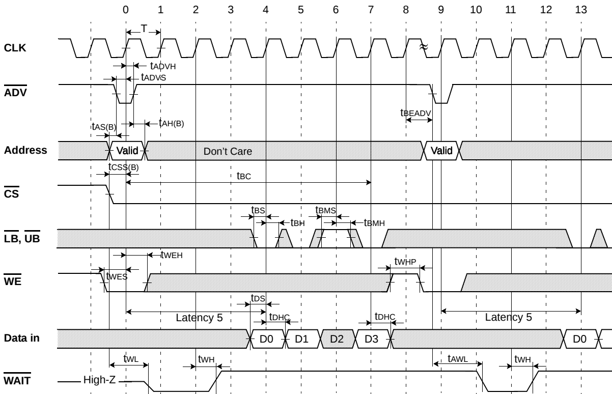
Fig.28 TIMING WAVEFORM OF BURST WRITE CYCLE(2) [Latency=5,Burst Length=4,WP=Low enable]( \overline{OE}=V_{IH} ) - \overline{CS} Low Holding Consecutive Burst Write
