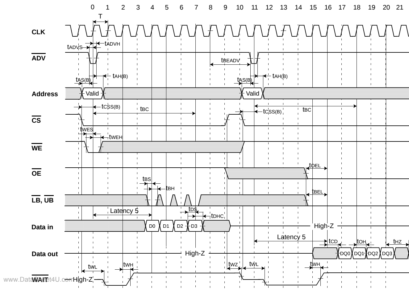
Fig.37 SYNCH. BURST WRITE to SYNCH. BURST READ TIMING WAVEFORM
