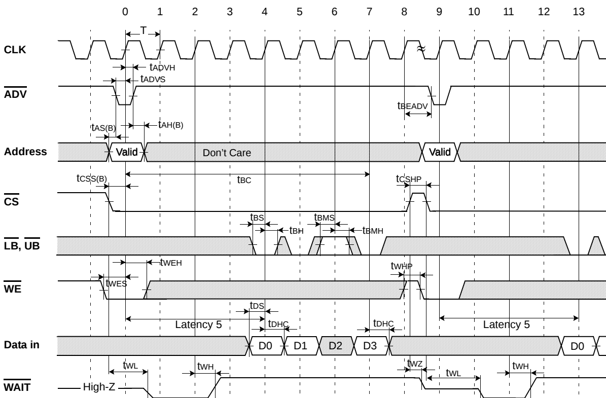
Fig.27 TIMING WAVEFORM OF BURST WRITE CYCLE(1) [Latency=5,Burst Length=4,WP=Low enable]( \overline{OE}=V_{IH} ) - CS Toggling Consecutive Burst Write
