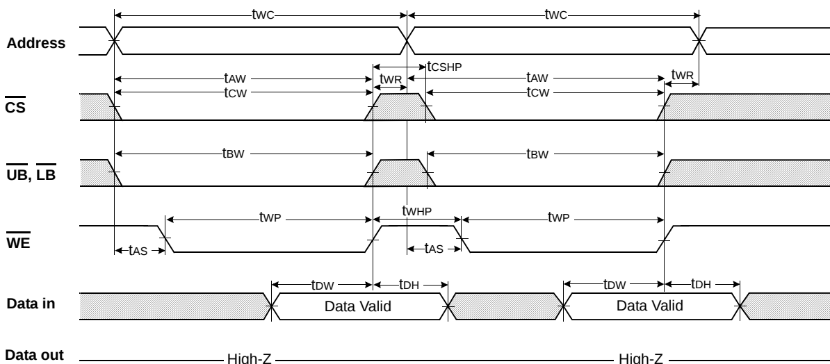
Fig.15 TIMING WAVEFORM OF WRITE CYCLE(1) ( \overline{OE}=V_{IH} , \overline{WAIT} =High-Z, \overline{WE} Controlled)
