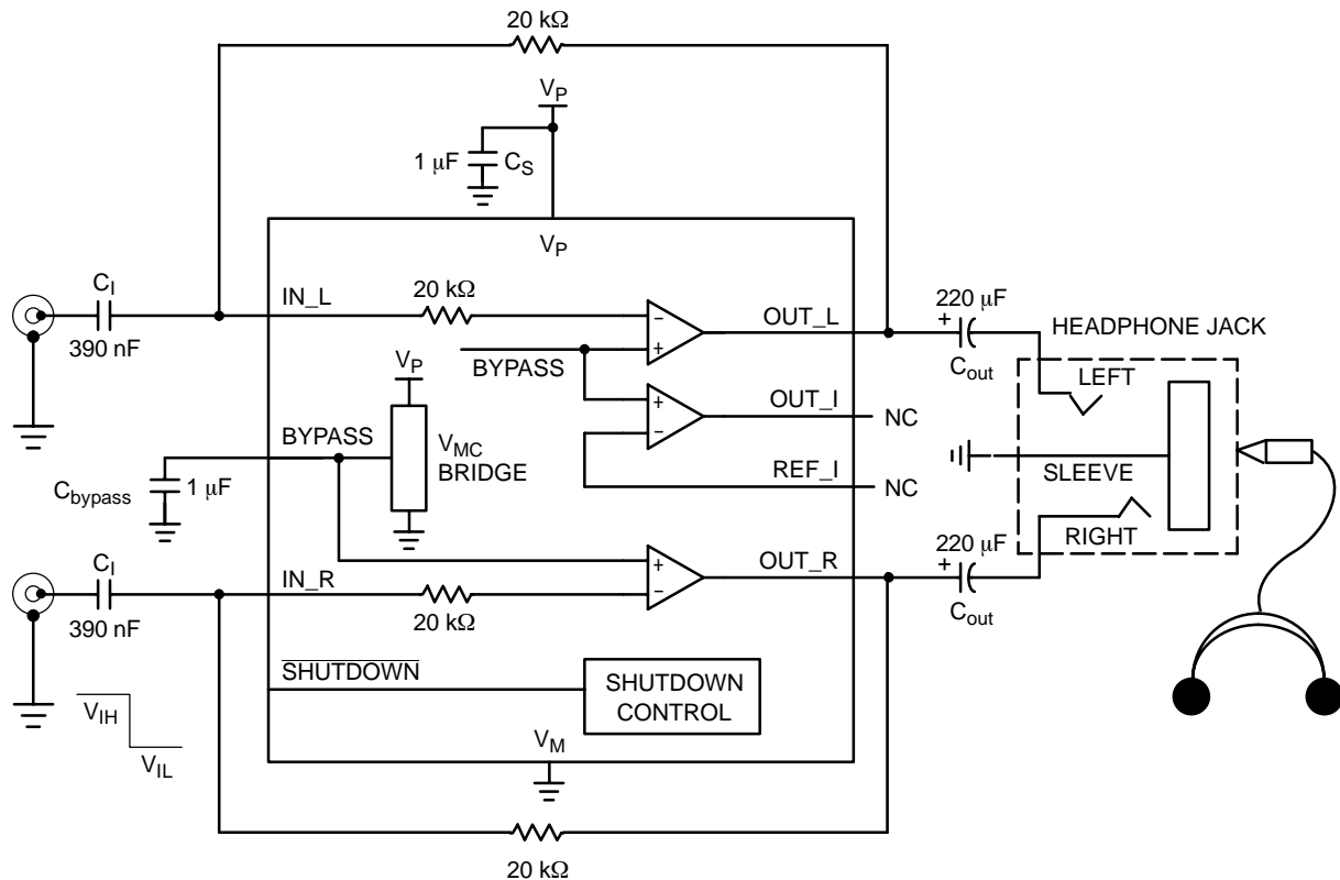
Figure 5. NCP2809B Typical Application Schematic with Output Coupling Capacitor
