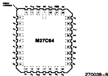
Figure 2. Pin Configurations
