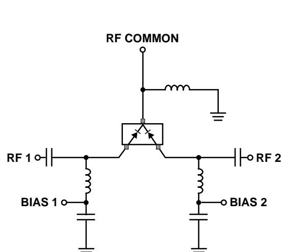
Figure 7. Simple SPDT Switch, Using Only Positive Current.
