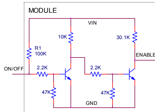
Figure 48. Remote On/Off Implementation. Resistor R1 is absent in the -49Z and -51Z option modules.
