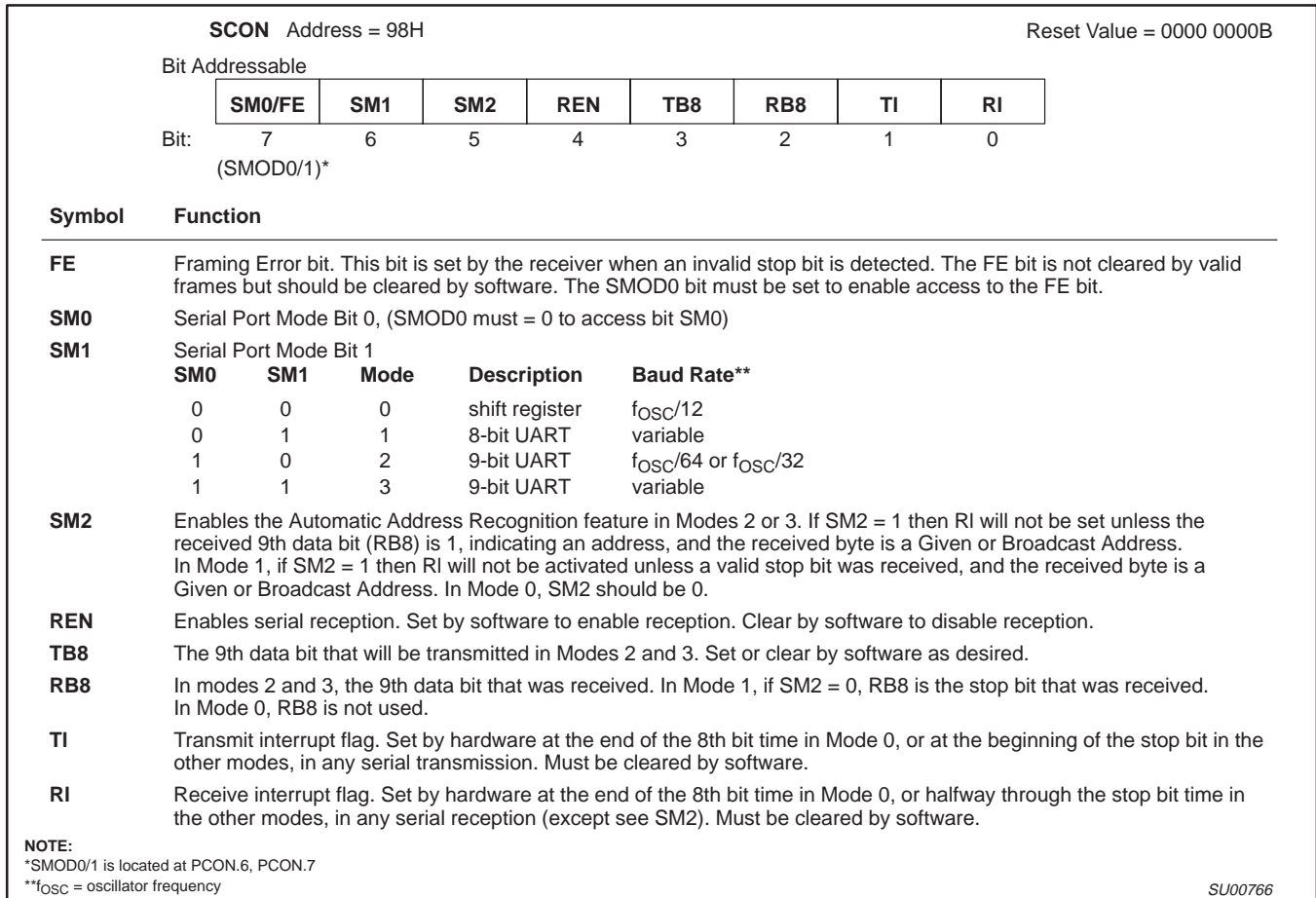
Figure 19. SCON: Serial Port Control Register
