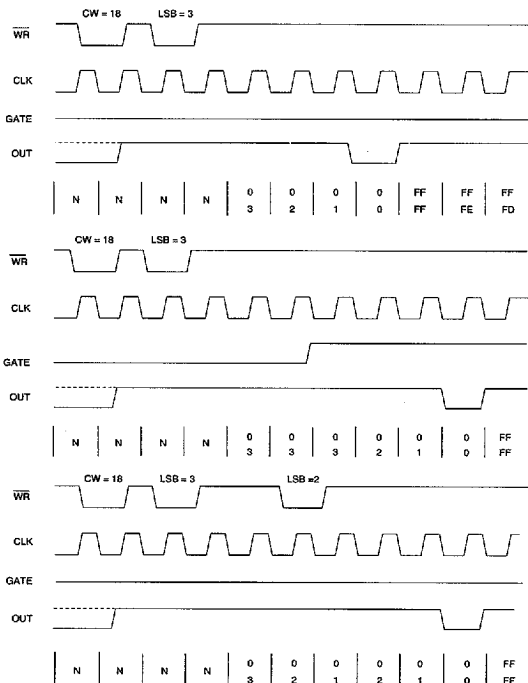
Figure 2-16: Mode 4 Timing
