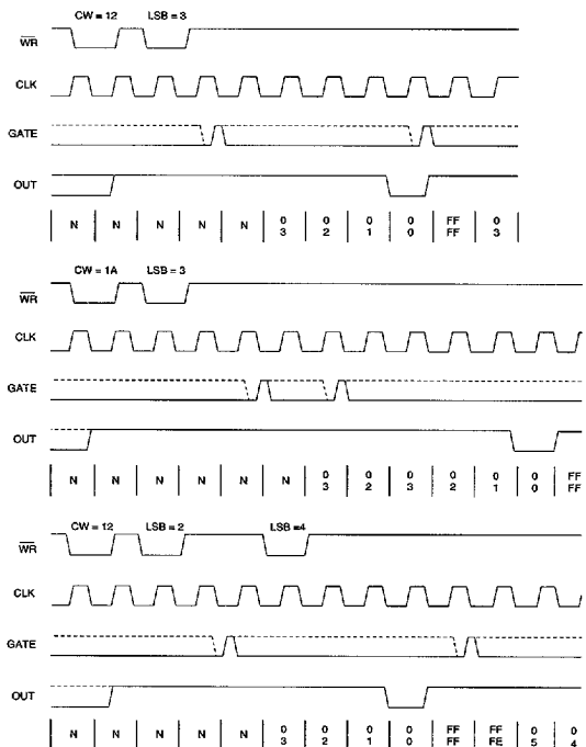
Figure 2-17: Mode 5 Timing
