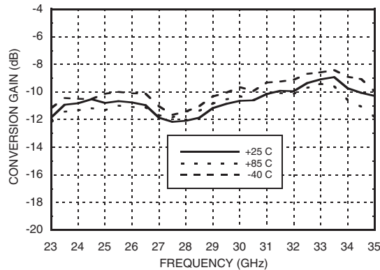
Conversion Gain vs. Temperature, LSB
