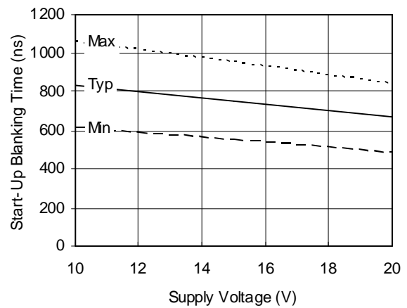
Figure 10B. Start-Up Blanking Time vs. Voltage
