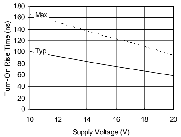
Figure 8B. Turn-On Rise Time vs. Voltage
