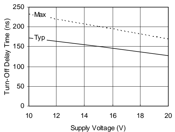
Figure 7B. Turn-Off Delay Time vs. Voltage
