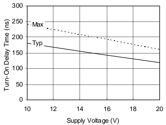
Figure 6B. Turn-On Delay Time vs. Voltage
