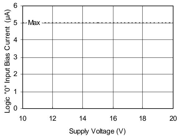
Figure 22B. Logic "0" Input Bias Current vs. Voltage
