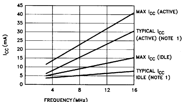
Figure 5. I_{CC} vs Frequency
