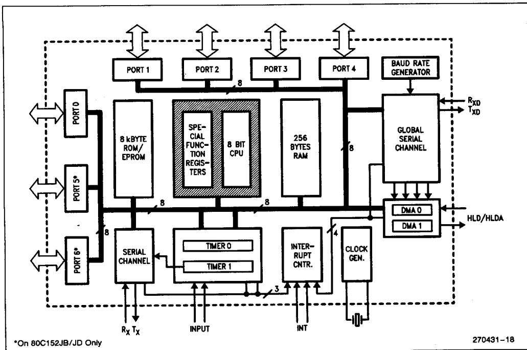
Figure 2. Block Diagram
