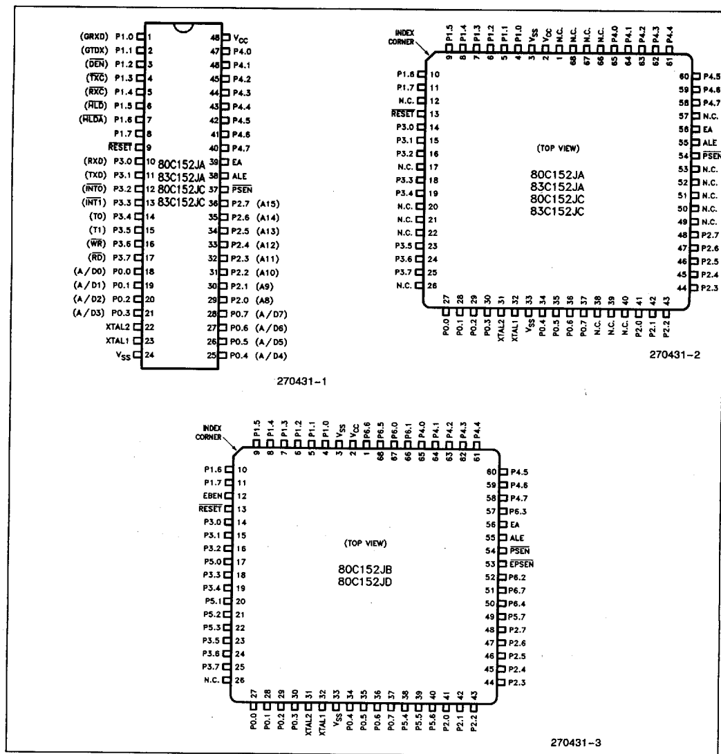
Figure 1. Connection Diagrams
