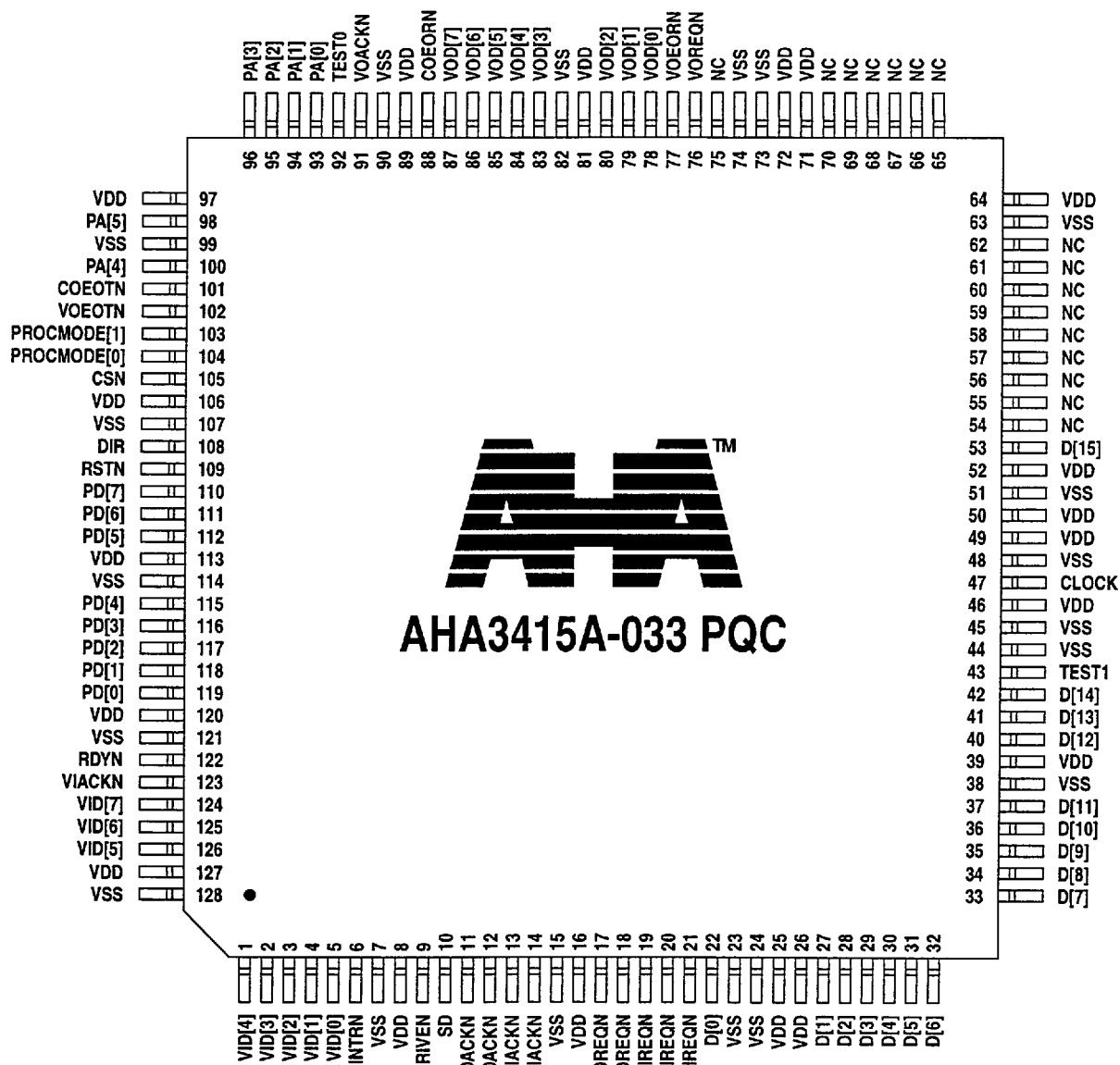
Figure 16: Pinout
