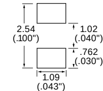
REFLOW SOLDER
