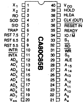
Figure 2 : PDIP PIN CONFIGURATIONS
