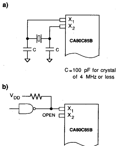
Figure 5 : EXTERNAL CLOCK CIRCUITS
