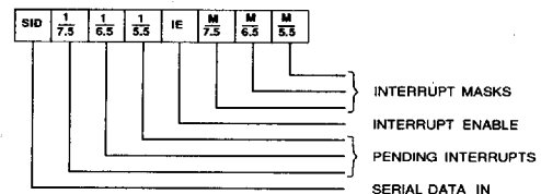
Figure 7 : RIM INSTRUCTION DATA BYTE
