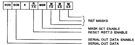
Figure 6 : SIM INSTRUCTION DATA BYTE
