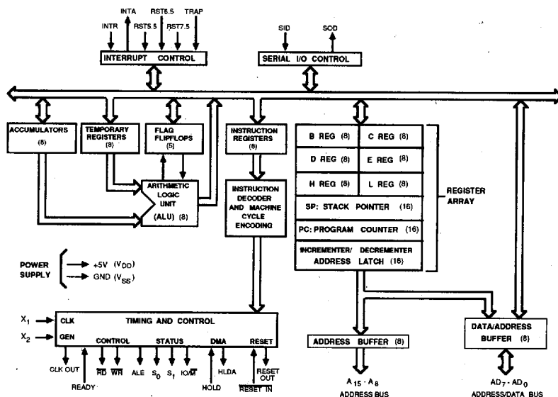
Figure 1 : CA80C85B BLOCK DIAGRAM
