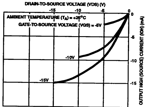
FIGURE 5. MINIMUM OUTPUT HIGH (SOURCE) CURRENT CHARACTERISTICS
