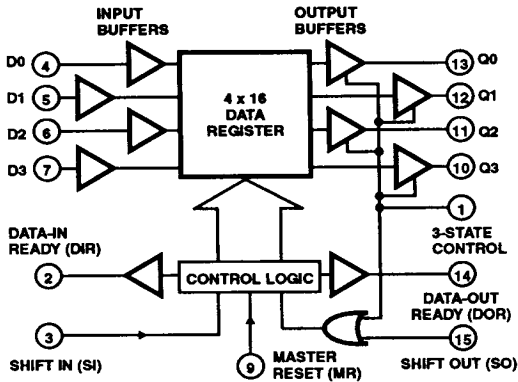
FIGURE 8. CD40105BMS FUNCTIONAL BLOCK DIAGRAM
