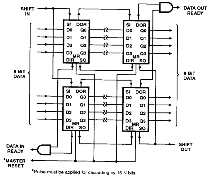
FIGURE 11. EXPANSION, 8-BITS-WIDE-BY-16 N-BITS LONG USING CD40105BMS
