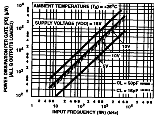
FIGURE 7. TYPICAL DYNAMIC POWER DISSIPATION AS A FUNCTION OF FREQUENCY
