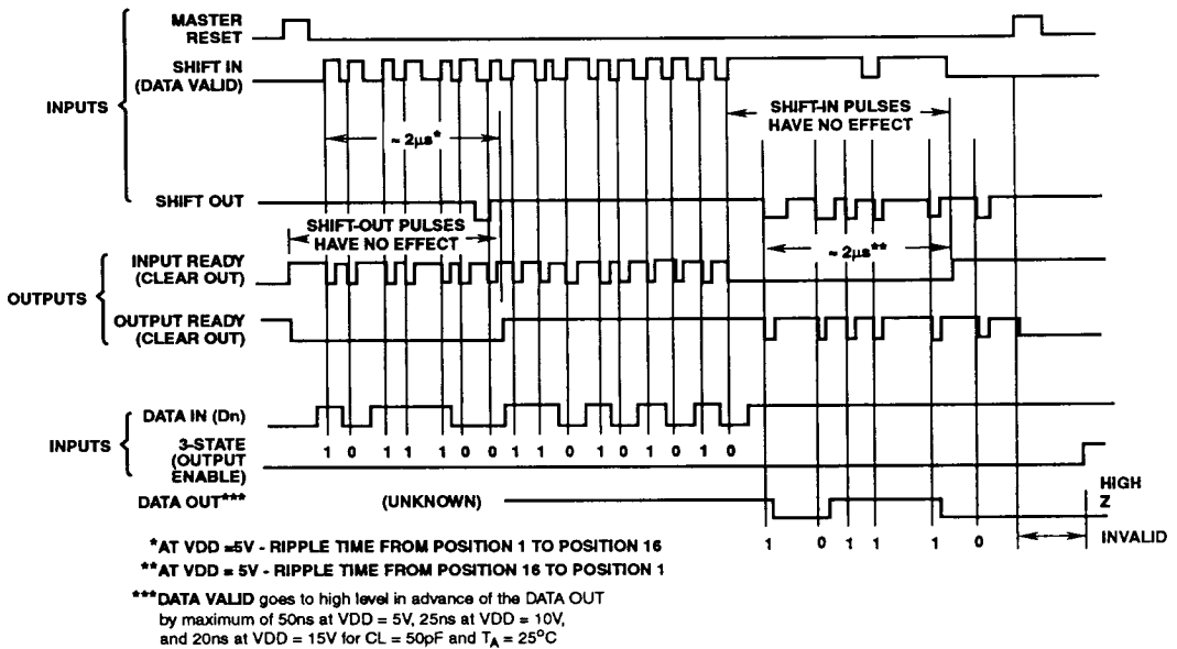
FIGURE 10. TIMING DIAGRAM FOR THE CD40105BMS
