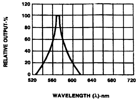
Fig.2 SPECTRAL RESPONSE
