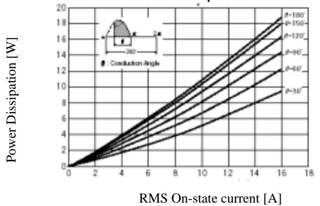
Fig 4. On State Current vs. Maximum Power Dissipation
