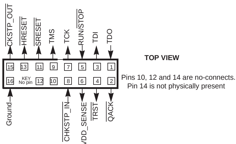
Figure 20. COP Connector Diagram
