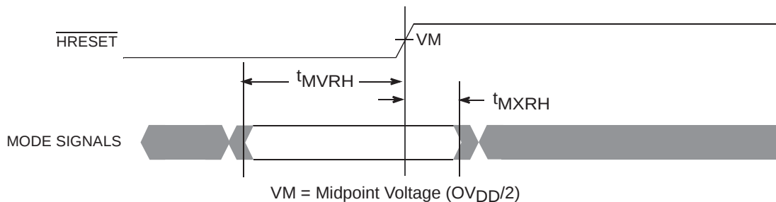
Figure 8. Mode Input Timing Diagram
