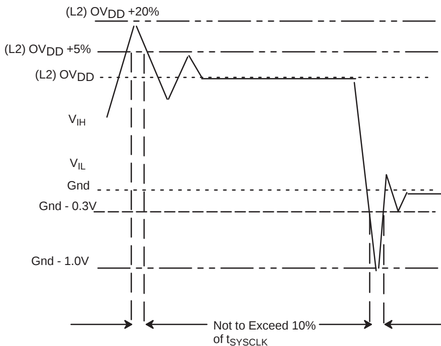
Figure 3. Overshoot/Undershoot Voltage
