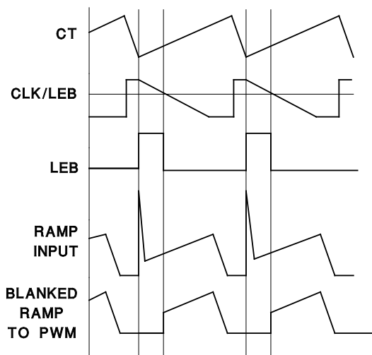
LEB Operational Waveforms
