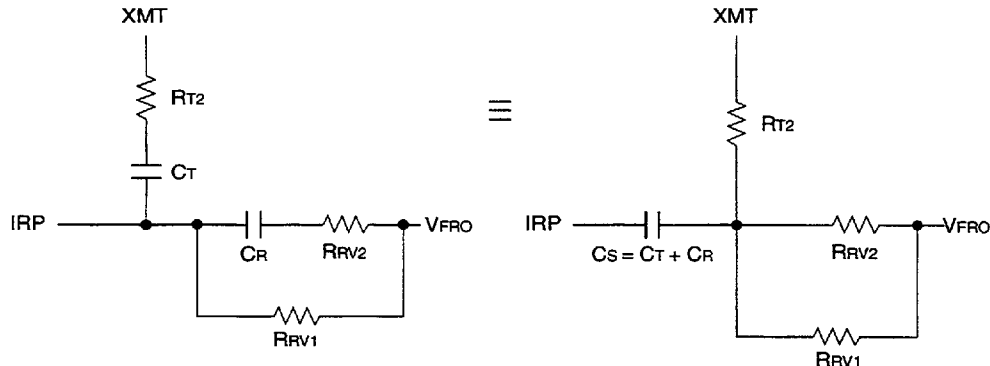
Figure 13. Revised ac Interface C_T and C_R Combined into a Single Capacitor C_s
