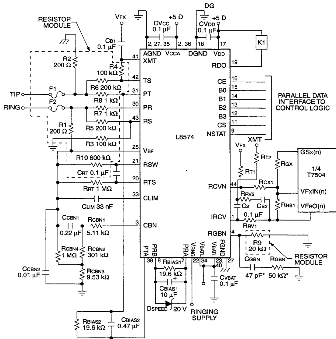
Figure 5. External Components Required
