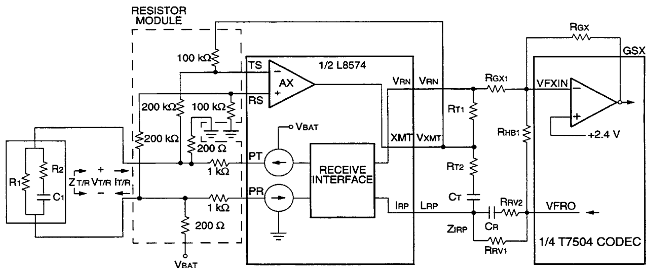
Figure 12. Initial ac Interface for Complex Termination Between L8574 SLIC and T7504 Codec Note: dc Blocking Capacitor (Cb) Not Shown, Ct and Cr Separate
