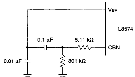
Figure 8. Implementing the Noise Cancellation Function
