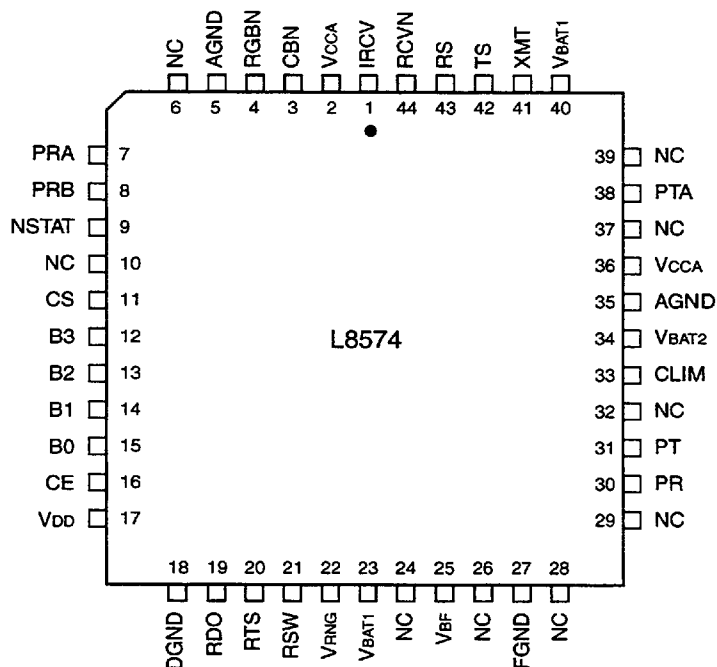
Figure 2. Pin Layout
