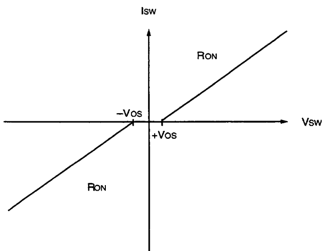
Figure 4. Switch On-State V-I Characteristics SW3
