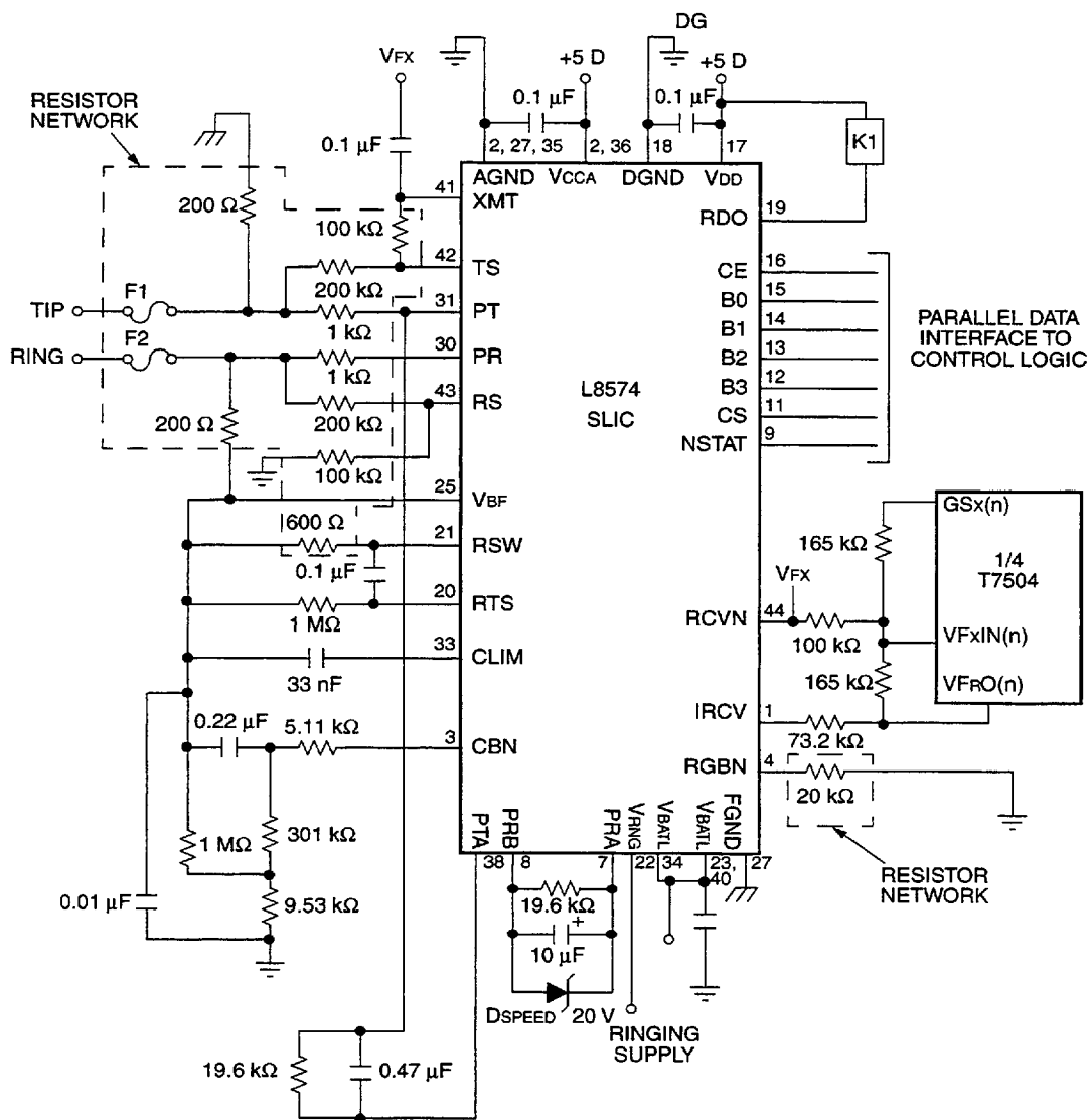
Figure 15. TR-57 Application Diagram
