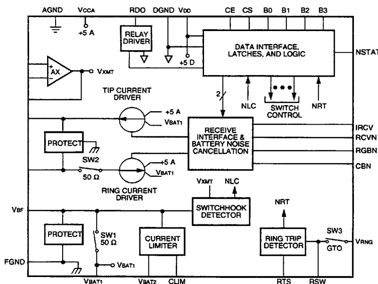
Figure 1. Architectural Diagram
