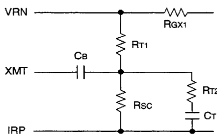
Figure 14. Addition of Resistor R_{SC} from XMT to IRP
