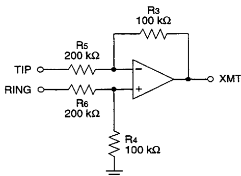
Figure 7. L8574 SLIC Matching Requirements
