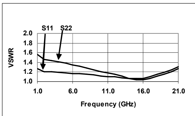
2 dB VSWR (S11, S22)
