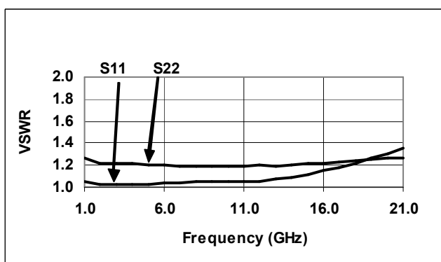
8 dB VSWR (S11, S22)
