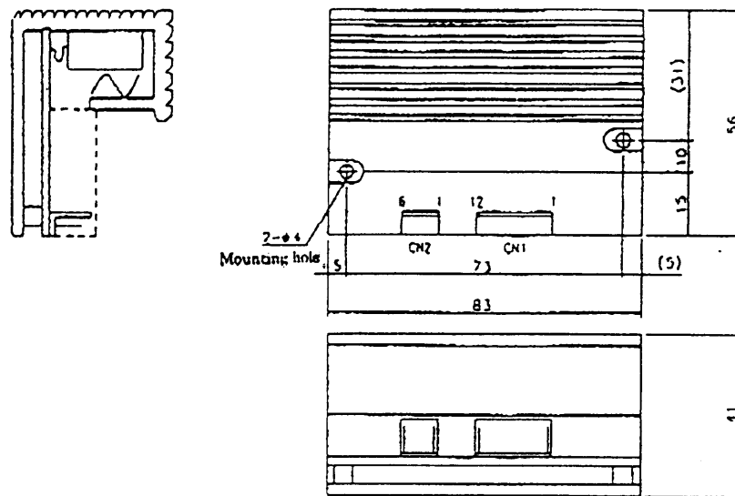
Figure 2. Overall Dimensions
