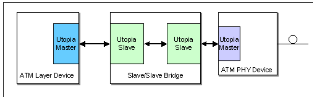
Figure 2: Utopia Slave Bridge
