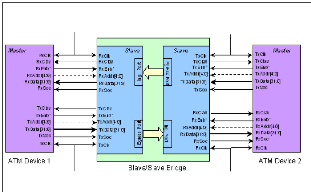
Figure 3: Slave/Slave Bridge connecting two Master Devices
