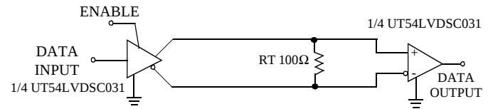
Figure 3. Point-to-Point Application
